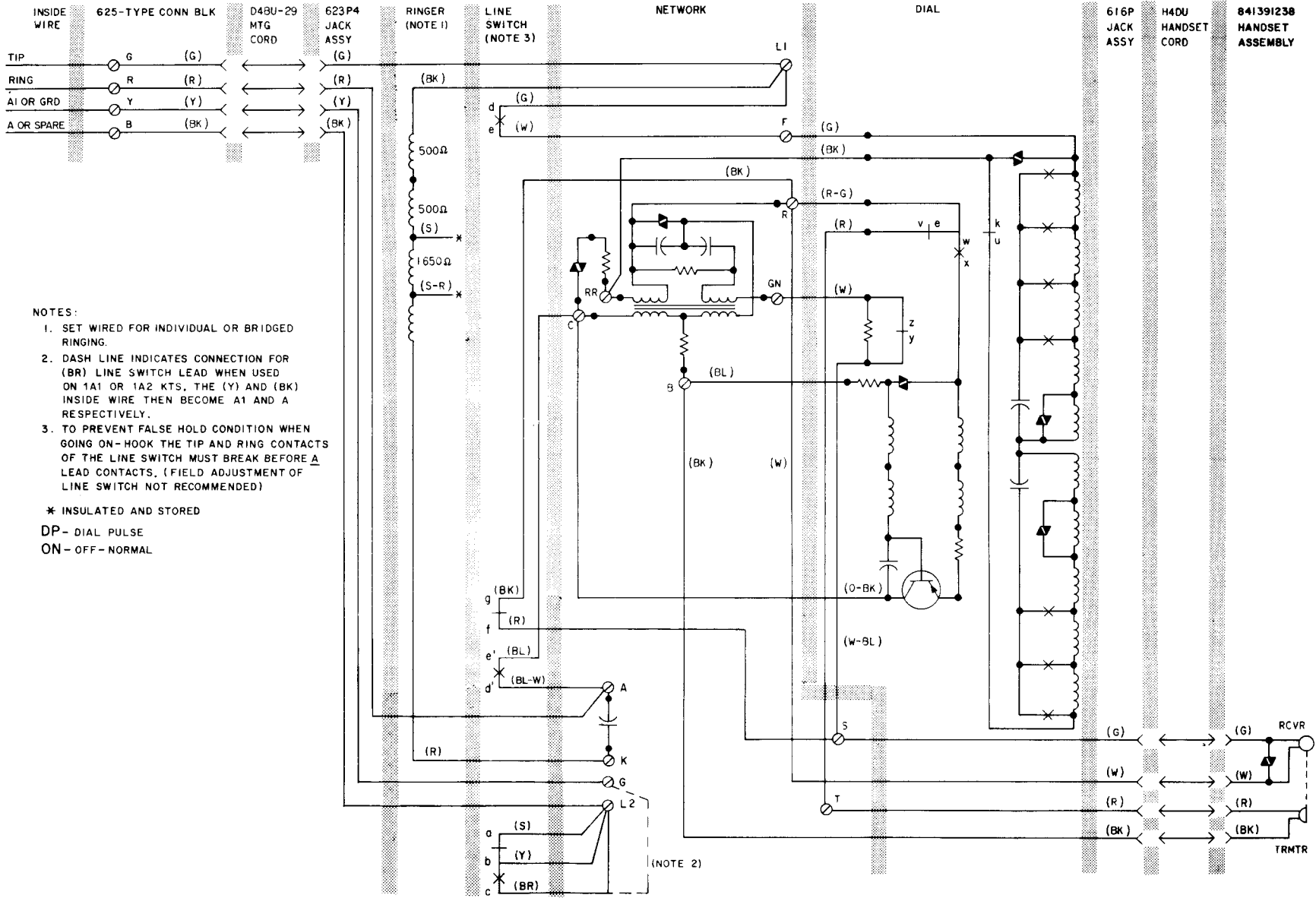
2881C109 Telephone Set, Connections
