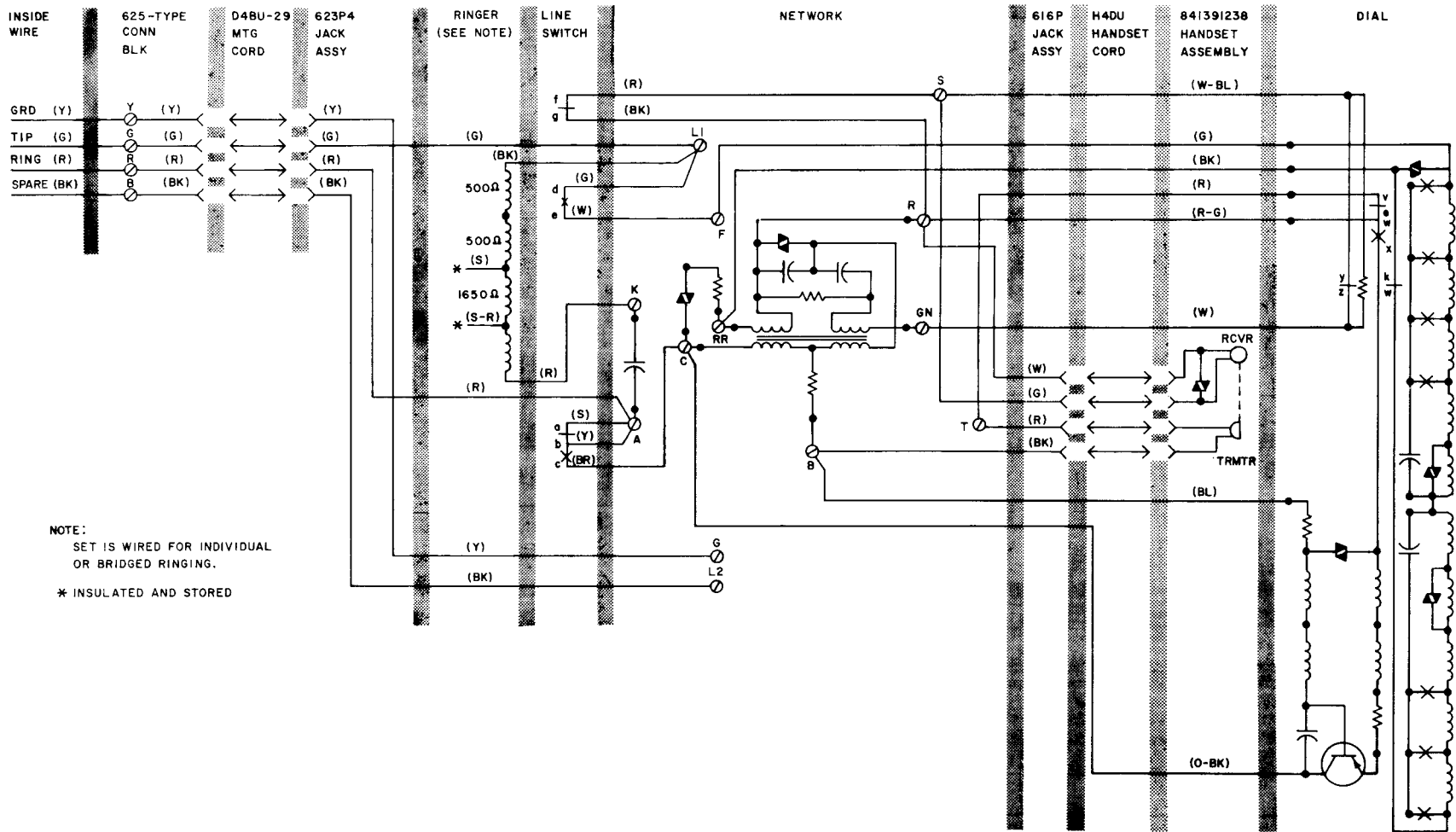
2881B109 (MD) Telephone Set, Connections
