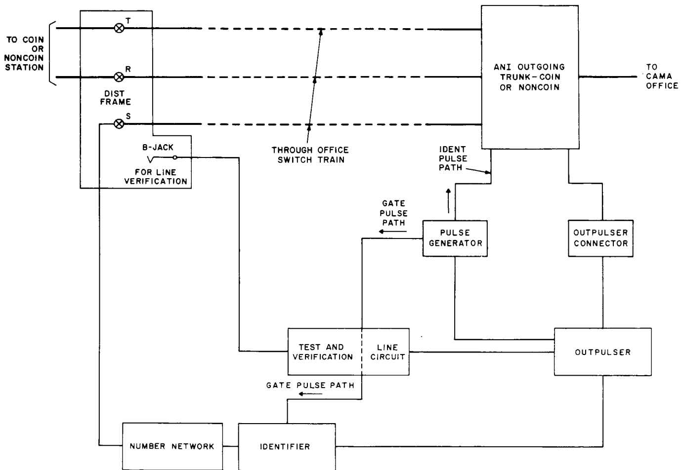
Fig. 1—Simplified System—Block Diagram ANI-C
