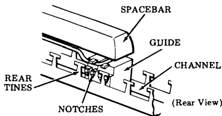
Fig. 2—Spacebar Removal
