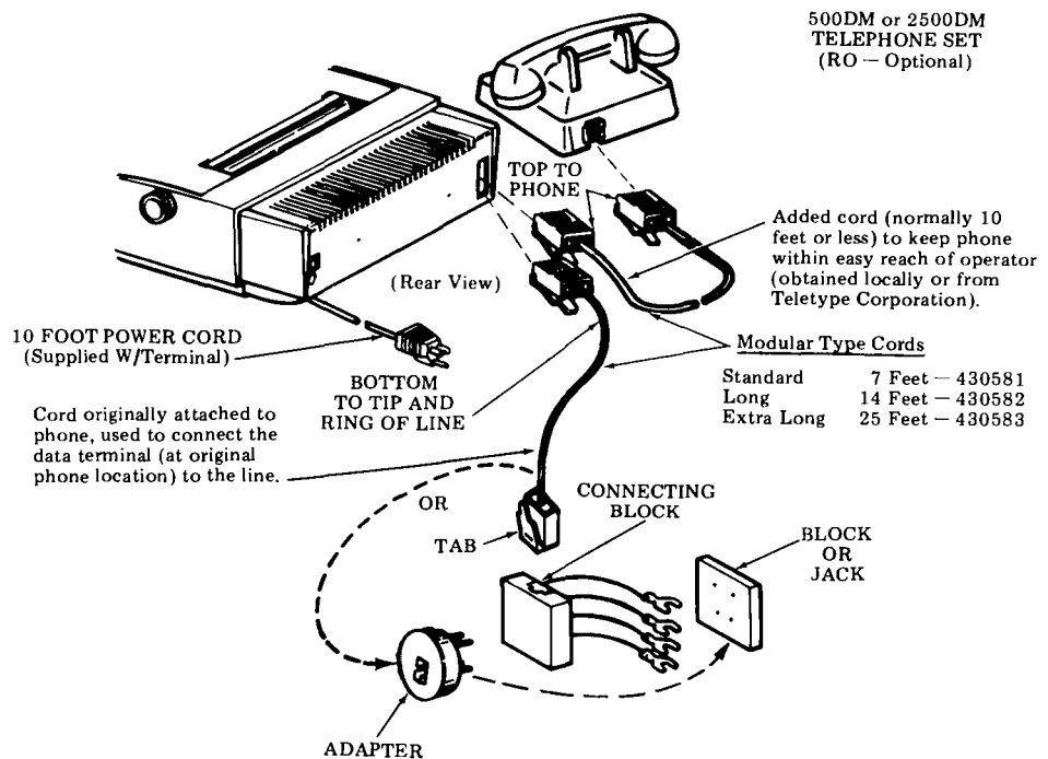
Fig. 4--Telephone Connection
