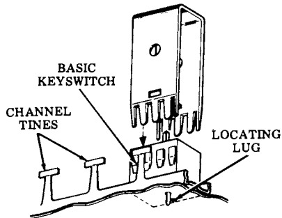
Fig. 10—Keyswitch Removal
