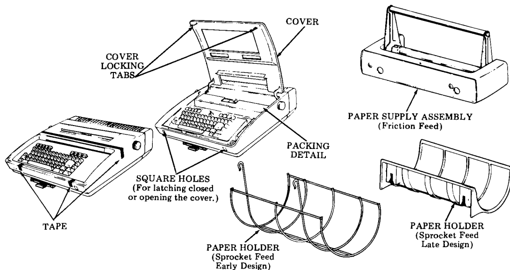
Fig. 2—Packing Detail
