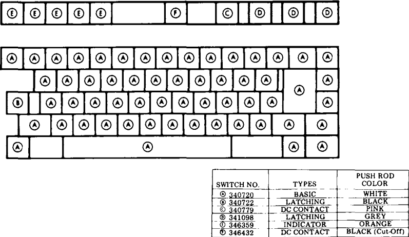
Fig. 22—Keyswitch Identification (KSR)
