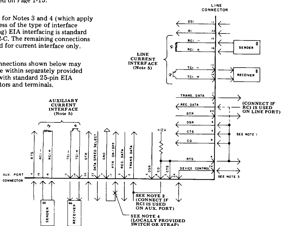
Fig. 8—Interface Connections
