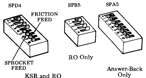
Fig. 2—Standard Switch Positions
