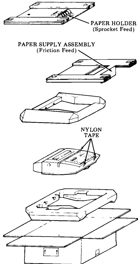
Fig. 12—Packing Details
