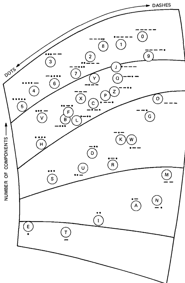
Fig. 11-6. Multidimensional scaling (MDS) map obtained by a computer analyzing data on confusability between Morse-code signals. The distance between any two signals on the map is monotonically and inversely related to the degree of confusion experienced by the listener (i.e., believing that two signals are the same). The confusability between two Morse-code signals appears to depend on the difference in the number of components (dots or dashes) in the two signals and on the relative proportions of dots and dashes. The curved lines, arbitrarily drawn to divide the map into regions where the signals have the same total number of components, facilitate the interpretation of the results. [Shepard, Human Factors 5 (1963): 39.]
