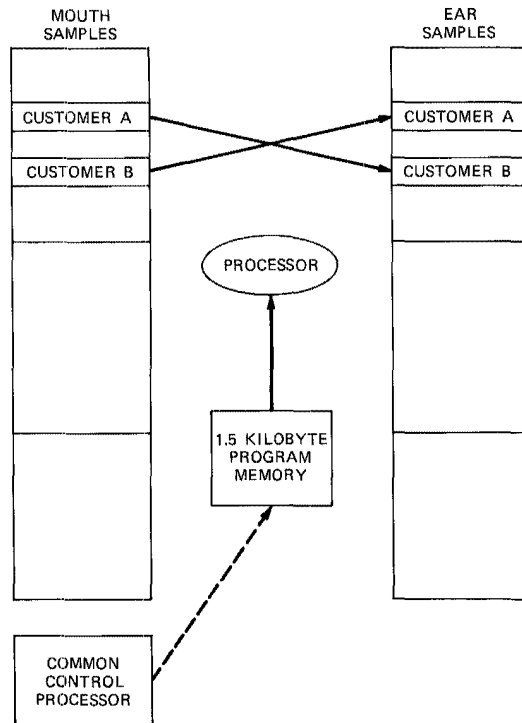
Fig. 8-15. Intelligent network processor. The fabric of the XDS network differed substantially from previous electronic switching systems. It performed the switching function by executing a series of computer instructions on a high-speed network processor instead of closing metal contacts or filling time slots.
