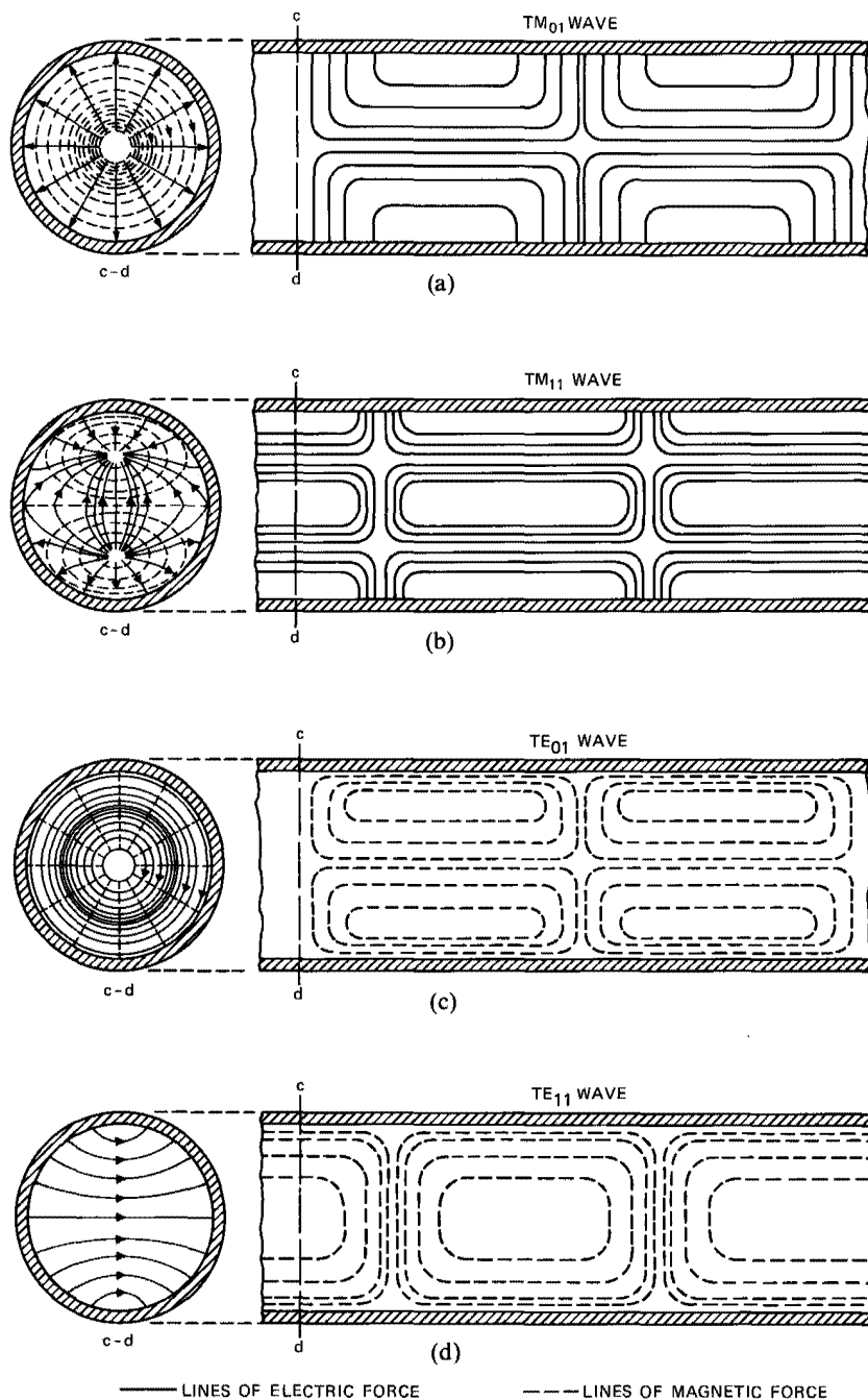
Fig. 6-3. Electric and magnetic fields in circular waveguide. [Southworth, Principles and Applications of Waveguide Transmission (1950): 120.]
