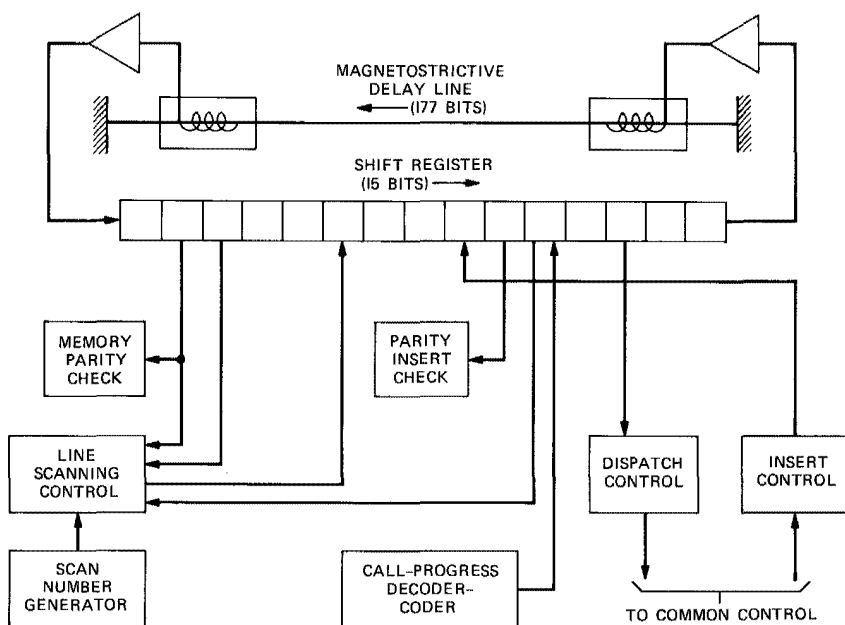
Fig. 8-13. Magnetostriuctive delay line. Memory units, such as the line-gate-number memory, in the ESSEX system were magnetostriuctive delay lines that held serial pulse trains of binary-coded words. Together with a 15-stage shift register, a recirculating loop operating at the clock rate of the system was formed for 24 words of 8 bits each. The information in the shift register could be examined and transmitted to external circuits in serial form as line gate numbers to the remote unit or in parallel form to the call-progress decoder-coder. Parity check circuits checked for data errors.
