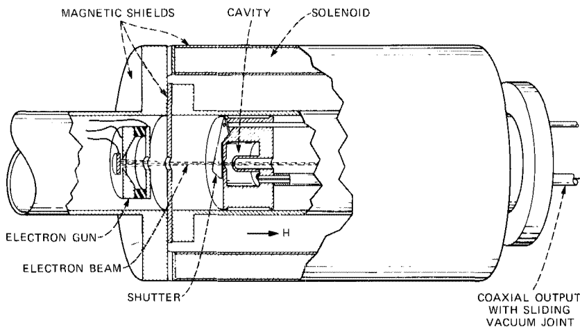
Fig. 4-10. The apparatus used by Cutler and Quate in measuring the noise current along an electron beam. The gun is at the left. The beam passes through a resonant cavity that can be slid along so that the noise current can be picked up and measured as a function of distance along the beam. [Cutler and Quate, Phys. Rev. 80 (1950): 875.]
