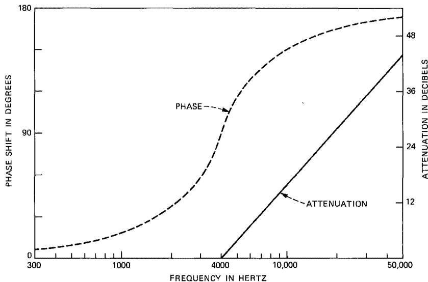
Fig. 1-21. Attenuation and phase-shift characteristics for a low-pass network filter, as derived from H. W. Bode's gain-phase integral, expressing the minimum phase function in terms of the given attenuation function. The example shown is for a filter having zero attenuation below 4000 Hz and an attenuation that increases at 12 dB per octave above 4000 Hz. Understanding the connection between attenuation and phase was a crucial help to designers of stable feedback amplifiers. [Bode, Network Analysis and Feedback Amplifier Design (1945): 316.]
