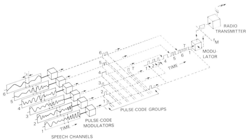
Fig. 10-6. Schematic of a time-multiplexed transmission system for six speech channels. This is taken from a 1948 description of C. B. Feldman's experimental 96-channel system.
