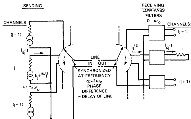
Fig. 10-3. W. R. Bennett's 1941 representation of a time-division multiplex system. Samples from three channels at left are delivered to three receiving channels at right.
