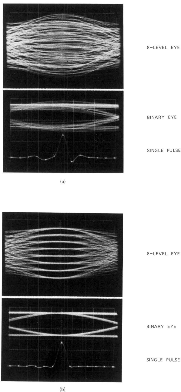
Fig. 10-14. Oscilloscope sweeps of received data voltage for a horizontal sweep rate of 1/T , where T is the sampling period. The display is known as an eye pattern for binary data. (a) Before equalization, and (b) after equalization with R. W. Lucky's automatic equalizer.
