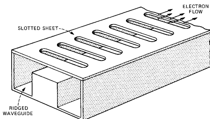
Fig. 4-9. Karp's space-harmonic circuit for traveling wave amplifiers and backward-wave oscillators of millimeter waves. [Karp, Proc. IRE 45 (1957): 496.]
