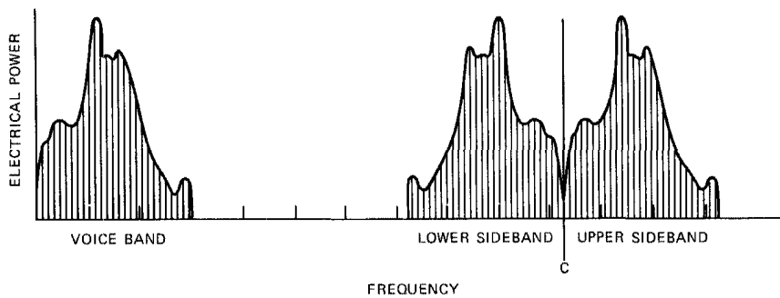
Fig. 1-2. When the voiceband of frequencies (left) is used to amplitude-modulate a carrier frequency (C), the double sideband frequency spectrum shown (right) is produced, since each sinusoidal speech component frequency, f_n , generates two additional components in the transmitted signal, C - f_n and C + f_n .
