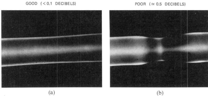
Fig. 7-7. Fusion splice of silica optical fibers, as obtained in 1975 by D. L. Bisbee, with an electric arc, a technique that has found worldwide commercial use. The photographs show (a) A good splice, with a loss of less than 0.1 dB. [Bisbee, Appl. Opt. 15 (1976): 797.] (b) A poor splice, with a loss over 0.5 dB. The latter was obtained when the fiber ends were not in intimate contact over the entire surface.
