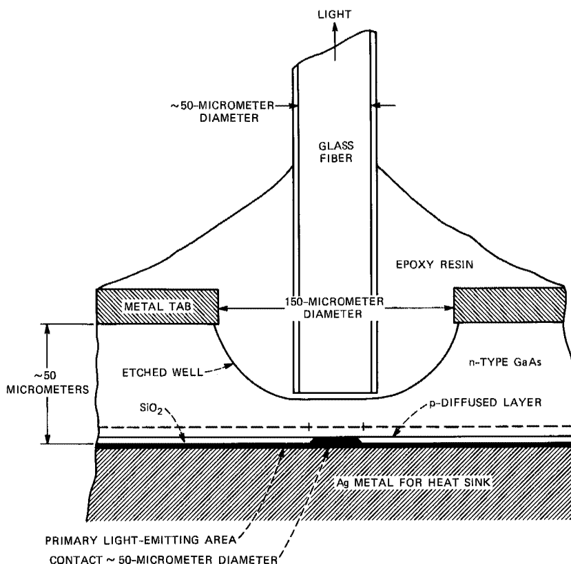
Fig. 7-3. Early version of the first LED designed by C. A. Burrus (about 1969) for use with optical fibers. Light emission was from a small region, defined by the electrical contact, which was approximately equal to the area of a fiber core. Later versions were more complicated double-heterostructure designs with several grown layers replacing the simple p-n junction. [Burrus and Dawson, Appl. Phys. Lett. 17 (1970): 97.]
