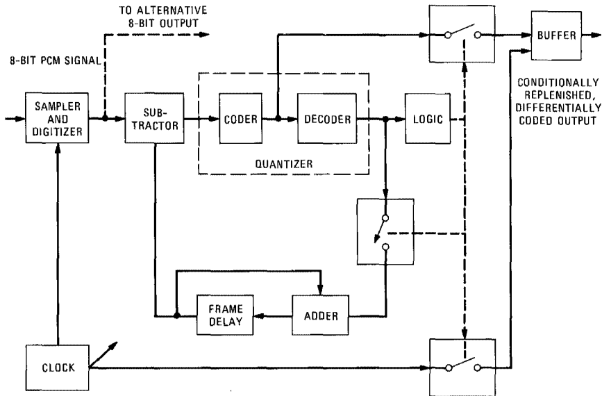
Fig. 3-9. Basic functions of a conditional replenishment television coder. The delay in the frame memory loop must equal the frame period. When there is no interframe change, the stored signal simply recirculates, and nothing is given to the buffer for transmission. When a significant difference is detected, the new signal is stored and transmitted along with a code that indicates position in a scan line. The decision threshold is adjusted to prevent buffer overflow or underflow.
