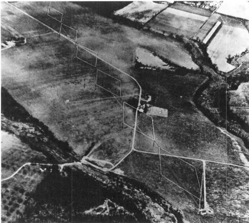
Fig. 5-7. The six-element Multiple Unit Steerable Antenna (MUSA). This first electronically steerable antenna had good vertical-plane directivity and could be electronically steered with phase shifters for angular directivity, resulting in improved reception, signal-to-noise ratio, and audio quality.
