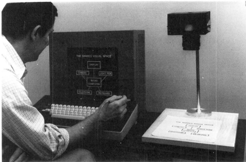
Fig. 3-13. Experimental graphic display system. A plasma panel was used for viewing a picture common to both terminals of a communication system. Pictures can be entered and annotated from either terminal with the aid of a microprocessor or from a digital memory. [Sosnowski and Brainard, Proc. SID 20/3 (1979): 132.]
