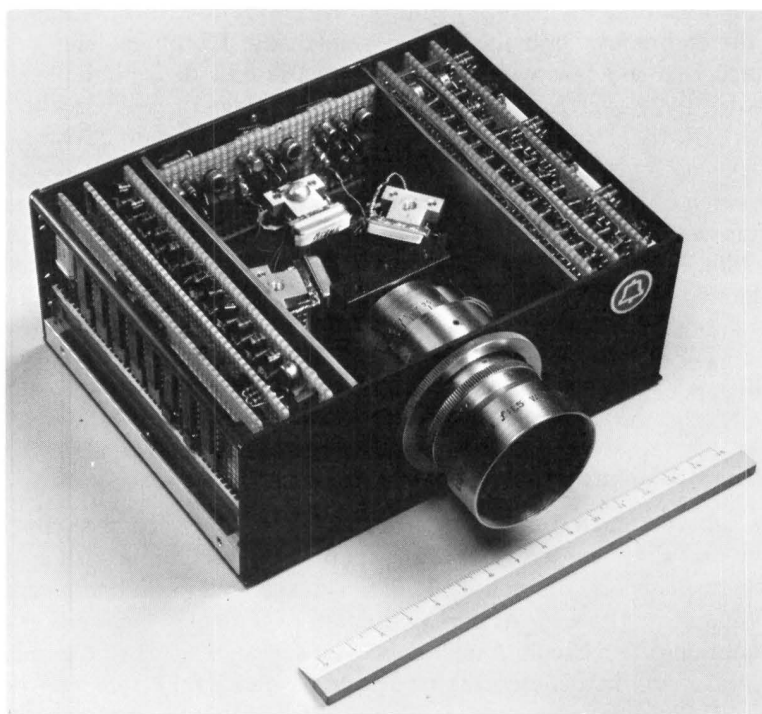
Fig. 3-11. The first solid-state color television camera. Light from a scene being viewed was split into three colors (red, green, and blue) and focused onto three separate silicon CCD image sensors. The light was converted by the sensors into electrical charge, stored and sequentially read out of each device as video signals corresponding to each color image. The signals were applied to a color television monitor to recreate the image of the scene.
