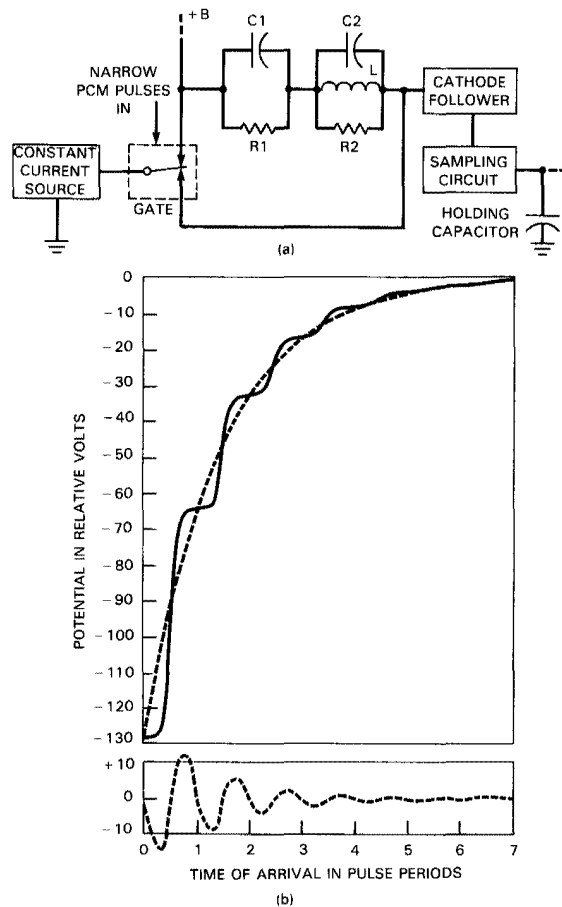
Fig. 10-8. Principles of Shannon-Rack decoder. (a) The decoder uses two capacitor discharging circuits in series. In the left-hand circuit, a capacitor is shunted by a resistor and discharges exponentially. In the right-hand circuit, the capacitor is shunted by a resistor and a resonating inductor; it discharges as an exponential sinusoid. (b) Curves in dashed lines represent the discharge of the left and right circuits of (a); their combination is shown by the solid-line curve.
