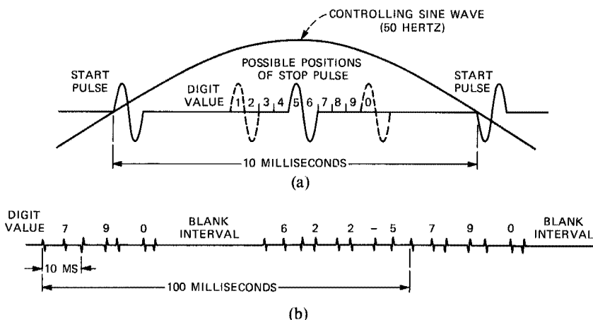
Fig. 8-3. ECASS pulse-position dialing. (a) Called-number signals at about 50 times the speed of conventionally dialed digits were sent from the ECASS telephone under control of 50-hertz simplex power sent from the central office. These signals, called pulse-position dialing, consisted of two pulses per digit: a start pulse at each zero-crossing of the 50-hertz control wave and some time later in the 10 millisecond half-cycle interval, a stop pulse. Each digit pulse was approximately a single cycle of a 1000-hertz sine wave and the interval between a start pulse and its following stop pulse was identified with an associated digit value. The digit pulses in consecutive intervals were of opposite polarity. (b) Compressed time scale. An interval of at least 3.2 milliseconds was provided after each pulse for possible transient lengthening in the transmission medium. A silent interval of two digits was provided between the automatic repetition of the entire dialed number.
