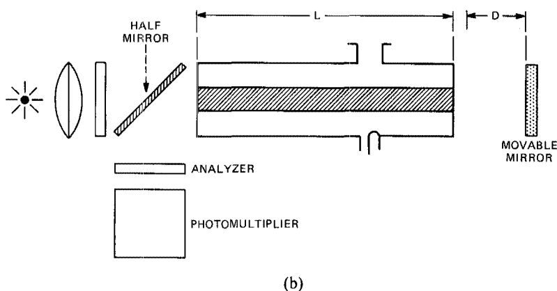
Fig. 7-9. Microwave light modulator. (a) Traveling wave light modulator used the electro-optic crystal KDP ( \text{KH}_2\text{PO}_4 ) and operated at 9.25 GHz. The refractive index in the crystal changes in proportion to an applied electric field. Thus, the microwave in the cavity, in synchronism with the optical wave, modulates the optical-phase retardation. The polarizer and analyzer convert the modulated retardation into intensity-modulated light. (b) Since no continuous-wave laser was readily available in 1961, a white-light source was employed and, since no high-speed optical detector was available, a movable mirror scheme (that showed a periodic behavior with mirror displacements equal to the microwave half-wavelength) was used. [Kaminow, Phys. Rev. Lett. 6 (1961): 528.]
