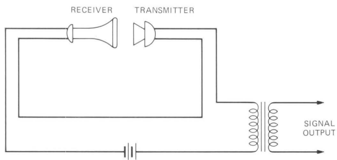
Fig. 1-13. A laboratory signal generator used in early telephony. This electromechanical feedback arrangement produces telephone howl or hum because the transmitter amplifies. [Adapted from Wright and Puchstein, Telephone Communication (1925): 402.]
