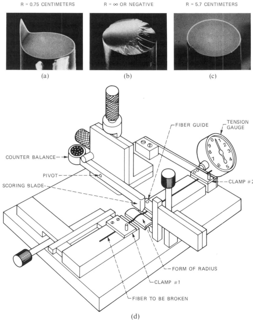
Fig. 7-8. Glass fiber ends. Glass fibers fracture in such a way that the ends resemble one of the three types shown in the top figure. To avoid the undesirable surfaces shown in (a) and (b) and consistently achieve the "mirror" surface (c), D. C. Gloge and coworkers proposed to bend the fiber over a form of suitable curvature radius R while simultaneously applying tension. If the radius is much larger than 5.7 cm, a "hackle" zone (b) forms; too small a radius causes the lip formation (a). To obtain reproducible fractures, they constructed the machine shown in the bottom figure (d).
