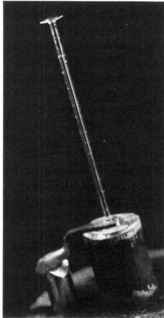
Fig. 7-2. Experimental LED-pumped Nd:YAG single-crystal fiber laser. The laser is composed of an Nd:YAG fiber grown at 75\text{-}\mu\text{m} diameter with heat from a \text{CO}_2 laser, a glass support tube, a 150\text{-}\mu\text{m} square output mirror, which is visible at the end of the fiber, and a similar input mirror in the well of the Burrus-LED pump. The LED operated near the 0.8\text{-}\mu\text{m} wavelength, and the 1.03\text{-}\mu\text{m} output of the laser was about a 1-milliwatt continuous wave. [Stone and Burrus, Fiber Integrated Opt. 2 (1979): 36.]
