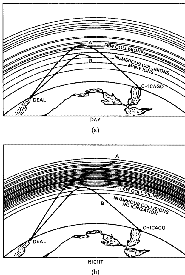
Fig. 5-2. Anomalous atmospheric propagation of shortwave radio. A is a higher-frequency radio wave (about 12 MHz). B is a lower-frequency radio wave (about 3 MHz). (a) With many ions in the atmosphere during the day, A is refracted to reach Chicago; B is just attenuated and does not reach its goal. (b) At night, however, the ions have disappeared. A is not refracted much, and B is much less attenuated.
