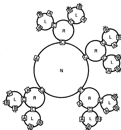
Fig. 10-18. The loop transmission hierarchy proposed by J. R. Pierce in 1972 for data transmission of blocks of data. L, R, and N represent local, regional, and national loops. Three types of boxes appear in the loops. In general, A times and closes the loop; B puts blocks of data on and takes blocks of data off the loop; C transfers blocks of data from one loop to another.
