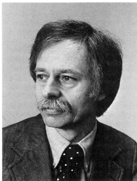
Fig. 11-4. R. N. Shepard, who pioneered in developing computer methods for constructing multidimensional "maps" of mental concepts from judged proximities among them.
