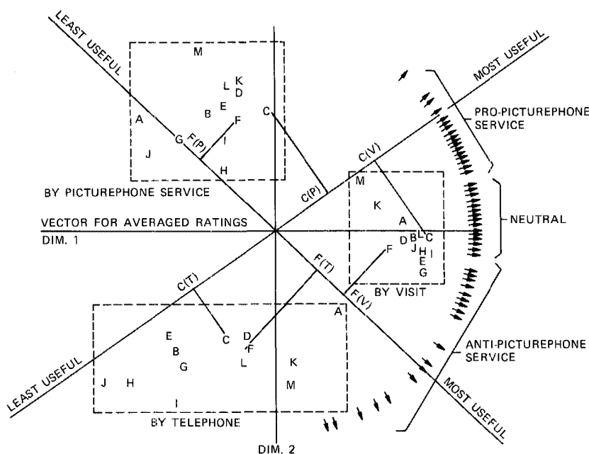
Fig. 11-12. Multidimensional preference analysis (MDPREF) based on ratings of usefulness of three different communication conditions—telephone (T), face-to-face visit (V), and PICTUREPHONE service (P) for the 13 different business tasks listed in Fig. 11-11. Each letter (A through M) refers to a different task; each task is represented three times, one for each communication condition. An arrowhead indicates the end of a vector through the origin that reflects a respondent's rating. A letter representing a task that received a high usefulness rating by someone projects highly on that person's vector. Positions of arrowheads and letters were determined directly by the MDPREF computer program. The rectangles around each of the services are inserted as an aid in interpreting the data. Generally, a visit was judged to be more useful for every business situation—i.e., all letters for visit project highest on most of the vectors. An interesting feature of this map is that two dimensions are required to account for all of the respondents' ratings. The second dimension separates PICTUREPHONE visual telephone service from the telephone.
