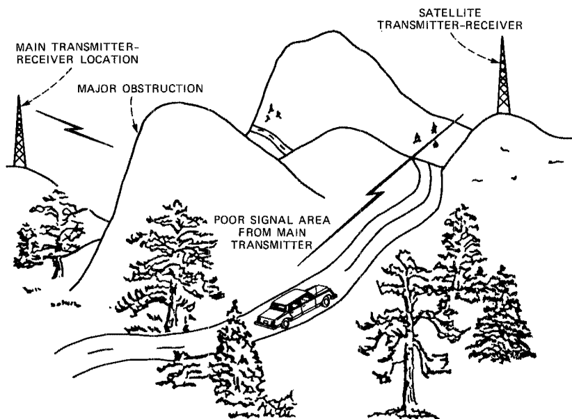
Fig. 5-15. Use of a satellite base station to fill an area of poor reception. [Jakes et al, Microwave Mobile Communications (1974): 378.]
