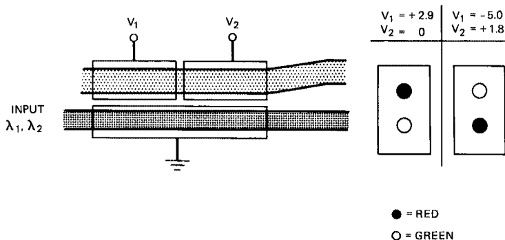
Fig. 7-13. Schematic drawing of the tunable, wavelength-selective directional coupler switch made with Ti:LiNbO 3 waveguides. Experimental results are shown for light of two colors (red and green) incident in the lower waveguide. Upon application of appropriate voltages to electrodes over the waveguides, the coupler is phase matched at the red wavelength, which crosses to and exits from the upper waveguide. The coupler is mismatched at the shorter wavelength and, as a result, the green light exits from the lower waveguide. By changing the applied voltages, the situation is reversed as shown. Crosstalk in both cases is -17 dB. The split electrode is required to achieve complete crossover at the phase-matched wavelength.
