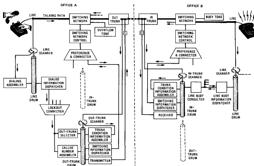
Fig. 8-8. Block diagram showing DIAD operation. In a DIAD system, the customer picked up the handset of the telephone and after hearing the dial tone dialed the number of the telephone he/she wished to reach. The digits were assembled on a magnetic drum that served lines in an area parallel to the axis of the drum and permanently assigned to the specific line. After collection, the dialed number was transferred to the outgoing trunk drum that sent orders to the switching network to set up a conversational path to a trunk to the called office. The called-line-number information was passed over the trunk to the in-trunk drum in the called office, which completed the connection to the called line.
