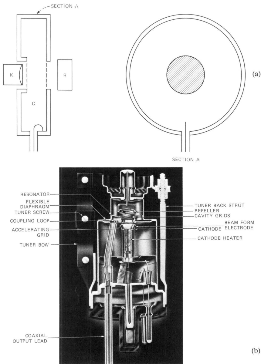
Fig. 4-2. The reflex klystron. (a) Schematic cross section of a reflex oscillator. Above left: C is the cavity, K is the hot cathode, and R is the repeller. Above right: a cross section of the cavity. (b) The reflex klystron (bottom). Many versions of this tube were built for use as beating oscillators for wartime radar. Output was about 100 milliwatts. The tube was tuned over a small range by bending the envelope structure so that the cavity dimensions were changed. The electron focusing was such that the electrons transversed the cavity just twice, avoiding hysteresis effects that took place in early tubes where reflected electrons reentered the cathode region.
