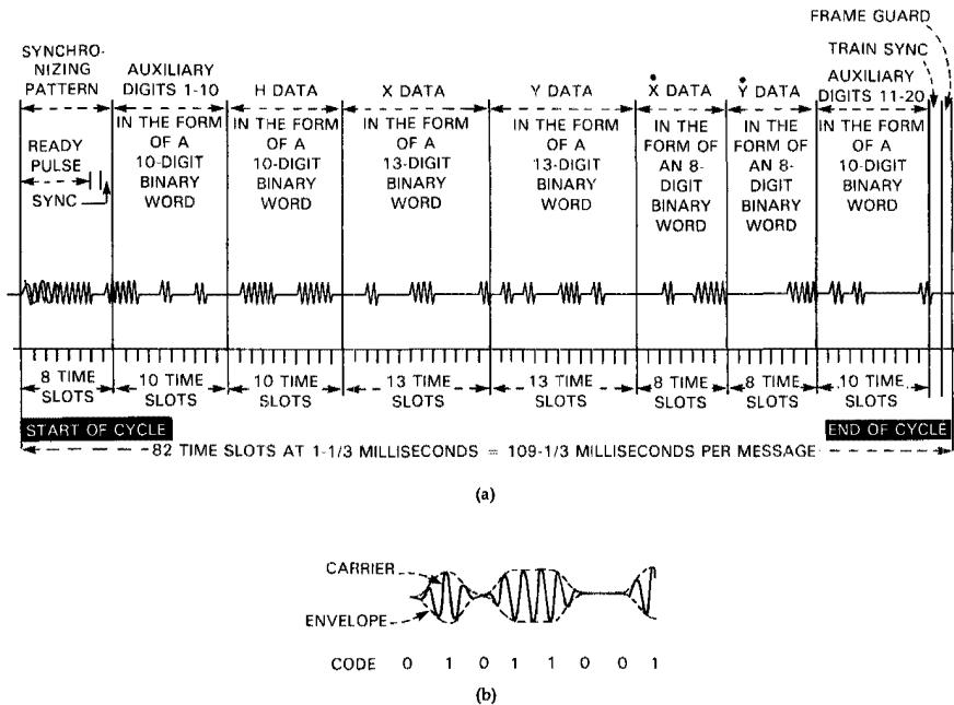
Fig. 10-12. Transmission of radar data with AN/TSQ-7 transmitter over ordinary telephone lines. The transmitter accepted voltages in analog form, converted these to binary digit form, and used the binary digits to control spurts of a carrier frequency applied to the telephone lines; the binary ones denoted the presence of spurts, and the zeros, the absence of spurts. (a) Typical transmitted message; X and Y data represent east-west and north-south location information, respectively, of detected aircraft, H its height, and \bar{X} and \bar{Y} its motion. (b) The line waveform for eight digits.
