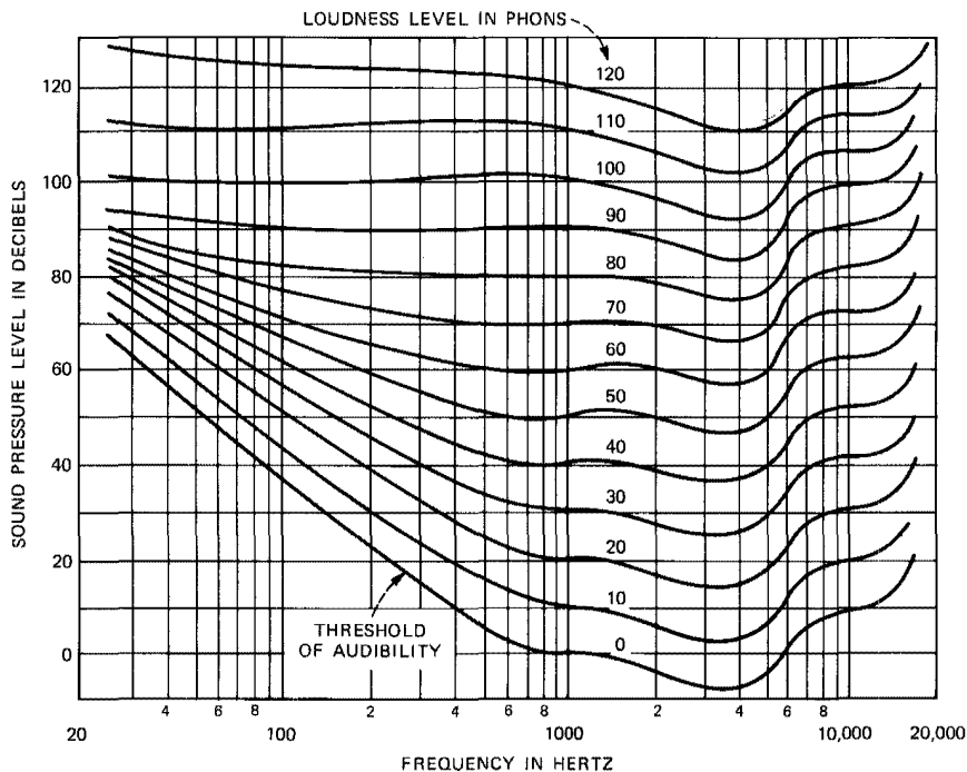
Fig. 2-4. Contours of equal subjective loudness as a function of loudness level in phons. At 1000 Hz, 0 dB corresponds to a pressure of 0.0002 dyne/cm 2 . [Fletcher and Munson, J. Acoust. Soc. Am. 5 (1933): 91.]
