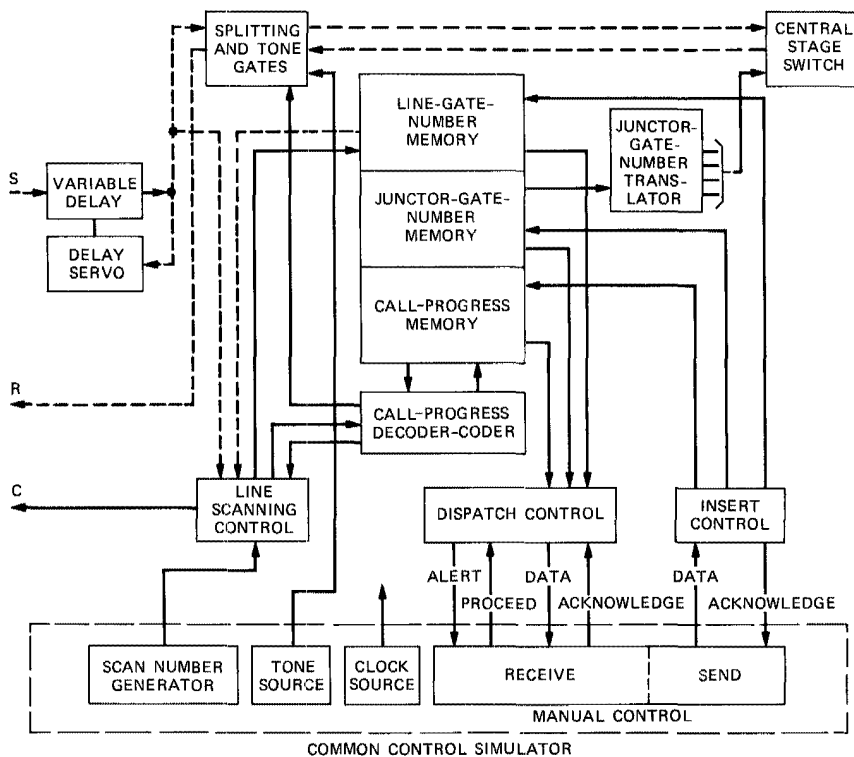
Fig. 8-12. ESSEX concentrator central unit. Each ESSEX line concentrator had an associated central unit with three memory sections, each recirculating a serial pulse train of binary-coded words. The line-gate-number memory stored the list of active line gate numbers for operation of the remote line unit. The junctor-gate-number memory stored words to control the operation of the central stage switch gates associated with the same concentrator. The call-progress memory stored code words concerning the states of the calls being handled. Words in the memories could be used for control in parallel or serial form and could also be received or transmitted in either fashion.
