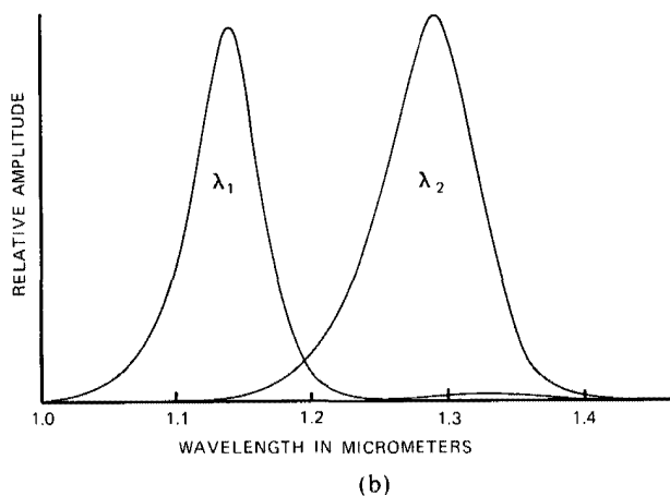
Fig. 7-16. Dual-wavelength LED and its emission spectra. (a) Cross-sectional view of a dual-wavelength LED composed of two independently driven p-n junction diodes in a single semiconductor chip; it can emit two wavelengths (e.g., 1.14 \mu\text{m} and 1.3 \mu\text{m} ) simultaneously. Such a device is useful for a light source in a wavelength-division-multiplexed lightwave system. The first active layer (Q 1 ) of In 0.77 Ga 0.23 As 0.5 P 0.5 is separated from a second active layer (Q 2 ) of In 0.66 Ga 0.34 As 0.75 P 0.25 by a thin InP barrier layer. All layers were grown by liquid-phase epitaxy onto an InP substrate, and p-n junctions were formed by a deep Zn-diffusion in the Q 1 layer and by a grown p-InP layer on the top Q 2 layer. Electrical isolation is accomplished by a chemically etched deep channel between the two junctions. (b) The emission spectra of the dual-wavelength LED. The electrical crosstalk between the two wavelengths was measured to be about -24 dB. [Lee, Burrus, and Dentai, Electron. Lett. 16 (1980): 845, 846.]
