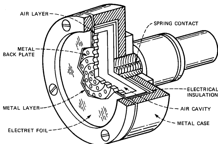
Fig. 2-19. Construction of an electret microphone.
