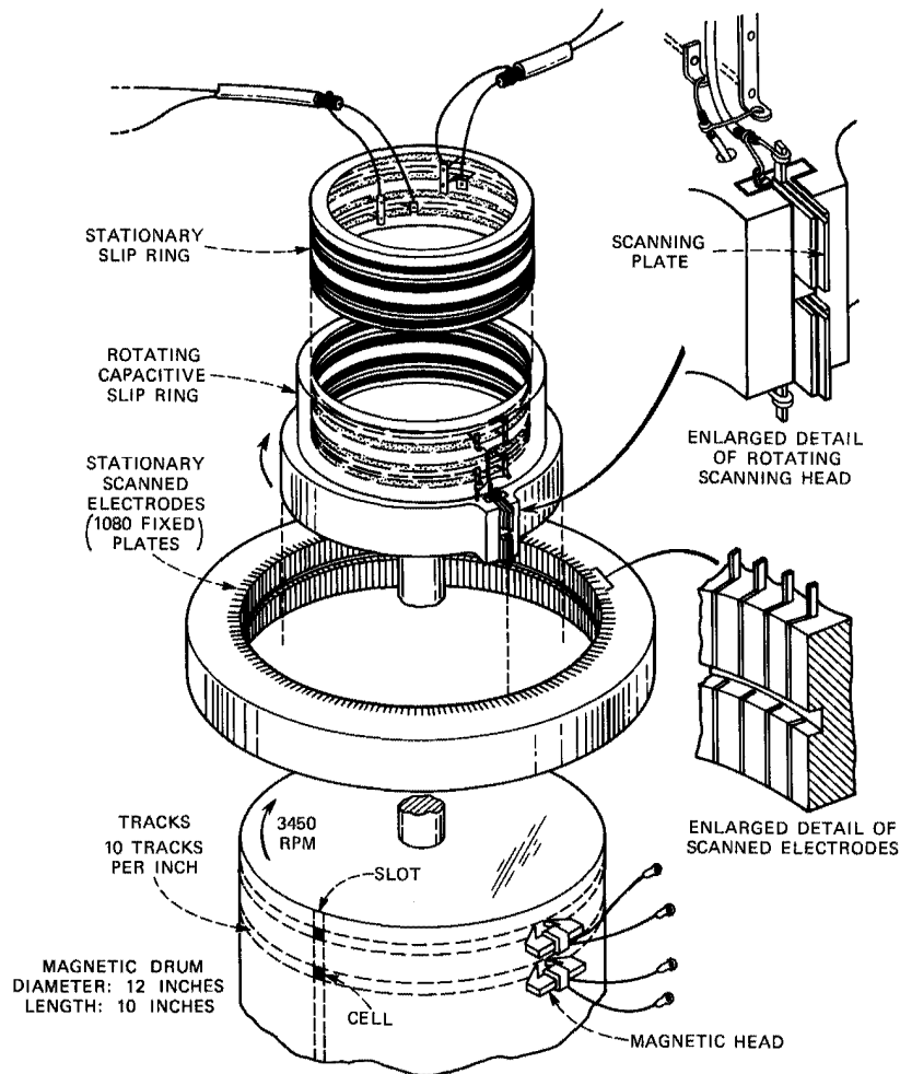
Fig. 8-6. DIAD drum and scanner. The memory of the DIAD system was in magnetizable cells on the surface of rotating drums. Rotating on the same shaft was a capacitively coupled scanning head used as a synchronized input path from lines and trunks. The 1080 electrodes of the stationary section of the scanner defined an equal number of axial areas or slots on the drum surface, each assigned to a corresponding line or trunk. All permanent and temporary data for the line or trunk were "remembered" in the magnetic cells of the associated slot and were read, and the call-related information was altered as required by the system program. The program itself was recorded in call-progress marks.
