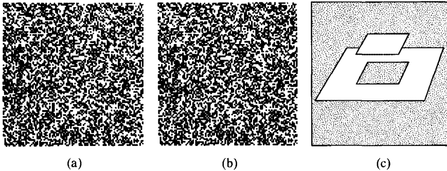
Fig. 11-14. Random-dot stereogram prepared by a program of B. Julesz. (a) and (b) Images seen by the left and right eyes are shown side-by-side in the figure. No patterns are perceptible in these separate images. (c) However, if the two images are fused, then a vivid pattern of depth variation can be seen in the fused image. [Julesz, Sci. Amer. 212 (1965): 43.]
