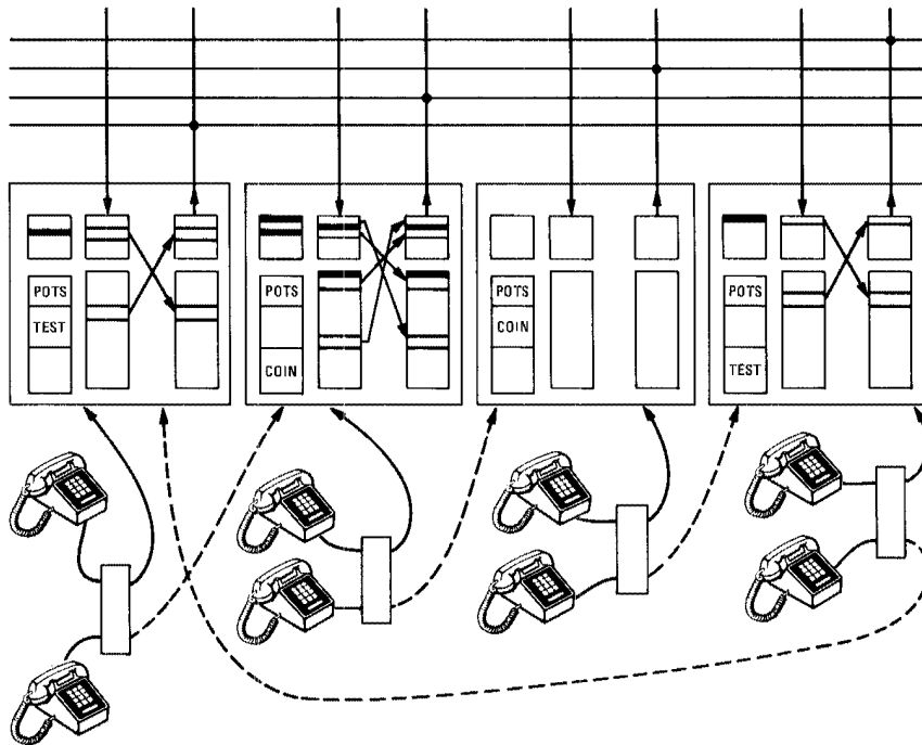
Fig. 8-16. The multiple module XDS system architecture. Up to 100 individual XDS modules could be interconnected using a large time-division multiplexed switch. Each module controlled and transmitted information on its own bus and received information from any of the other buses. Programs could be stored in separate modules and yet be used by all modules. For example, the Plain Old Telephone Service (POTS) feature is shown in all modules; the coin telephone program (COIN) is only shown in two modules but could be used by any of the modules.
