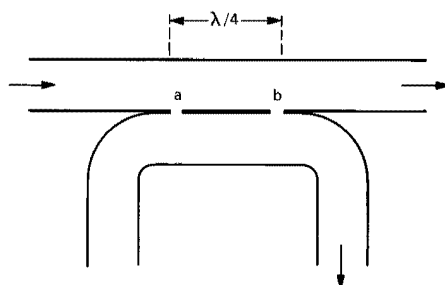
Fig. 6-10. A simple form of directional coupler. Two openings, a and b , placed a quarter wave-length apart, allow transmission in the forward direction and cancellation in the backward direction. [Southworth, Principles and Applications of Waveguide Transmission (1950): 346.]
