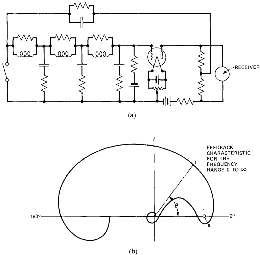
Fig. 1-17. Nyquist's amplifier. (a) An adaptation of one of H. Nyquist's patent diagrams of a feedback amplifier. (b) The amplifier's related diagram. The diagram is a plot, in the complex plane, of the path traced out by the complex loop gain \mu\beta as the frequency is varied. The path encircles the point 1, showing that the amplifier is unstable. The amplifier is unusual because it becomes stable if the vacuum tube is replaced by one of higher gain.
