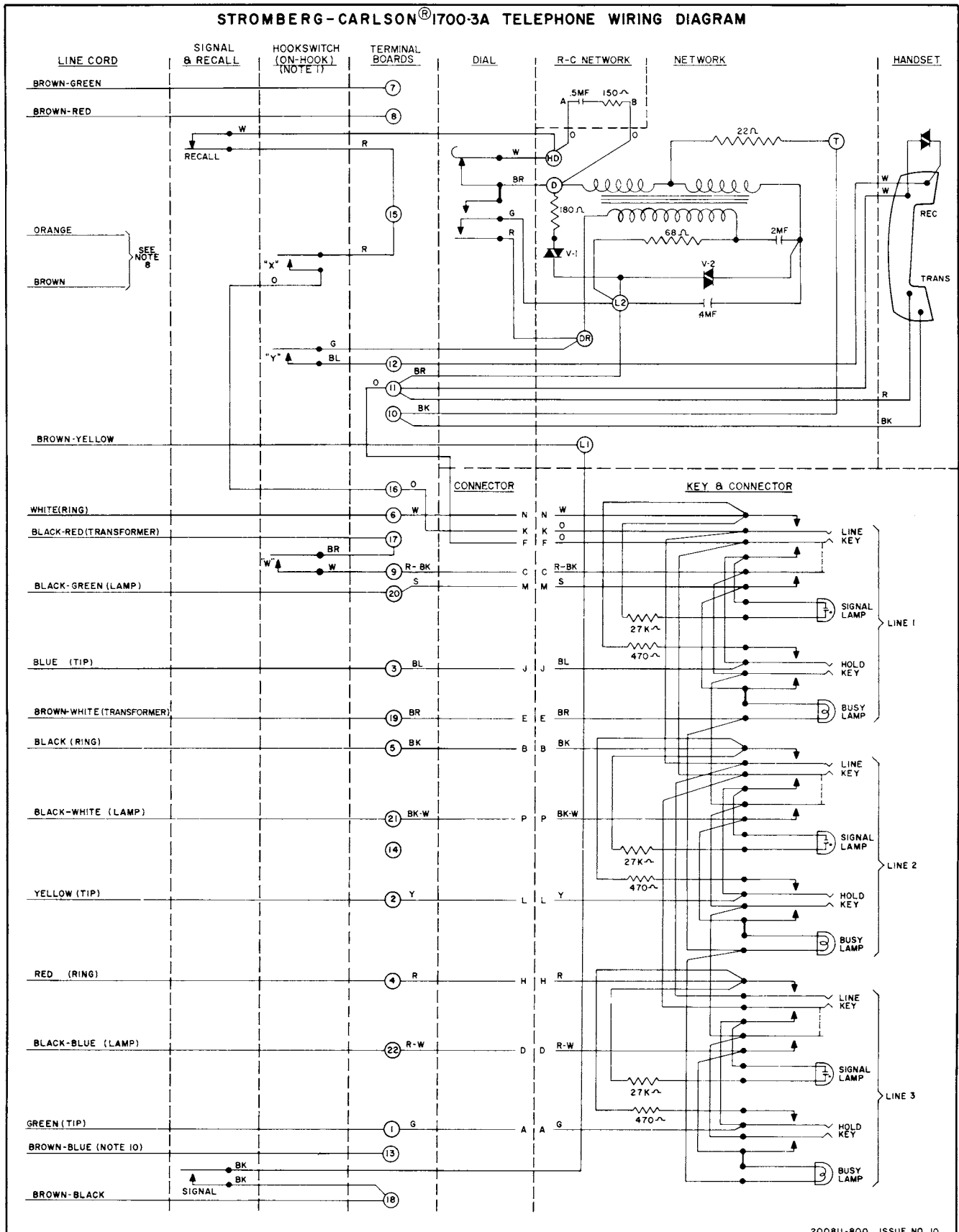
Figure 9. Wiring Diagram. 1700-3A Telephone, Sheet 1
