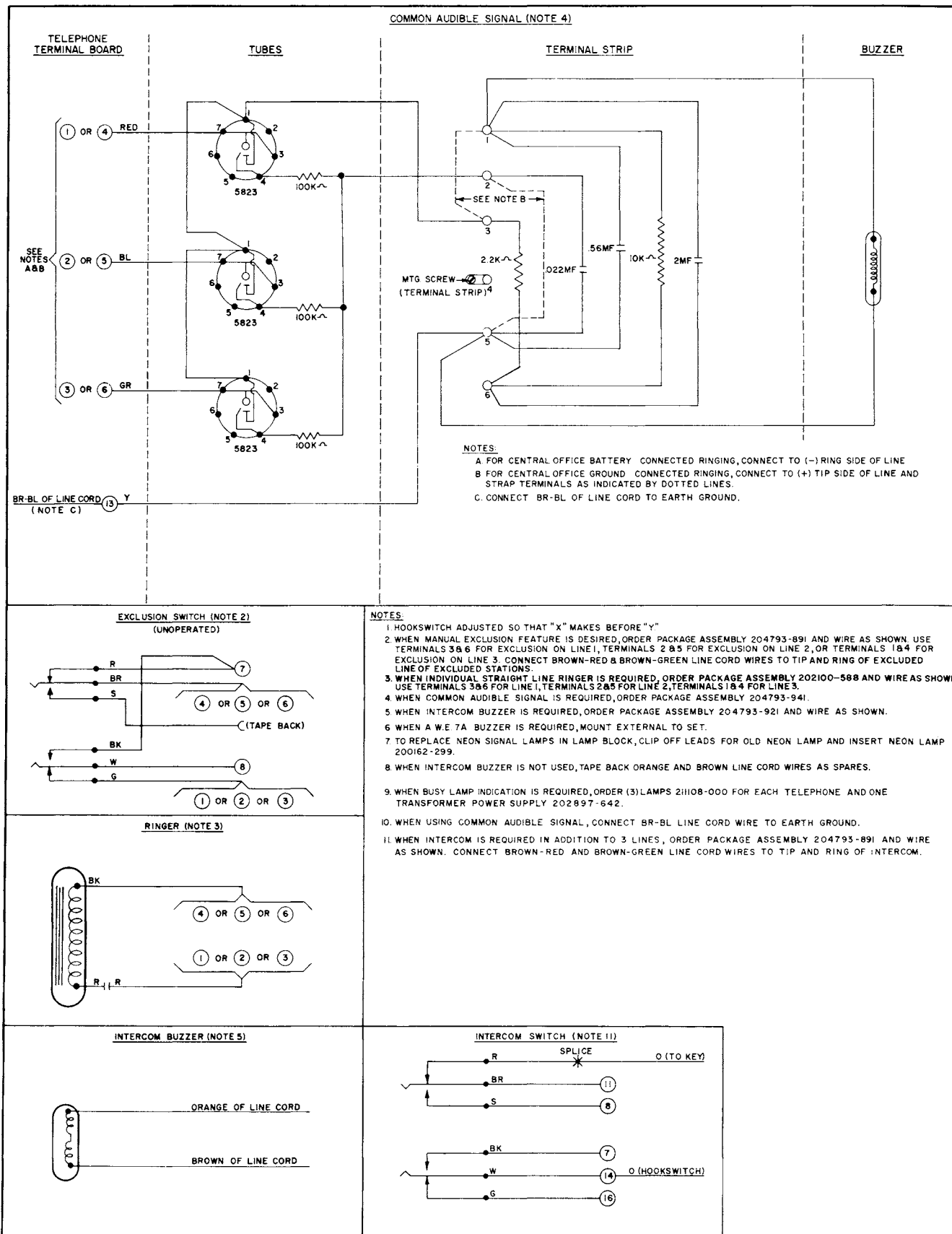
TCI Library: www.telephonecollectors.info Figure 9. Wiring Diagram. 1700-3A Telephone, Sheet 2
