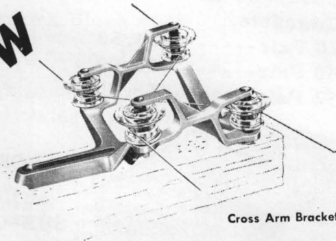
Case Transposition Brackets
