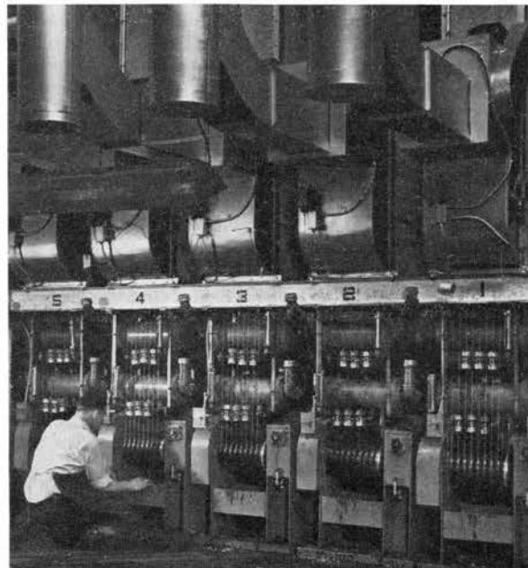
Stromberg-Carlson Lacquer Towers for coating miles of copper wire.
