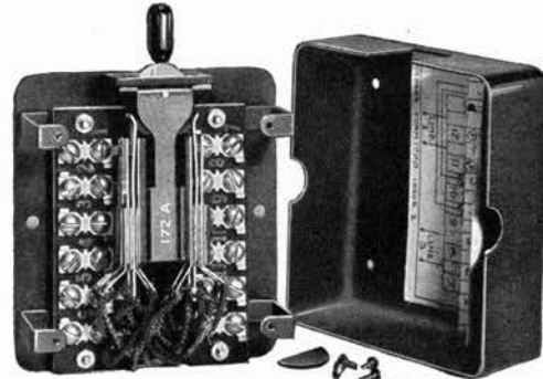
No. 13 Key Box—Open
