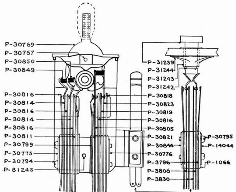
Line Drawing showing parts of the No. 350 Key
