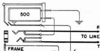
Line Circuit arranged for central checking line
