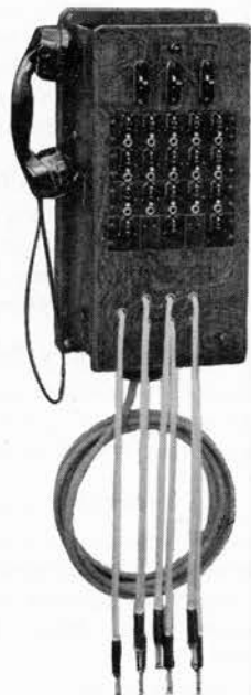
No. 126 Magneto Switchboard Capacity—15 Drop Lines
