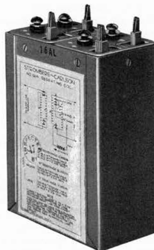
The Stromberg-Carlson No. 16-AL Repeating Coil which makes possible the use of Common Battery Telephones with Magneto Lines.
