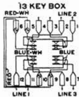
Wiring Diagram No. 13 Key Box
