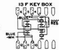
With No. 343-E Locking Key
