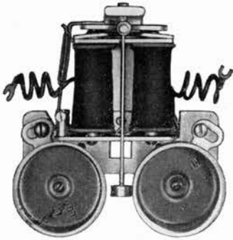
No. 65 Ringer With Biasing Spring
