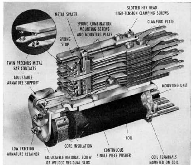
"A" Type Relay
