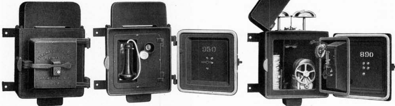
No. 950 BY Ironclad Telephone Open View No. 950 BY Ironclad Telephone No. 890 Generally Similar to the above No. 950.
