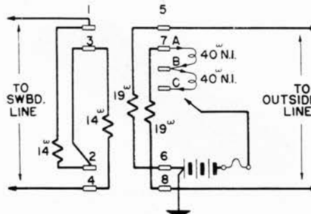
No. 16-AL Talk-Through, Ring-Through Repeating Coil, Connection Diagram
