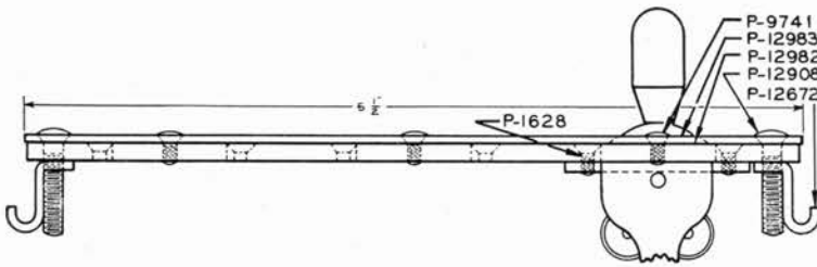
Above: Line Drawing shows Parts of No. 88 Key Mounting
