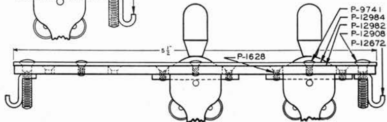
Below: Line Drawing shows Parts of No. 89 Key Mounting.
