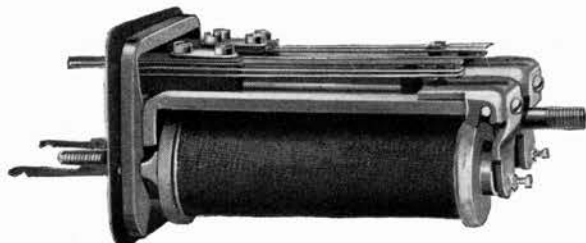
Two No. 200 Type Relays mounted on Relays Casing Support
