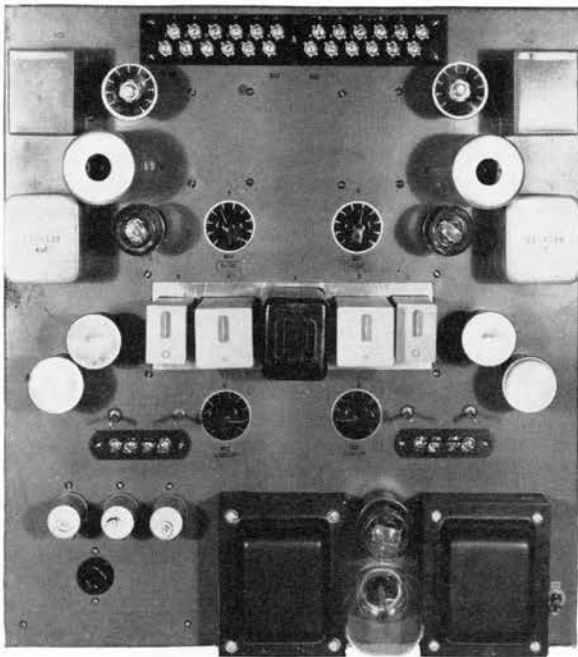
A Typical Adler Carrier Repeater Unit Rack Mounted for Interchangeability
