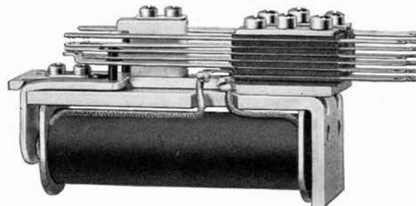
No. 500 Type Relay
