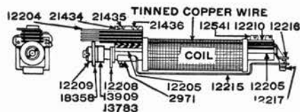
Parts Drawing of No. 190 Type Relay
