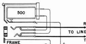
Line Circuit of No. 125 Switchboard with double cut-off jacks
