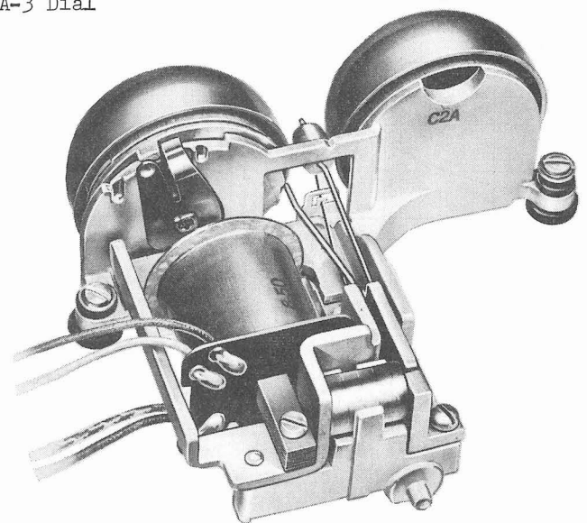
Fig. 12 - C2A Ringer
