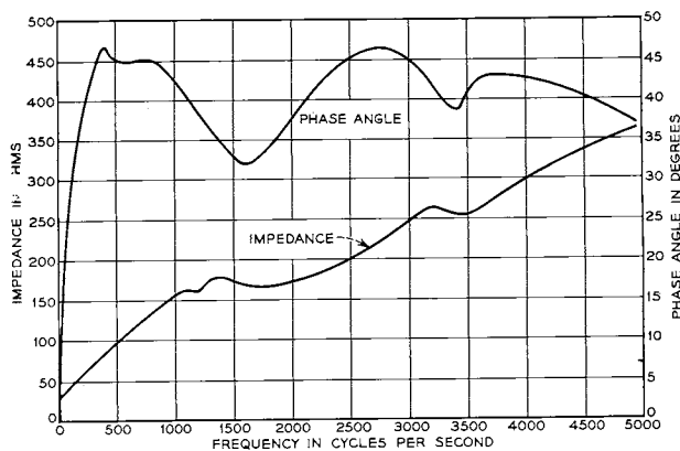
Fig. 10 - Impedance of UL Receiver
