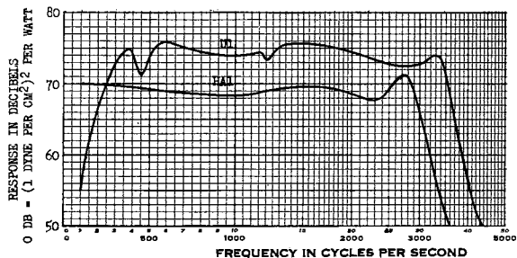
Fig. 9 - Available Power Response-Frequency Characteristics of UL and HAL Receivers in Standard Handles Measured on a 6 cc Coupler
