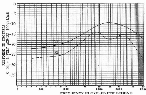
Fig. 6 - Frequency Response of T1 and F1 Transmitters Measured in Standard Handles with Constant Sound Pressure Applied at Modal Distances
