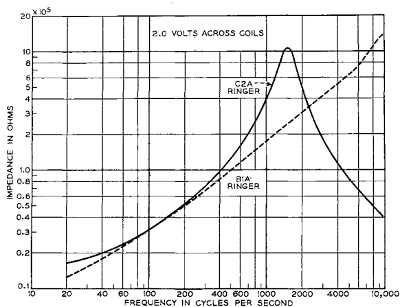
Fig. 13 - Impedance Characteristics of C2A and B1A Ringers
