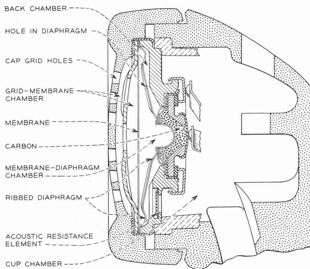
Fig. 5 - T1 Transmitter - Sectional View in G1 Hand Set
