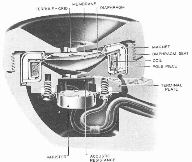
Fig. 7 - U1 Receiver - Sectional View in G1 Hand Set
