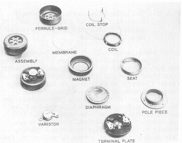
Fig. 8 - U1 Receiver Parts
