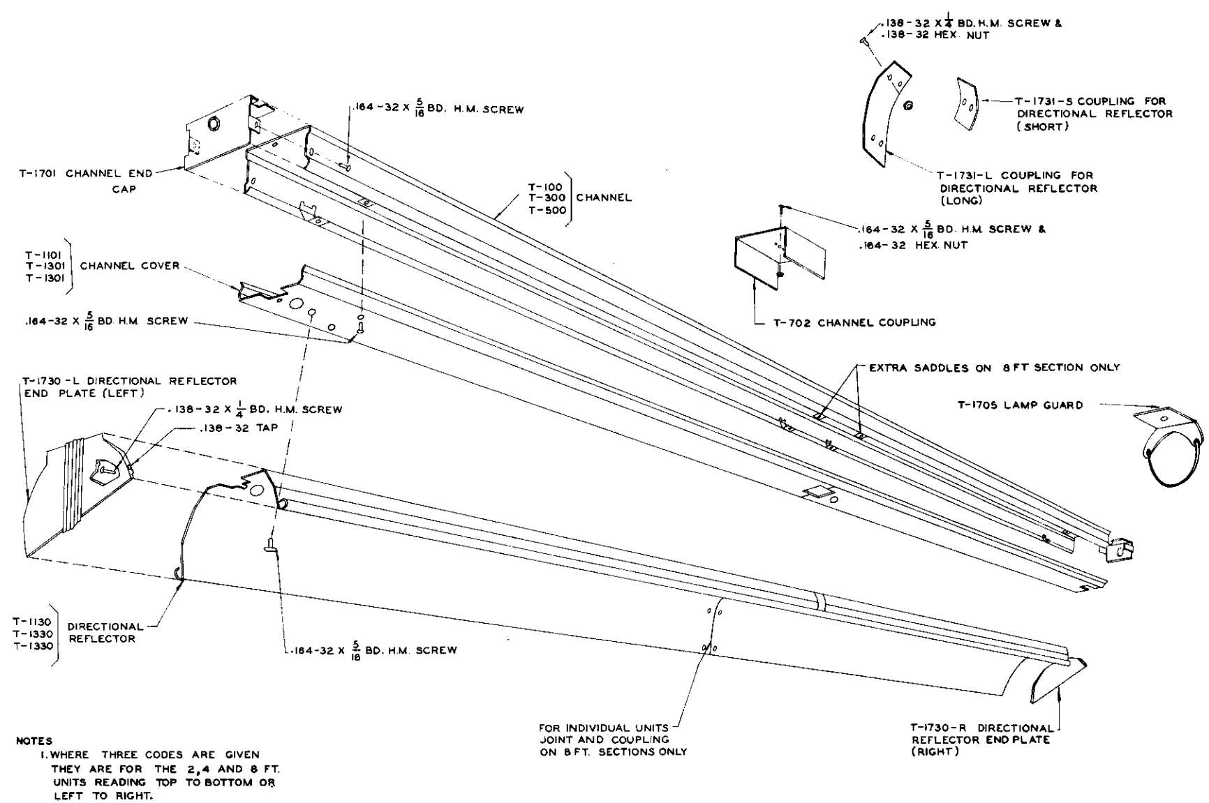
Fig. 3 - Fluorescent Lighting Fixtures Details for One-lamp Units
