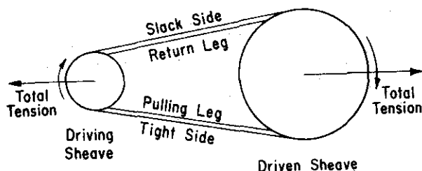
Fig. 4 - V-Belt Drive
