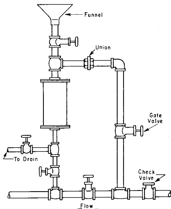
Fig. 1 - Bypass Feeder
