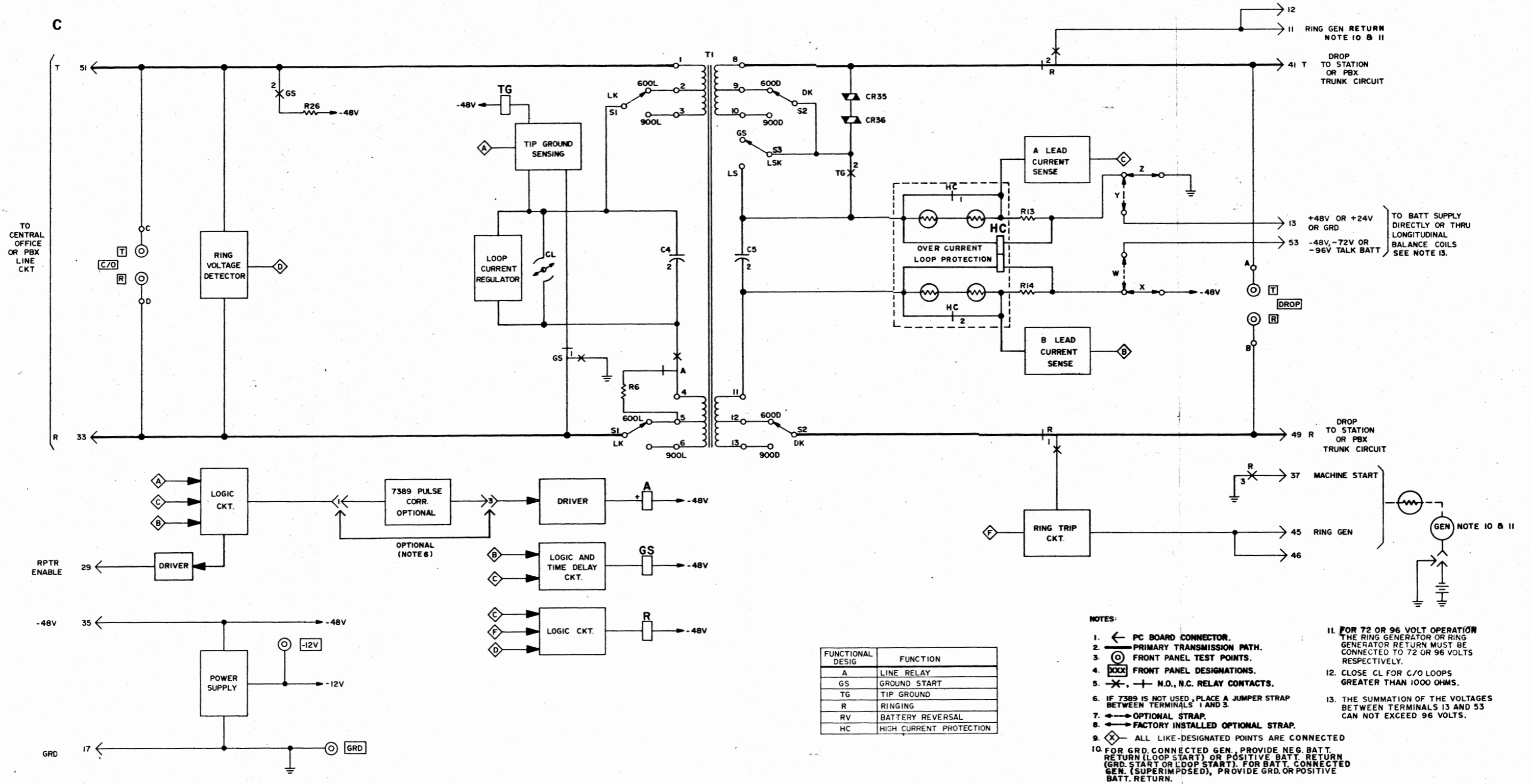
Figure 4. 7376 Functional Block Diagram (Issue 2)
