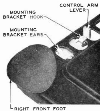
FIG. 8—MOUNTING BRACKET
