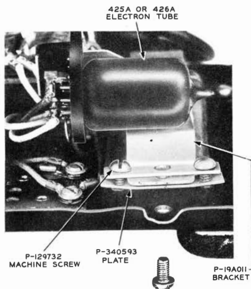
FIG. 4—ELECTRON TUBE BRACKET ASSEMBLY
