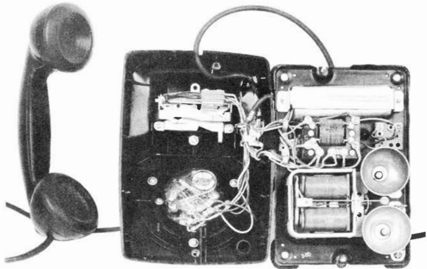
FIG. 1B—INTERIOR VIEW
