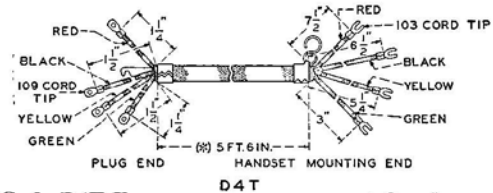
Code D4T Type 4 Conductors
