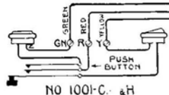
NO 1001-C &amp; H
