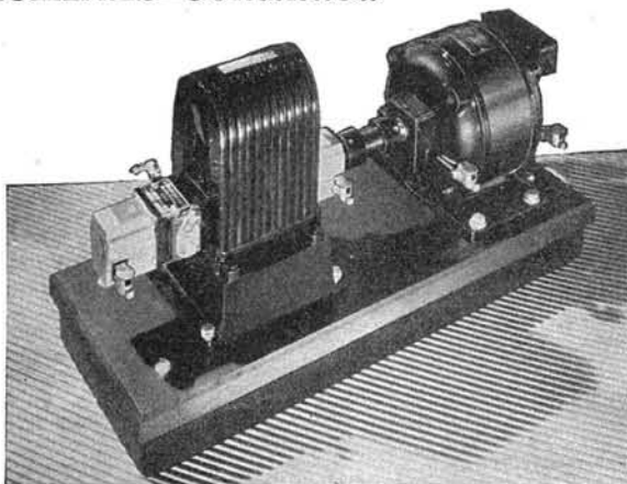
Motor Generator Ringing Set
