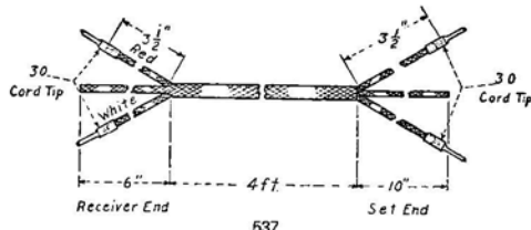
Code 537 2 Conductors (Water-proofed Rubber Covered Conductors) Black Cotton Covered. Receiver Cord intended for use with 19A Test Set.
