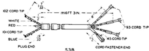
Code S3B S3B 3 Conductors
