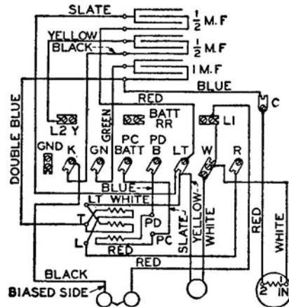
Wiring diagram No. 634BB Subscriber Set
