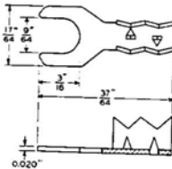
No. 103 Nickel Finished
