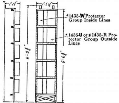
No. 1420B Distributing Frame
