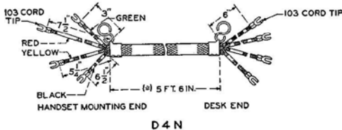
Code D4N Type 4 Conductors
