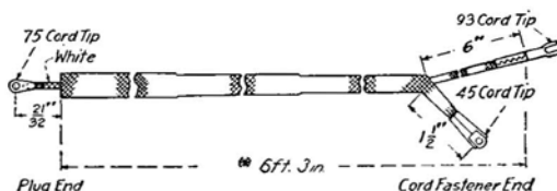
Code S1A S1A 1 Conductor
