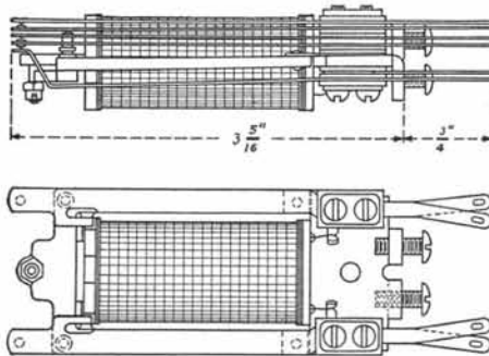
NO. R-7 ALSO GENERAL DESIGN AND DIMENSIONS OF “R” TYPE
