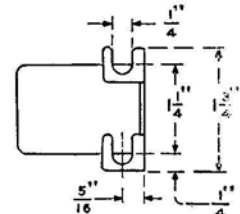
Dimensional Drawing of No. 146A
