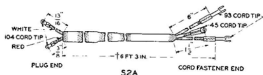
Code S2A S2A 2 Conductors
