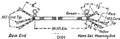
Code D3H Type 3 Conductors
