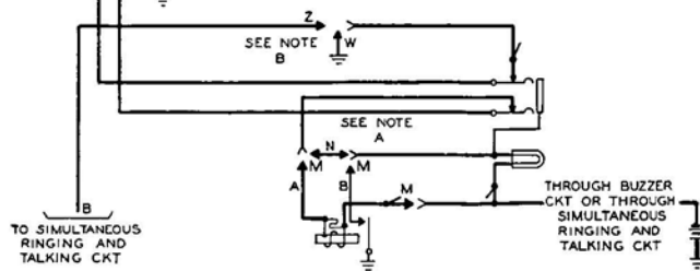
Station Line Circuit—"System C"
