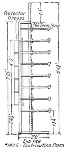
*1425 - Distributing Frame
