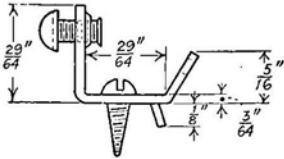
No. 9 Cord Fastener
