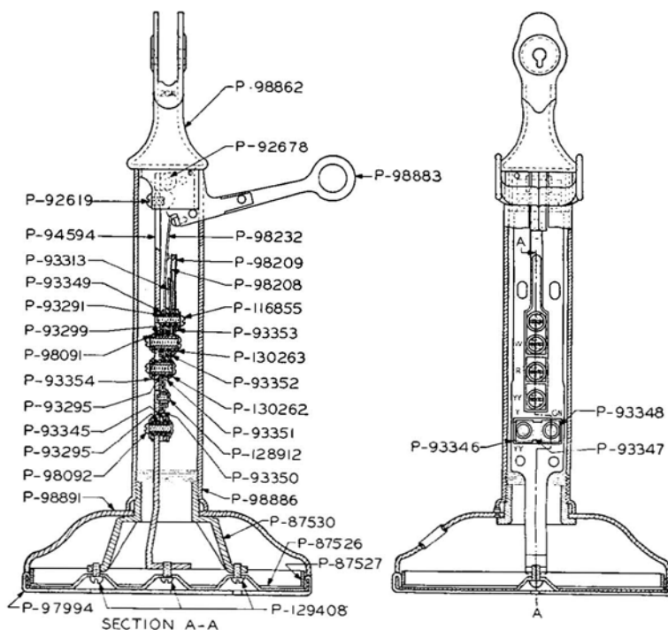
NO. 20-AL DESK STAND
