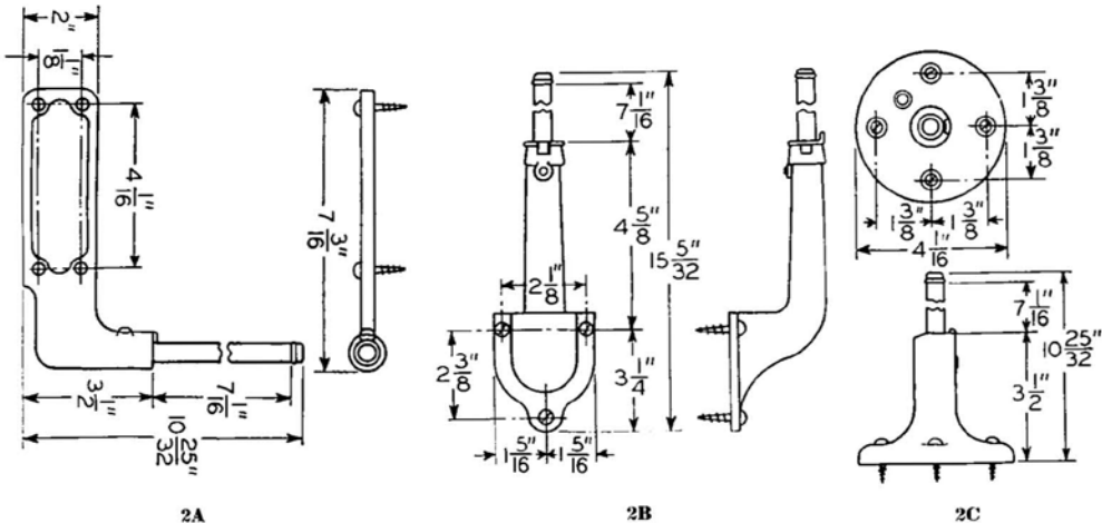
Transmitter Arm Brackets
