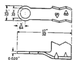
No. 102 Nickel Finished
