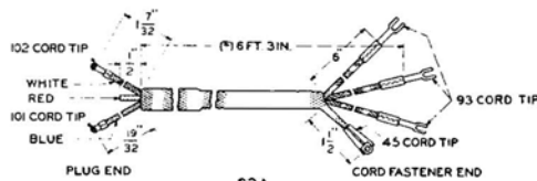
Code S3A S3A 3 Conductors
