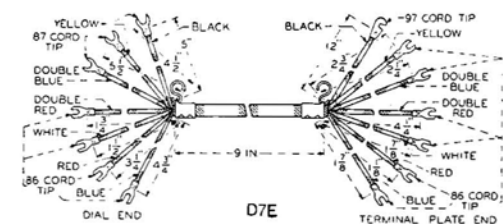
Code D7E (Moisture-proofed) 7 Conductors
