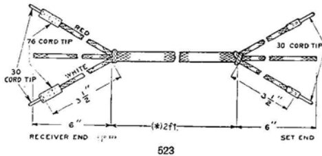
Code 523 (Water-proofed) 2 Conductors Black Cotton Covered. (*) 2 1/2 ft. cords can be furnished when specified. Linemen's Receiver Cord, intended for use with 6 and 17 Type Test Sets. Replaces 15 and 522.
