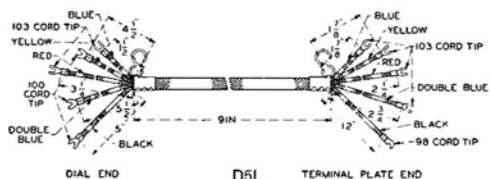
Code D5L 5 Conductors
