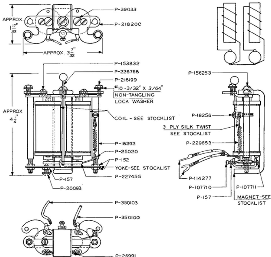
No. 68JA Ringer
