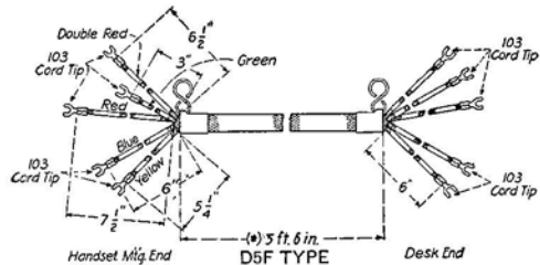
Code D5F Type 5 Conductors
