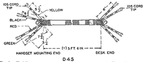
Code D4S 4 Conductors (Water-proofed Rubber Covered Conductors) Cotton Covered.
