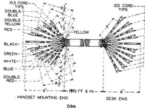
Code D9A Type 9 Conductors Intended for use with 205D, 205E, or 205F Type Hand Telephone Sets.
