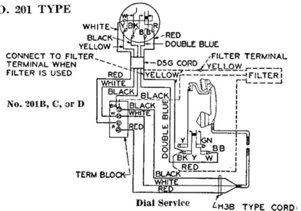
Dial Service H3B TYPE CORD
