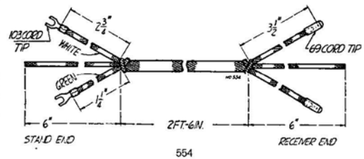
Code 554 (Moisture-proofed) 2 Conductors Black and Maroon Cotton Covered.
