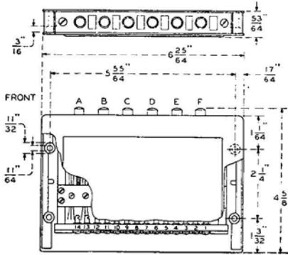
Dimensional Drawing
