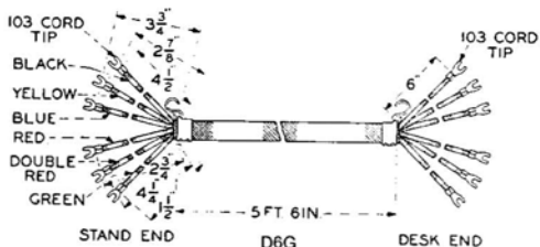
Code D6G (Moisture-proofed) 6 Conductors
