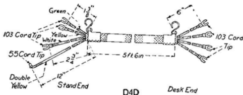
Code D4D (Moisture-proofed) 4 Conductors
