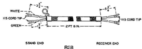
Code R2B 2 Conductors
