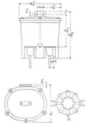
Wiring Diagram No. 121A
