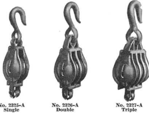
Malleable Iron Shells—Loose Side Hooks and Becketts
