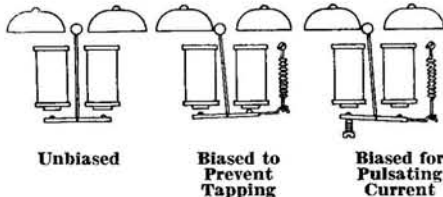
No. 8 Type Ringer
