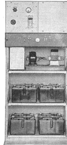
Front view of power equipment showing small motor driven magneto generator and one rectifier
