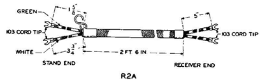
Code R2A 2 Conductors
