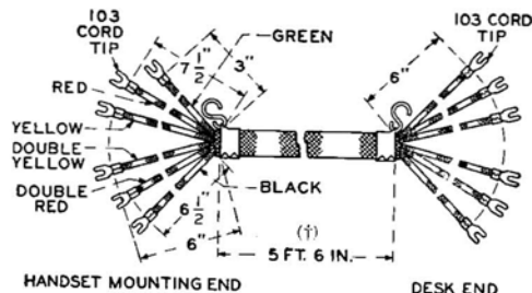
Code D6H Type 6 Conductors
