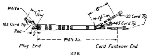
Code S2B S2B 2 Conductors
