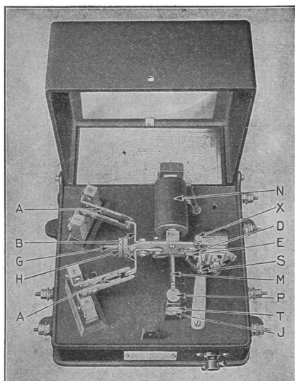
Top View of No. 84D Interrupter
