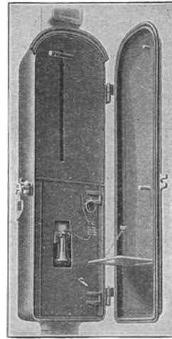
Selector Signal Mechanism, and Telephone Apparatus Case
