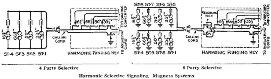
Harmonic Selective Signaling—Magneto Systems
