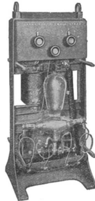
Type AT Rectifier Cover Off
