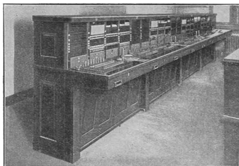
Toll Multiple Switchboard, Lynchburg, Virginia
