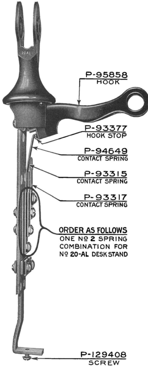
No. 20-AL DESK STAND
