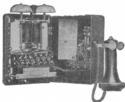
No. 1333 Telephone—Open
