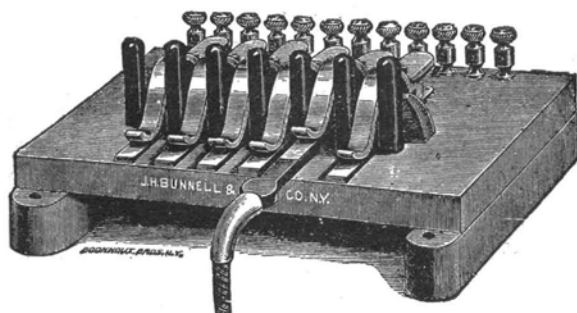
No. 1268 Spring Jack
