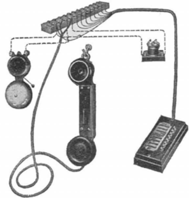
No. 6034 Type Hand Set Inter-phone
