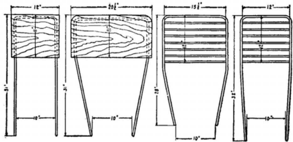
Pole Seats
