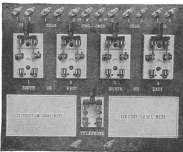
No. A-102412 Switching Panel
