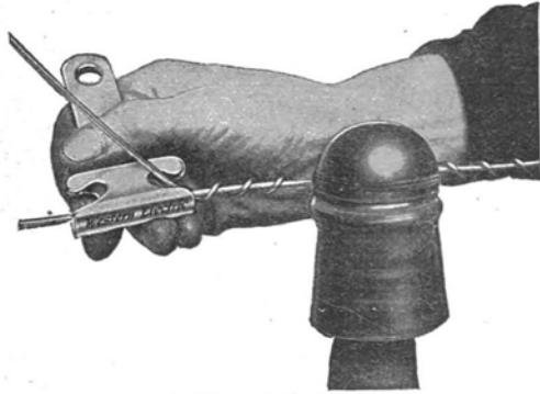
Method of "Tying In" with Tie Wrench
