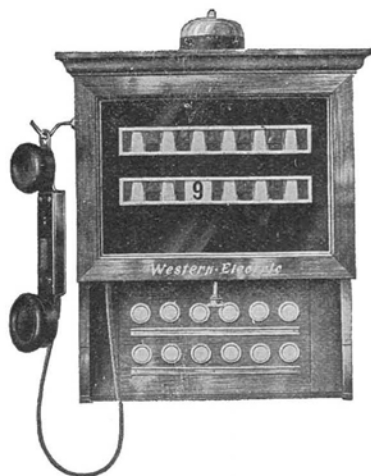
No. 36005 Master Station Two-way Service
