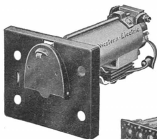
No. 30C Supervisory Signal Shutter Restored
