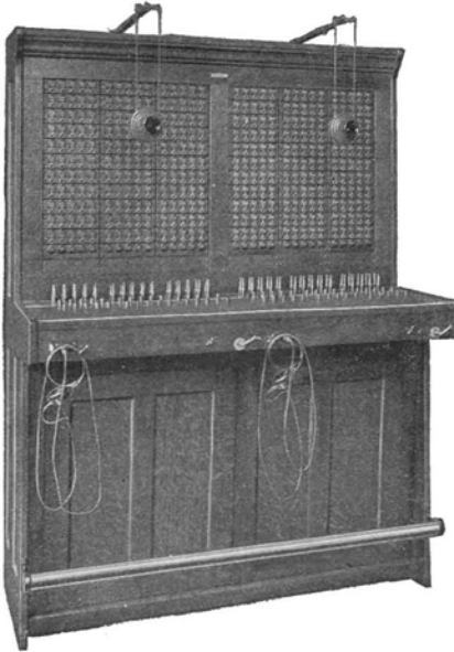
No. 1250D Switchboard
