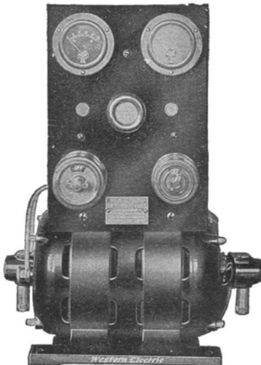
Battery Charging Unit, Front View
