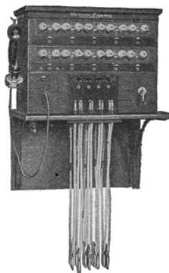
Wall Type—20 Lines Consists of: 1—AA-1 Top Unit 1—BA-7 Line Unit 1—BB-7 Line Unit 1—CA-1 Cord Unit 1—D-1 Supporting Unit
