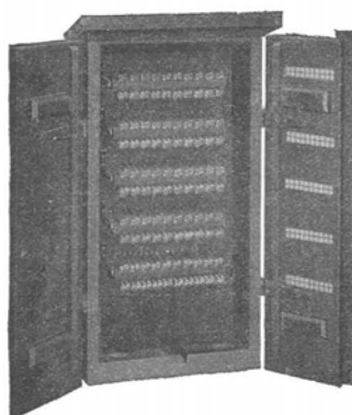
No. 15A Cable Terminal Open, with Protectors
