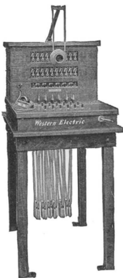
Floor Type—20 Lines Consists of: 1—AA-2 Top Unit 1—BA-12 Line Unit 1—BA-13 Line Unit 1—CA-6 Cord Unit 1—D-3 Supporting Unit
