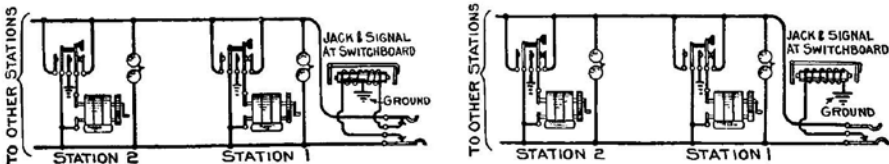
Double Wound Drop Wiring of Telephones and Switchboard Apparatus When No. 1002A Push Buttons Are Used
