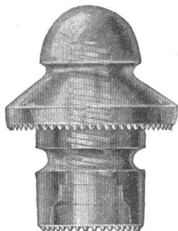
No. 51 Perfect Transposition
