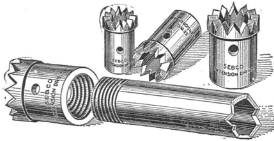
Extension Drills
