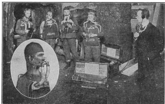
Mine Rescue Crew Using Rescue Telephone Apparatus
