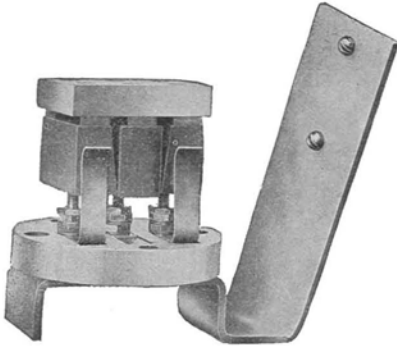
No. 86A Protector. Cover Removed
