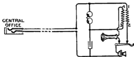
FIG. 1 Circuit of Induction Coil Telephone
