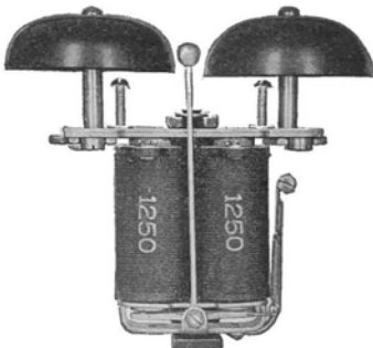
Ringer
