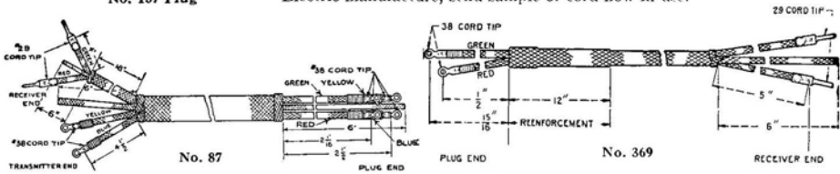
No. 87 Cord Attached to No. 103 or No. 137 Plug
