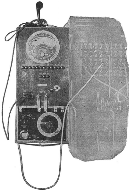
No. 1407 Testing Cabinet with No. 1407 Bridge Unit Attached to the Side of a No. 1200 Type Switchboard
