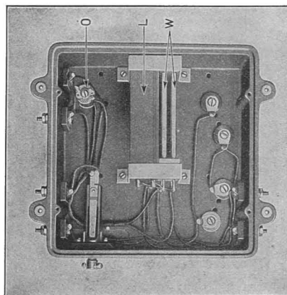
Bottom View of No. 84D Interrupter
