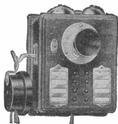
No. 1327 Type Wall Inter-telephone
