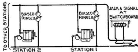
Wiring of Telephones for Center Checking Service
