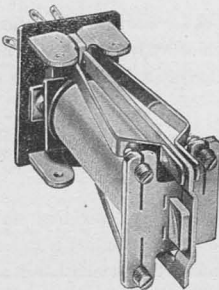
"B" Type, Cover Removed Telephone Apparatus and Supplies
