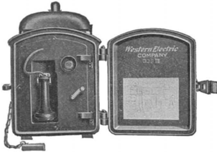
No. 1336 Mine Telephone (Outer Door Open)
