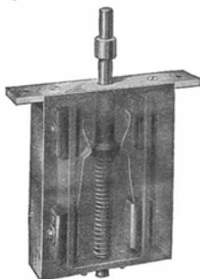
No. 1A Booth Switch
