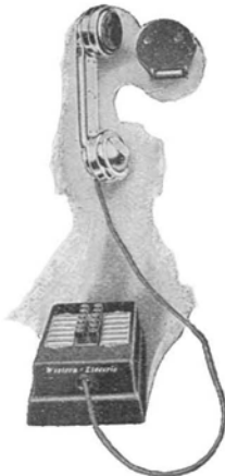
No. 6016 Type Hand Set Inter-phone
