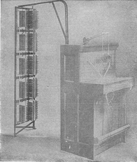
No. 1430D, E or F—Main Distributing Frame
