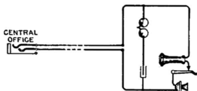
FIG. 2 Circuit of Series Telephone
