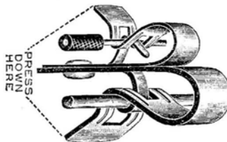
No. 31 Line Connector
