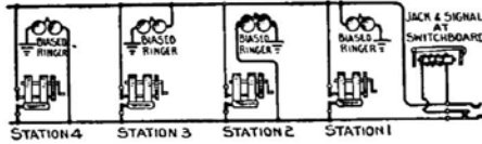
Pulsating Current 4 Party Selective Signaling—Magneto Systems
