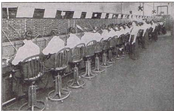
Central Battery Multiple Switchboard at Yonkers, N. Y.
