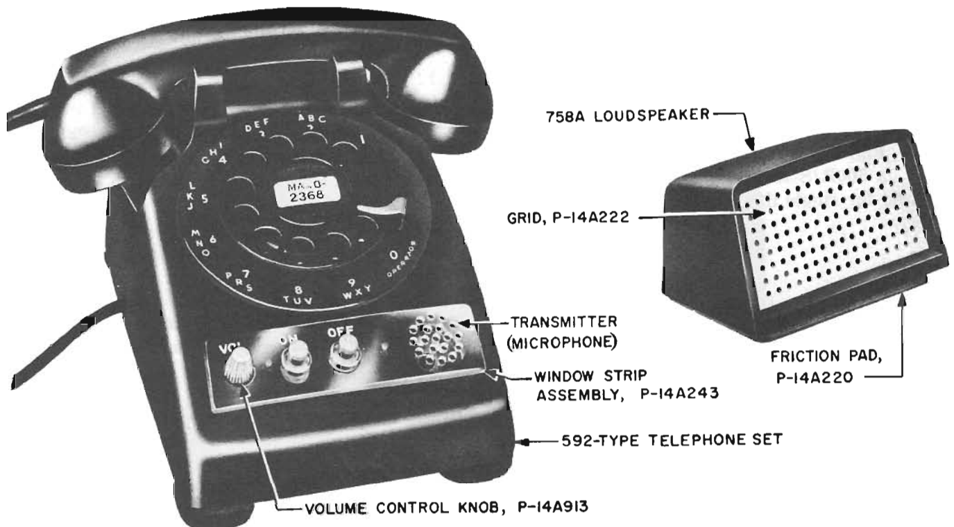
Fig. 1 — Speakerphone Components, Microphone in Base of Set
