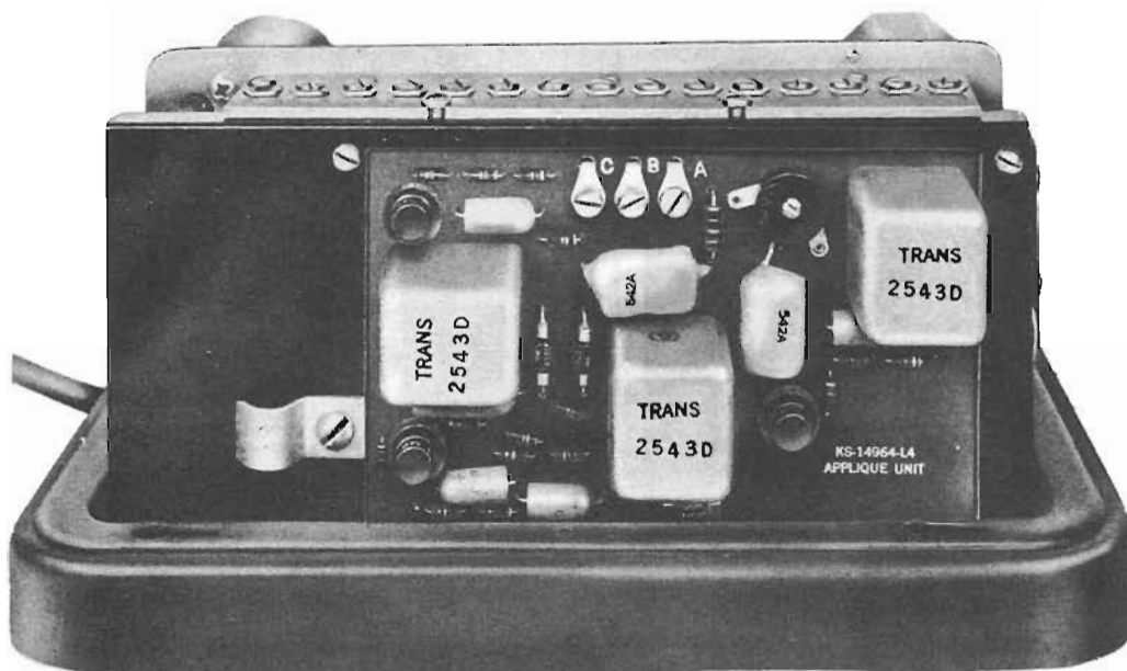
Fig. 6 — KS-14964, List 3 Control Unit, Side View
