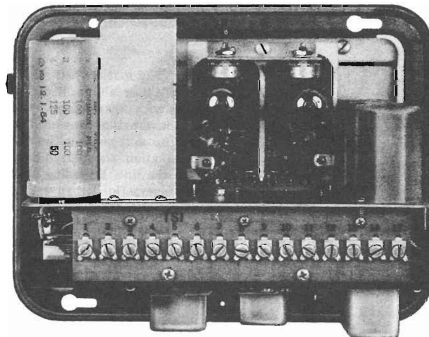
Fig. 5 - KS-14964, List 3 Control Unit, Top View
