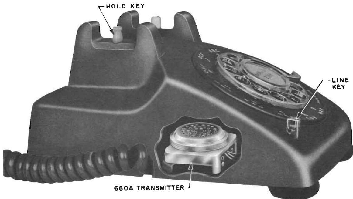
Fig. 4 — 511C/D Telephone Set Modified to Include 660A Transmitter Unit
