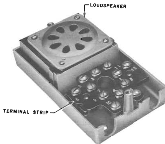
Fig. 8 — 759A Loudspeaker
