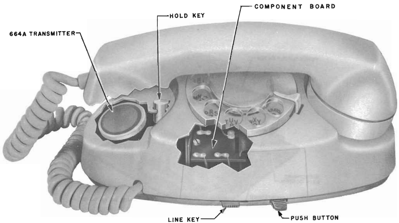
Fig. 6 — 711B Telephone Set Modified to Include 664A Transmitter Unit
