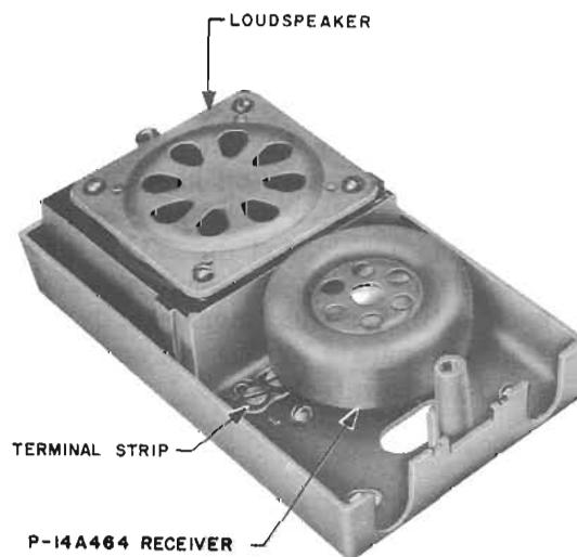
Fig. 9 — 730A Receiver
