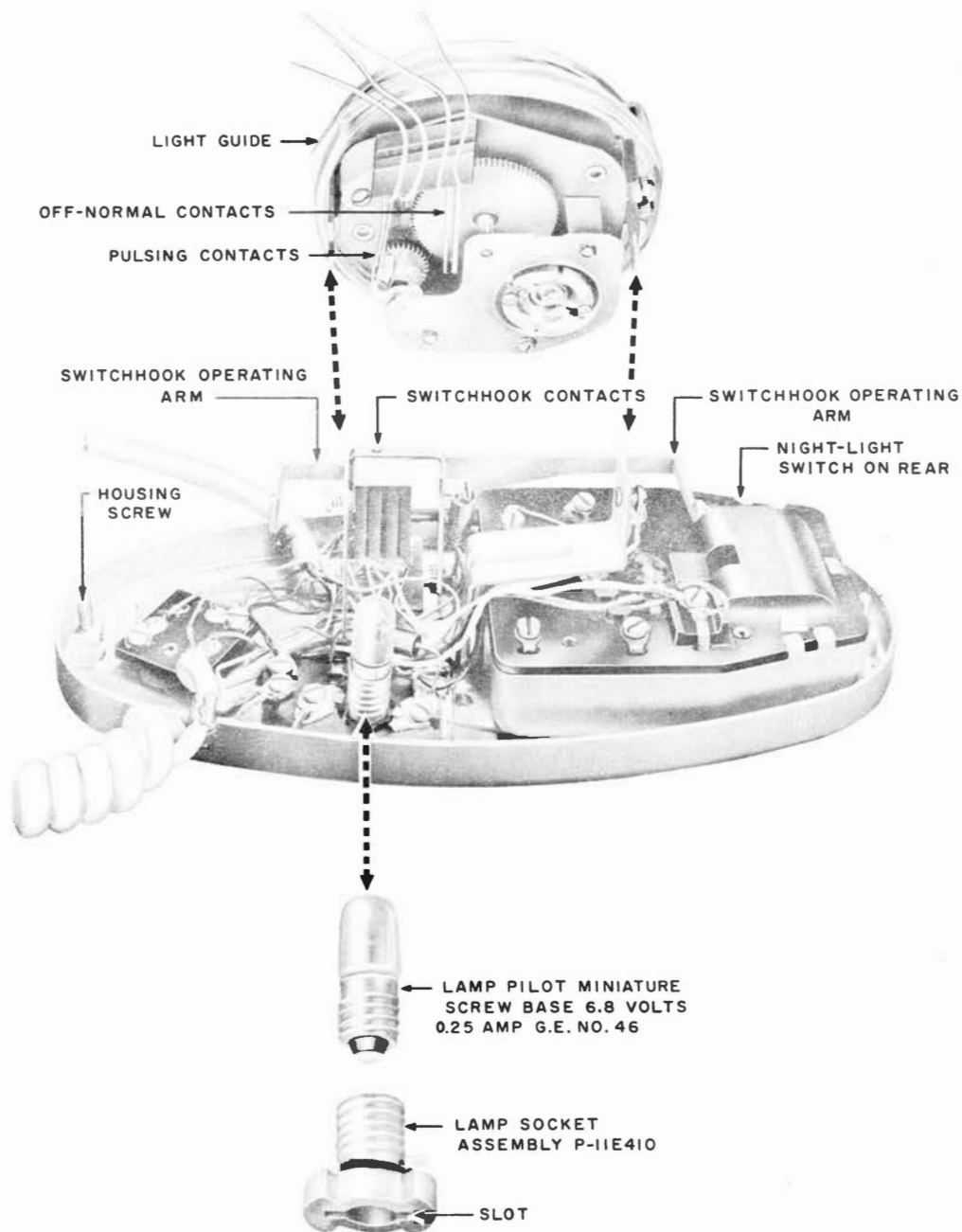
Fig. 3 — 701B Telephone Set with Dial and Lamp Socket Removed
