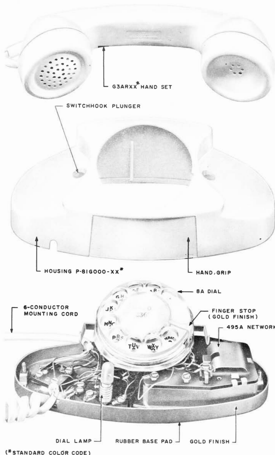
Fig. 2—701B Telephone Set with Housing Removed
