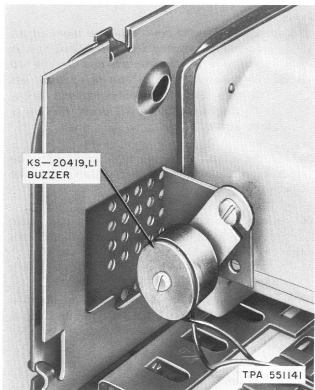
Fig. 15—Buzzer Mounting, Current Model
