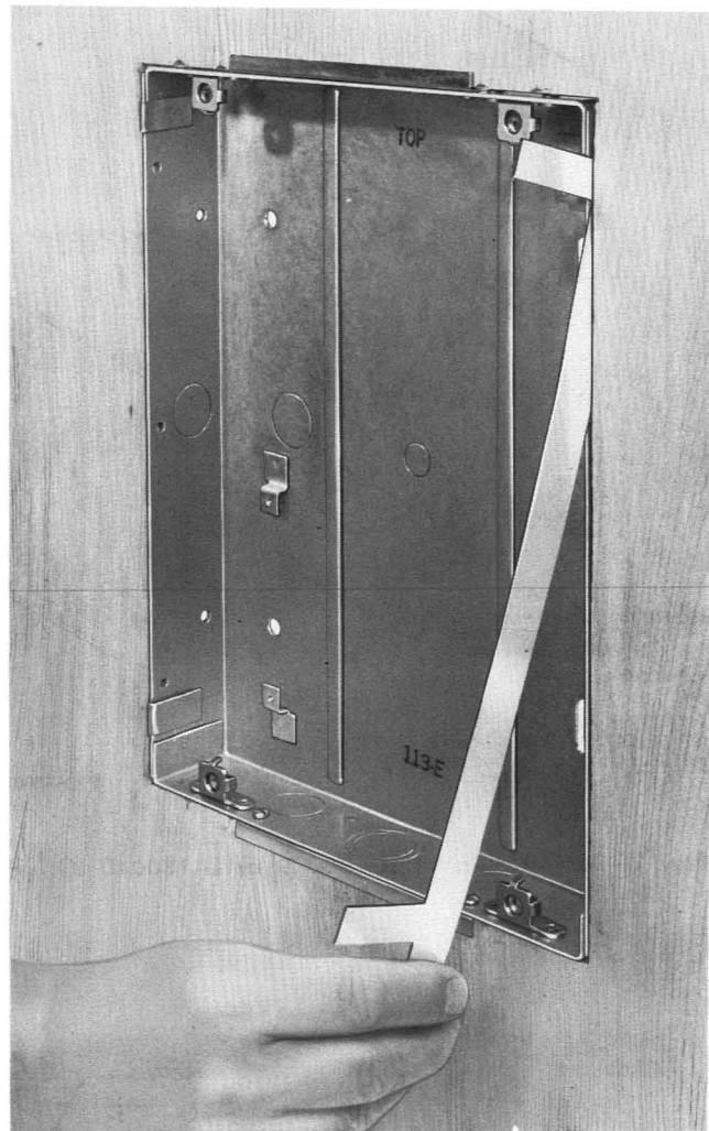
Fig. 5—Installation of Clips from D-179941 Kit of Parts on 113E Apparatus Box
