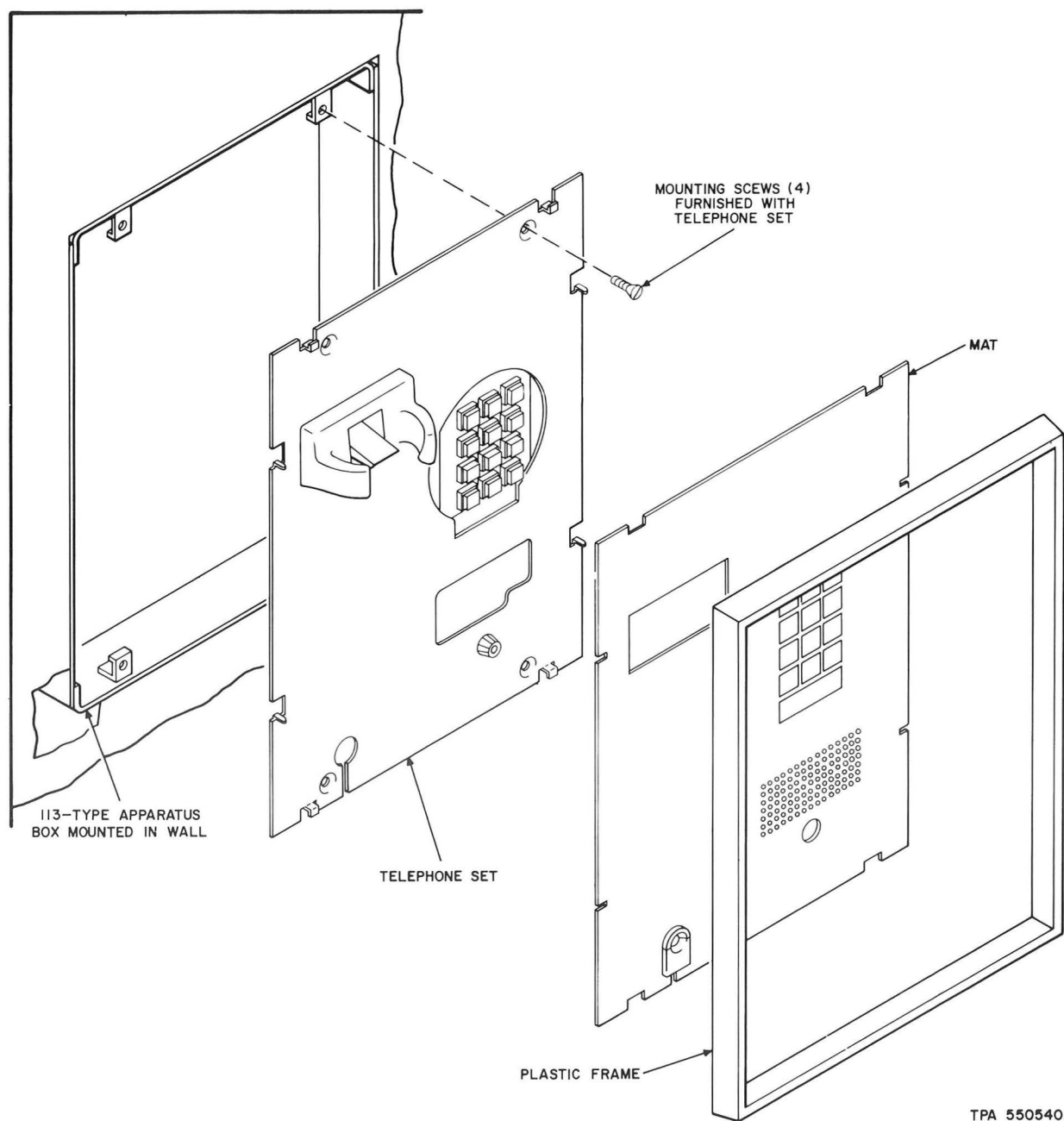
Fig. 1—Typical Installation of Panel Type Telephone Set (Recess Mounting)
