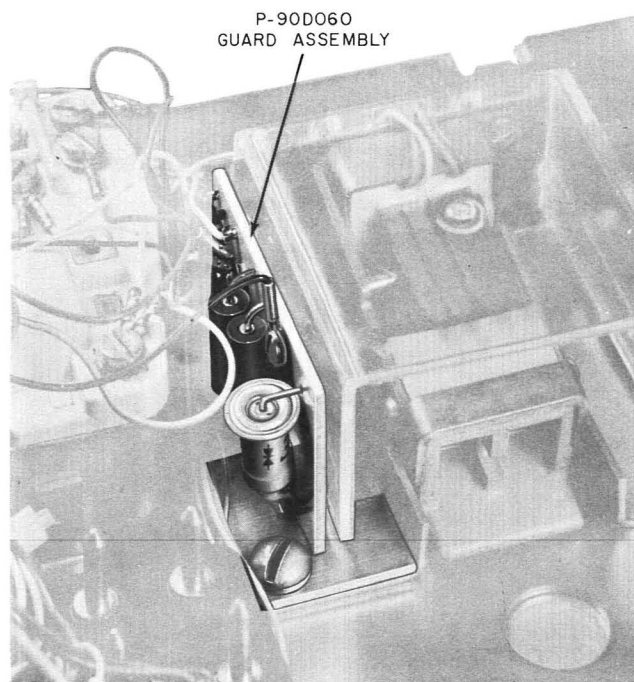
Fig. 13—P-90D060 Polarity Guard Assembly Installed
