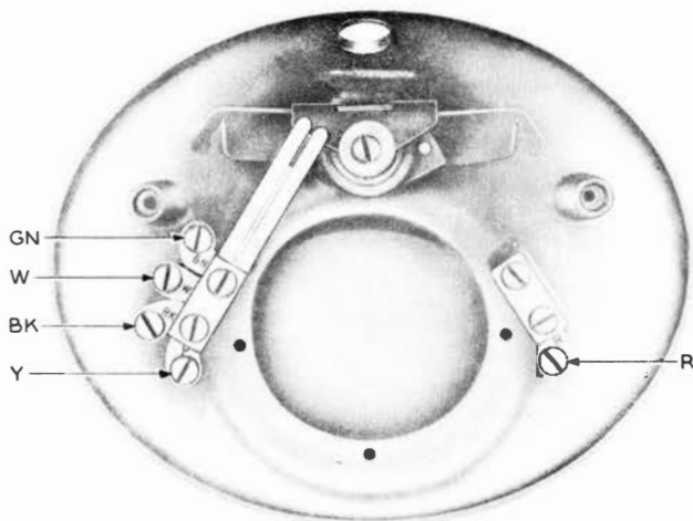
FIG. 5—D1-TYPE HANDSET MOUNTING
