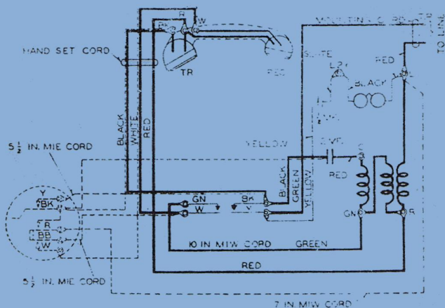
Fig. 2—S327A, B, C and D Type Telephone Sets—Connections
