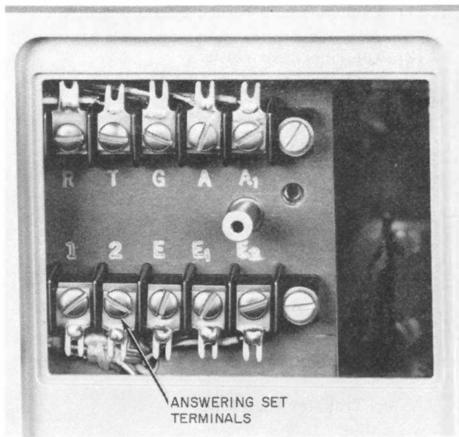
Fig. 28—KS-19245, List 1 (MD) Telephone Answering Set—Terminal Board
