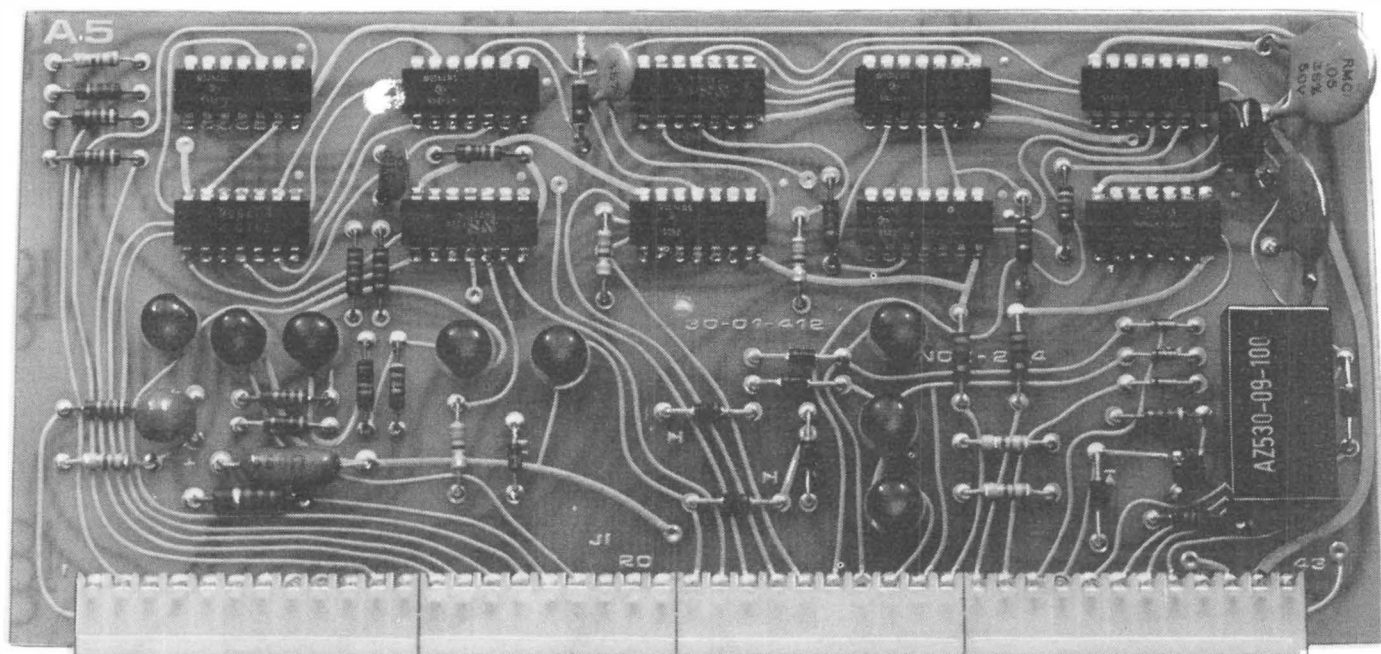
Fig. 15—KS-19245, List 16 Deck Control Board
