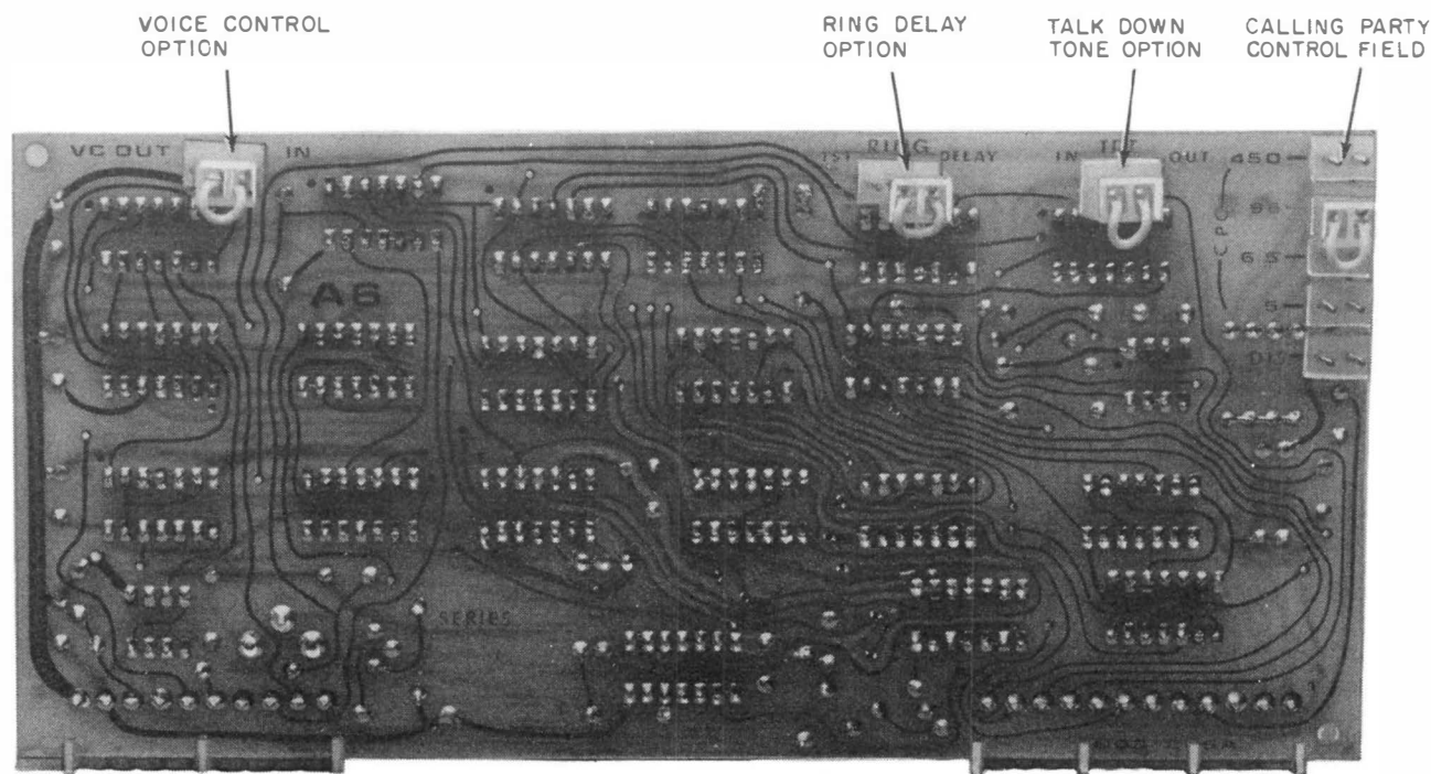
Fig. 16—KS-19245, List 17 Logic Board
