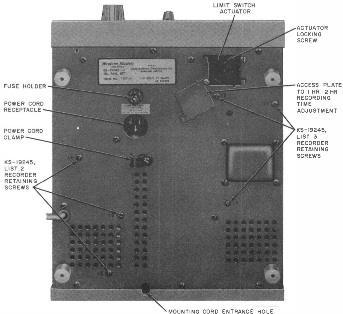
Fig. 21—KS-19245, List 1 (MD) Telephone Answering Set—Bottom View
