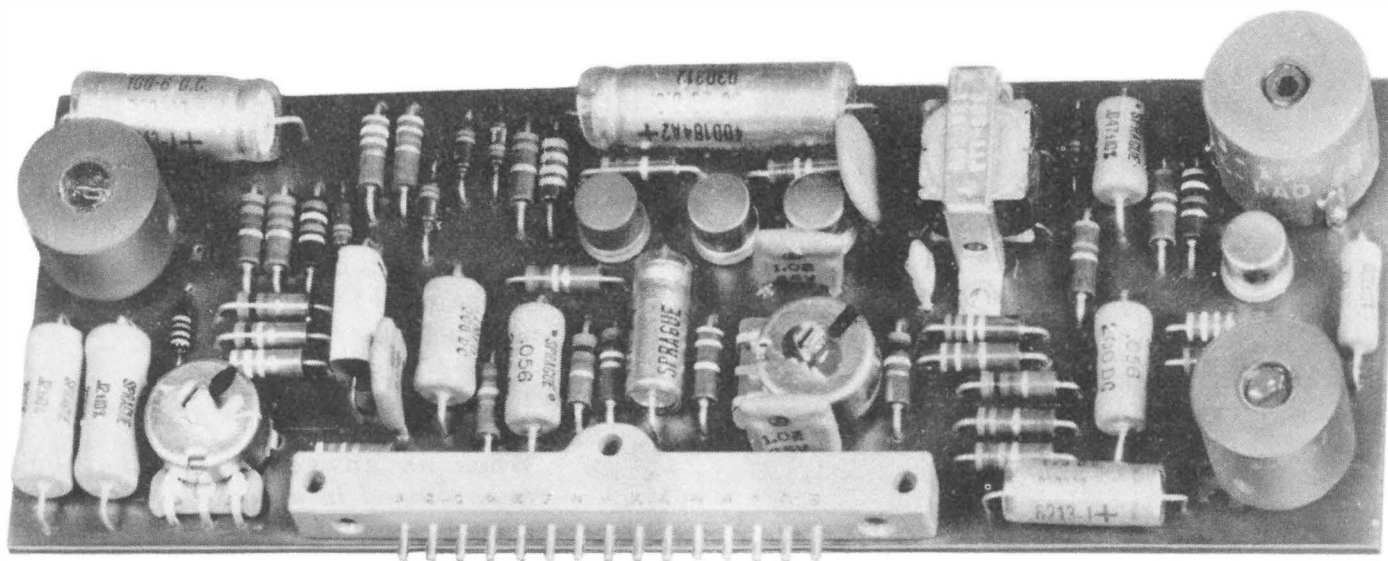
Fig. 8—KS-19245, List 4 Amplifier
