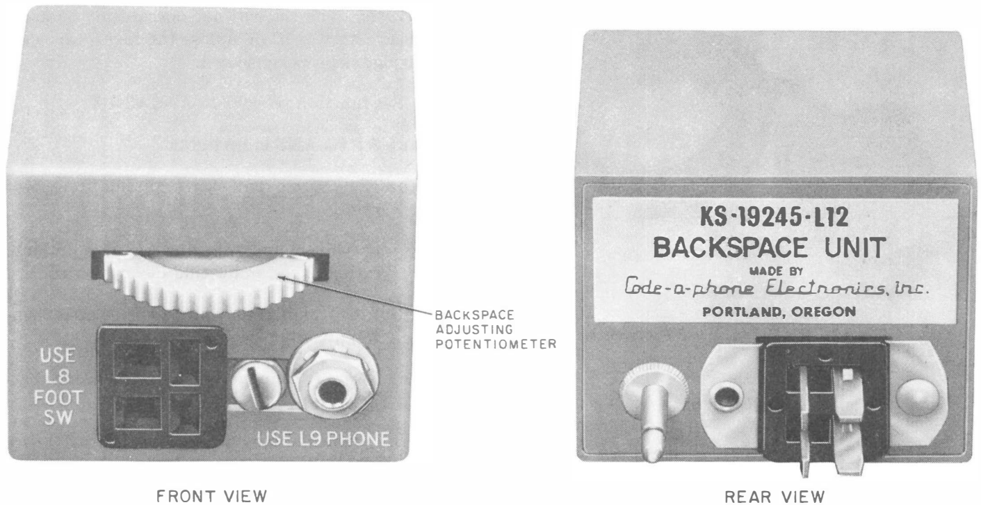
Fig. 19—KS-19245, List 12 Backspace Unit
