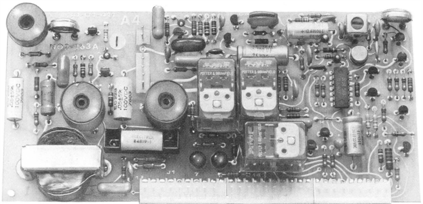
Fig. 14—KS-19245, List 15 Amplifier Board
