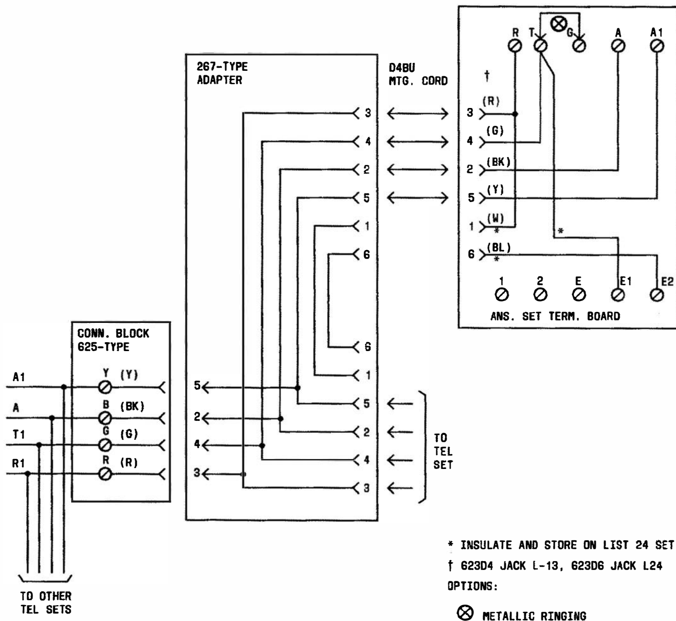
Fig. 36—KS-19245, Lists 13 (MD), 24 (MD), and 26 Telephone Answering Sets, Connections for Key Telephone Systems (Four Terminal Modular)
