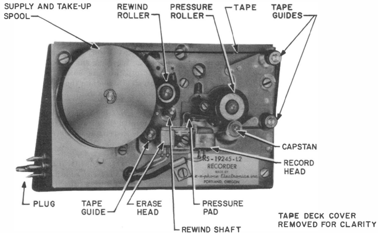
Fig. 4—KS-19245, List 2 Recorder (Reel Side)
