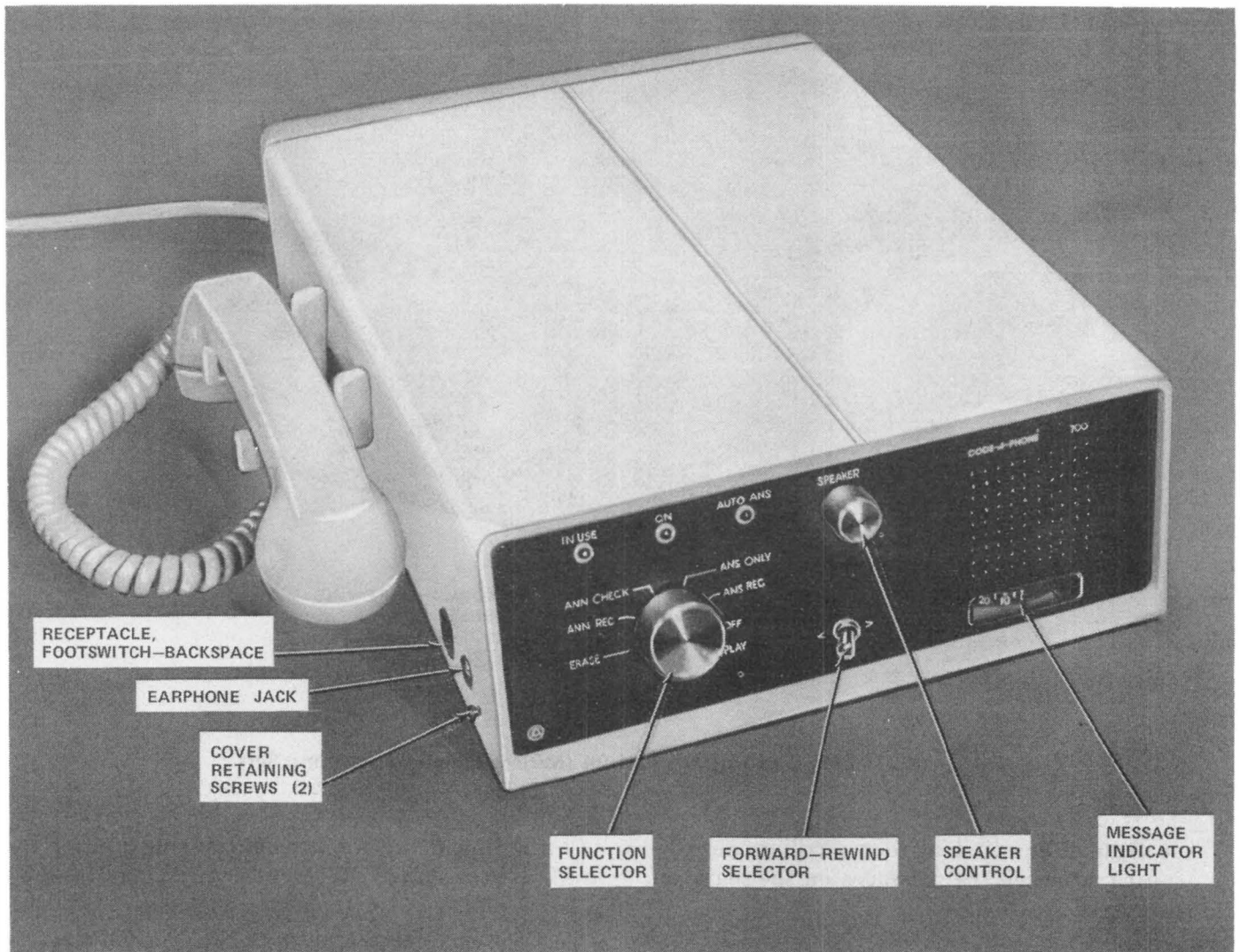
Fig. 3—KS-19245, List 26 Telephone Answering Set
