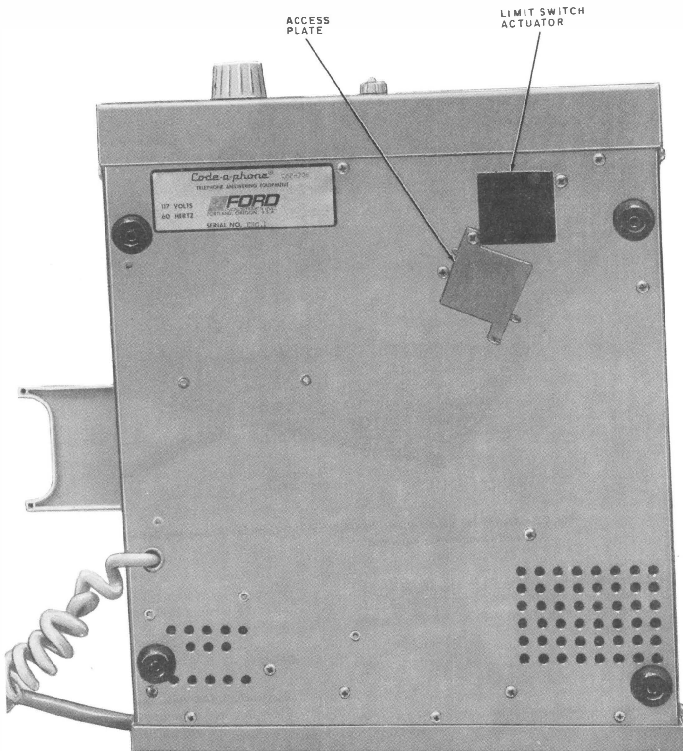
Fig. 23—KS-19245, List 13 (MD) Telephone Answering Set—Bottom View
