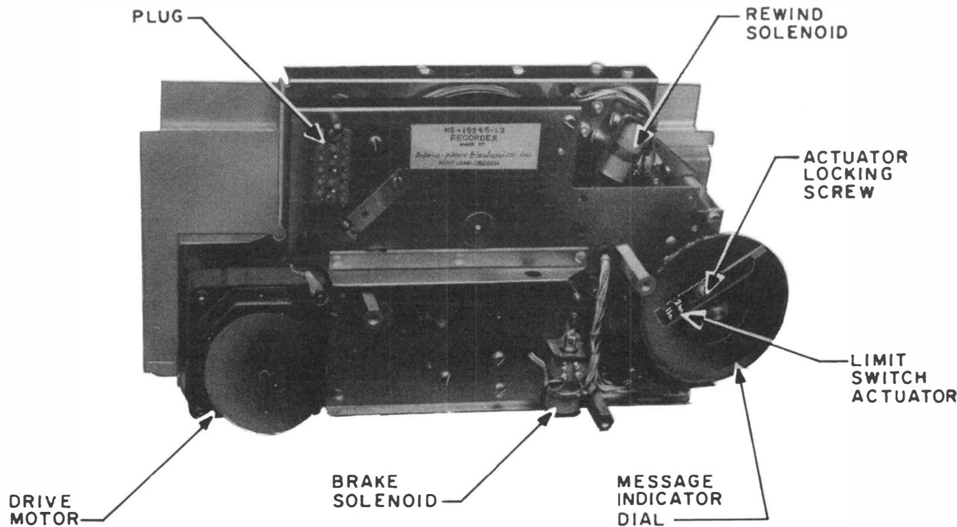
Fig. 7—KS-19245, List 3 Recorder (Motor Side)
