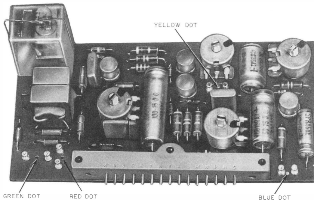
Fig. 9—KS-19245, List 5 Amplifier
