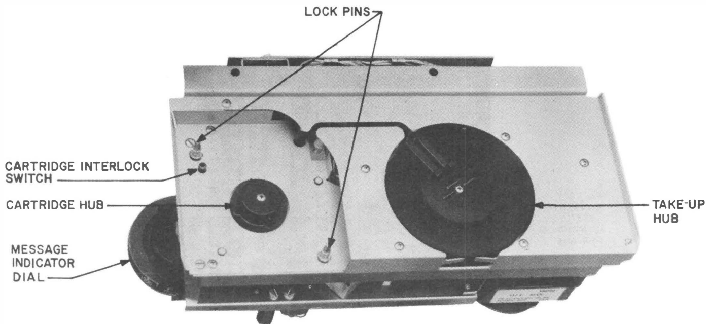
Fig. 6—KS-19245, List 3 Recorder (Reel Side)
