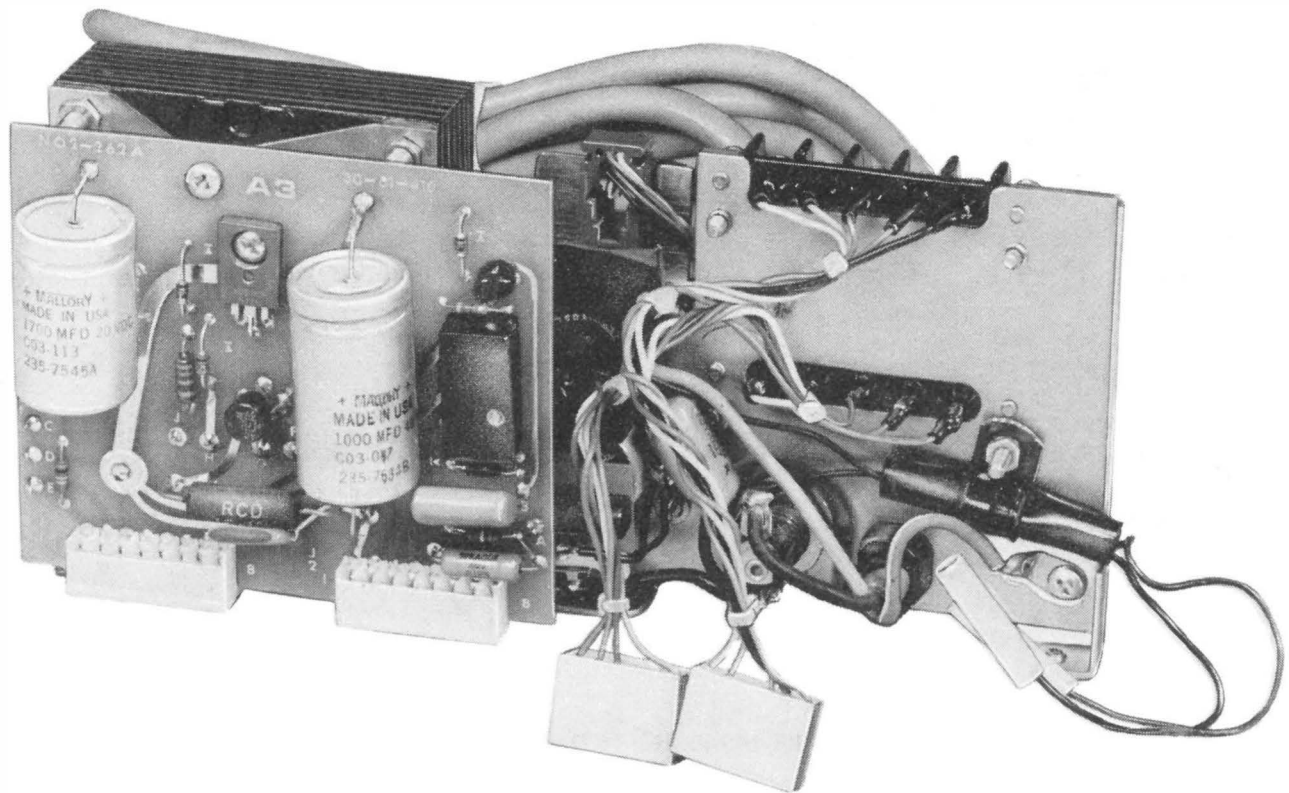
Fig. 13—KS-19245, List 19 Power Supply
