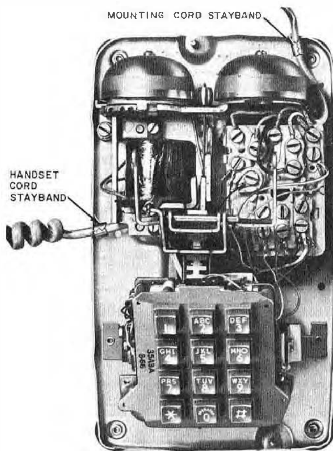
Fig. 5—2500-Type Telephone Set (Interior View)
