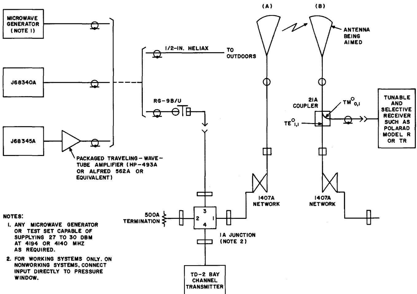
Fig. 5 — Block Diagram of Test Arrangement
