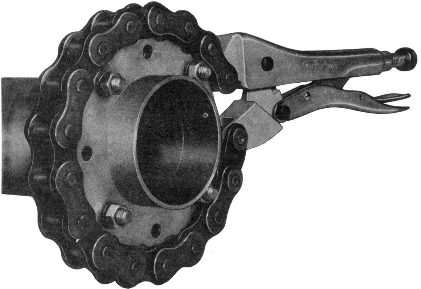
Fig. 9 — AT-8390 Waveguide Alignment Wrench
