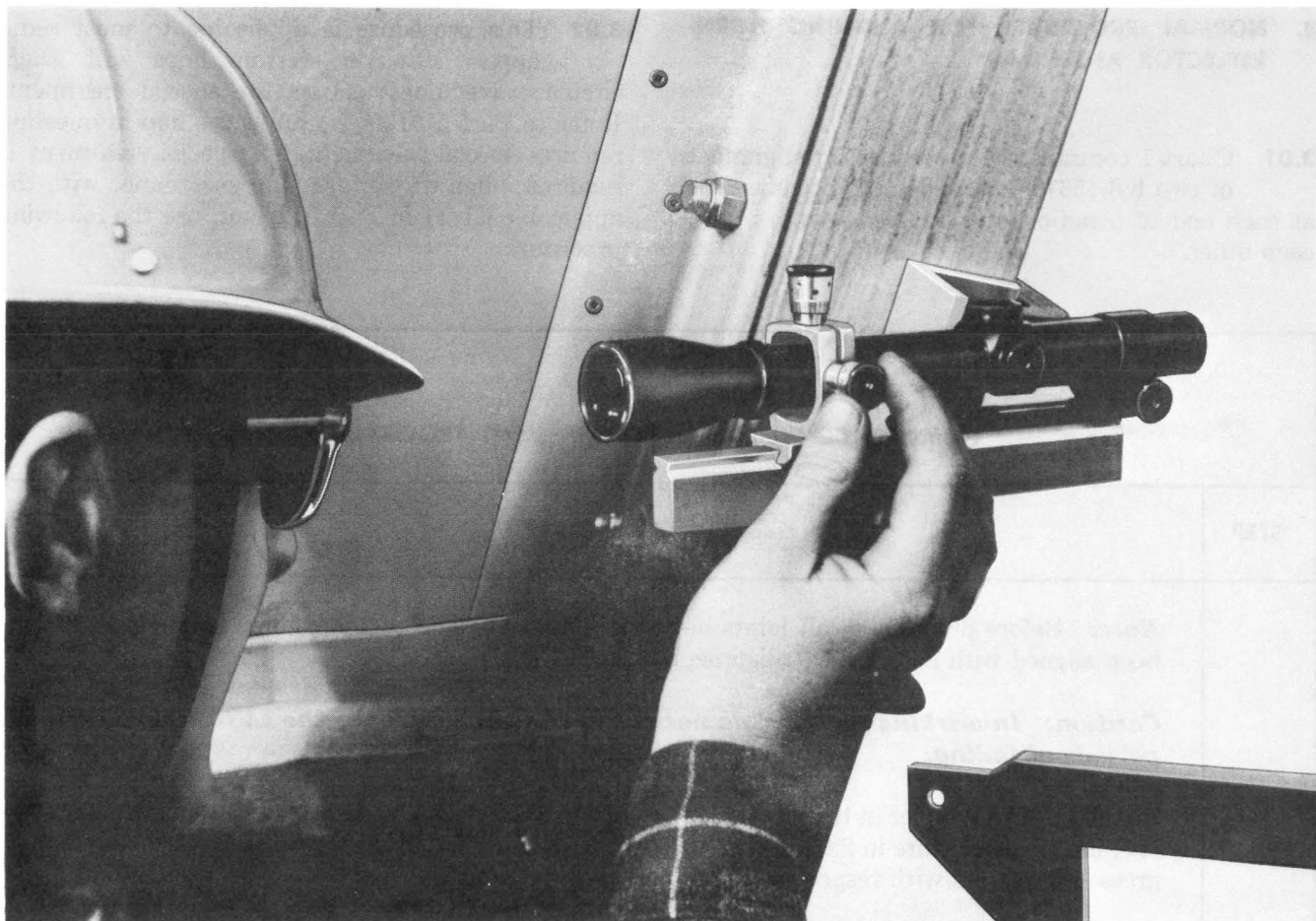
Fig. 10 — KS-20073 Telescope Installed on Antenna
