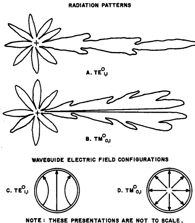
Fig. 3 — Radiation Patterns and Circular-Waveguide Field Configurations for TE_{1,1}^o and TM_{0,1}^o Modes
