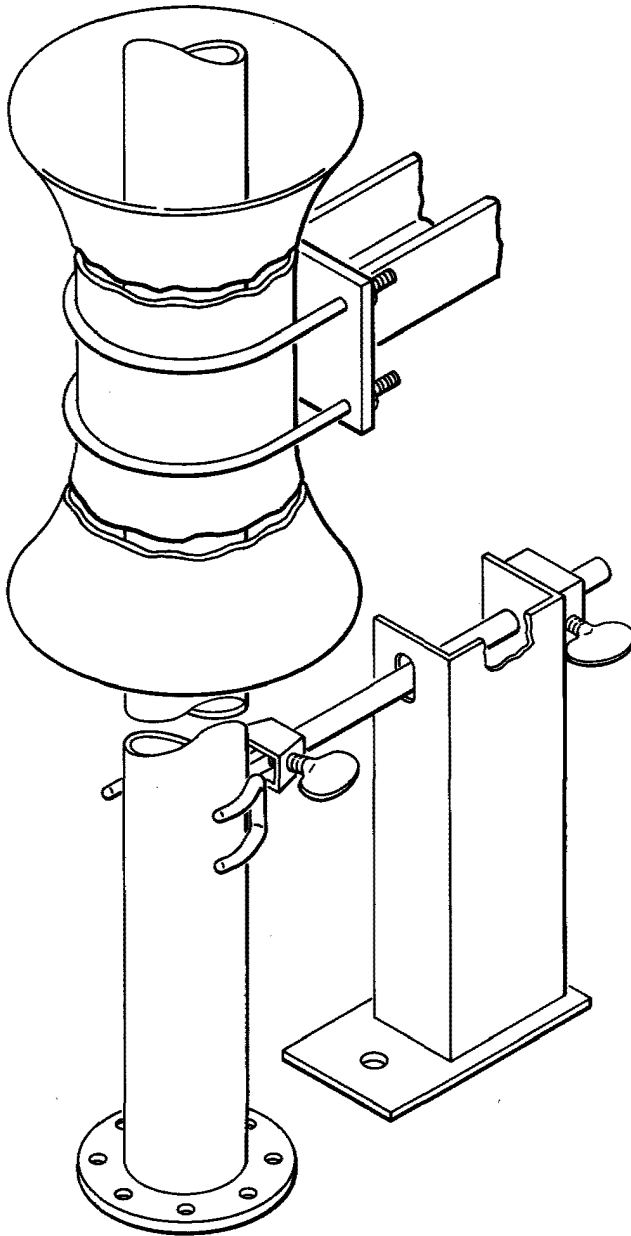
Fig. 7 — AT-8422 B Waveguide Stabilizer
