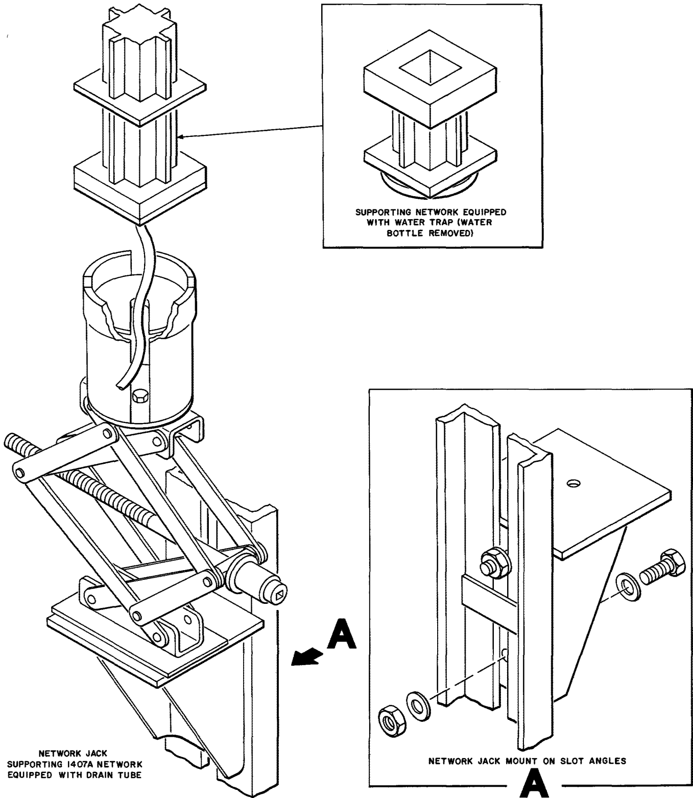
Fig. 8 — AT-8421 B Network Jack
