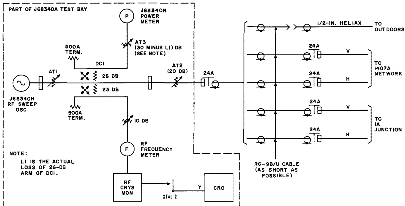
Fig. 6 — Test Connections Using J68340A Test Bay
