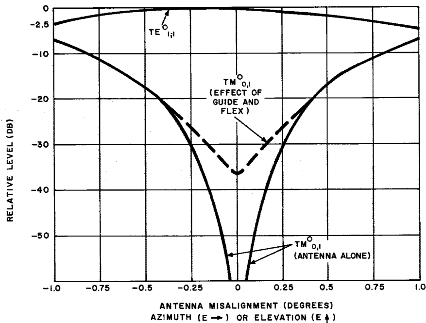
Fig. 2 — TM_{0,1}^{\circ} and TE_{1,1}^{\circ} Levels Versus Antenna Position
