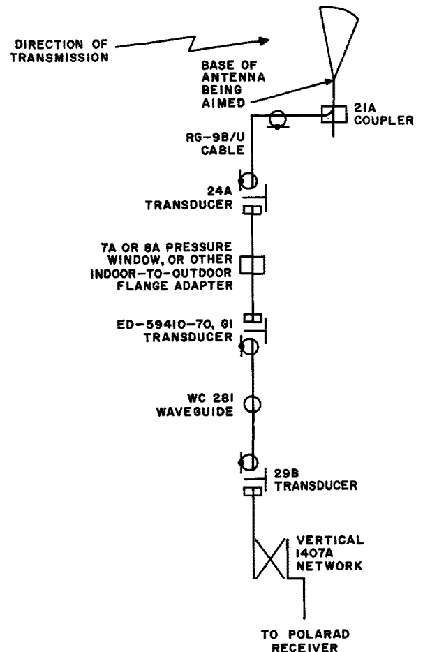
Fig. 14—Test Arrangement for Checking Path Loss (Nonworking Systems Only)
