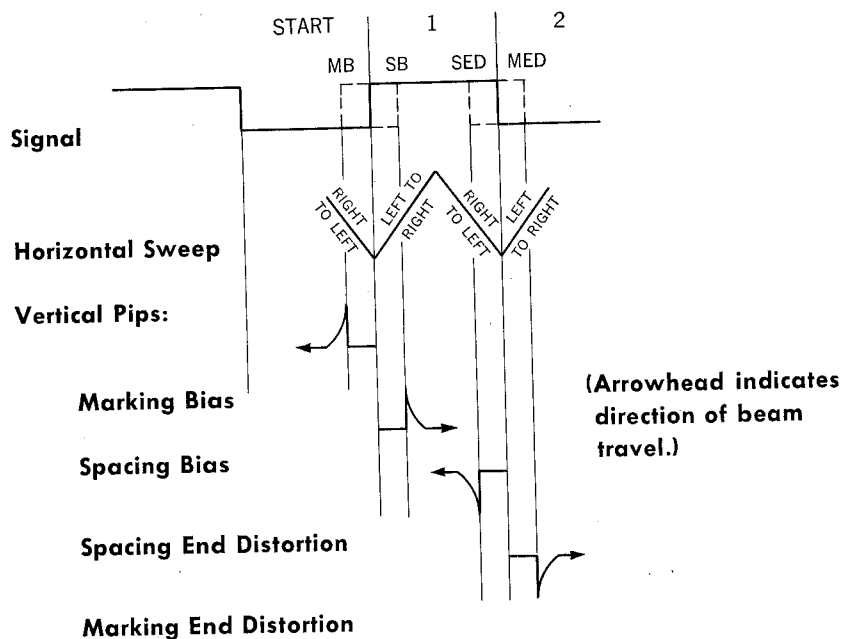
Fig. 4 – Pulses (or Pips) Caused by Different Types of Distortion
