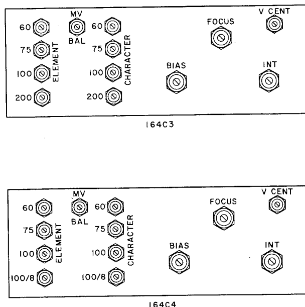
Fig. 6 - Calibration and Adjustment Potentiometers
