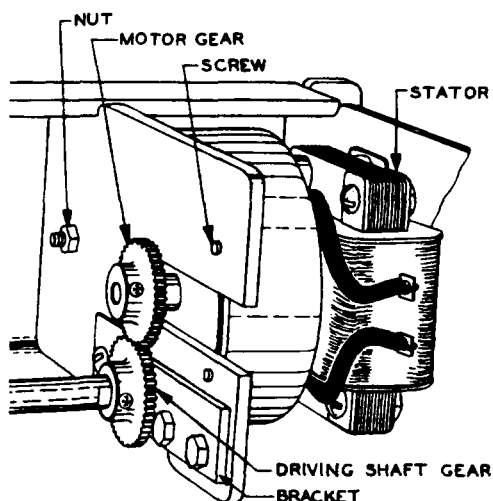
Fig. 1 - 51- and 52-type Drives
