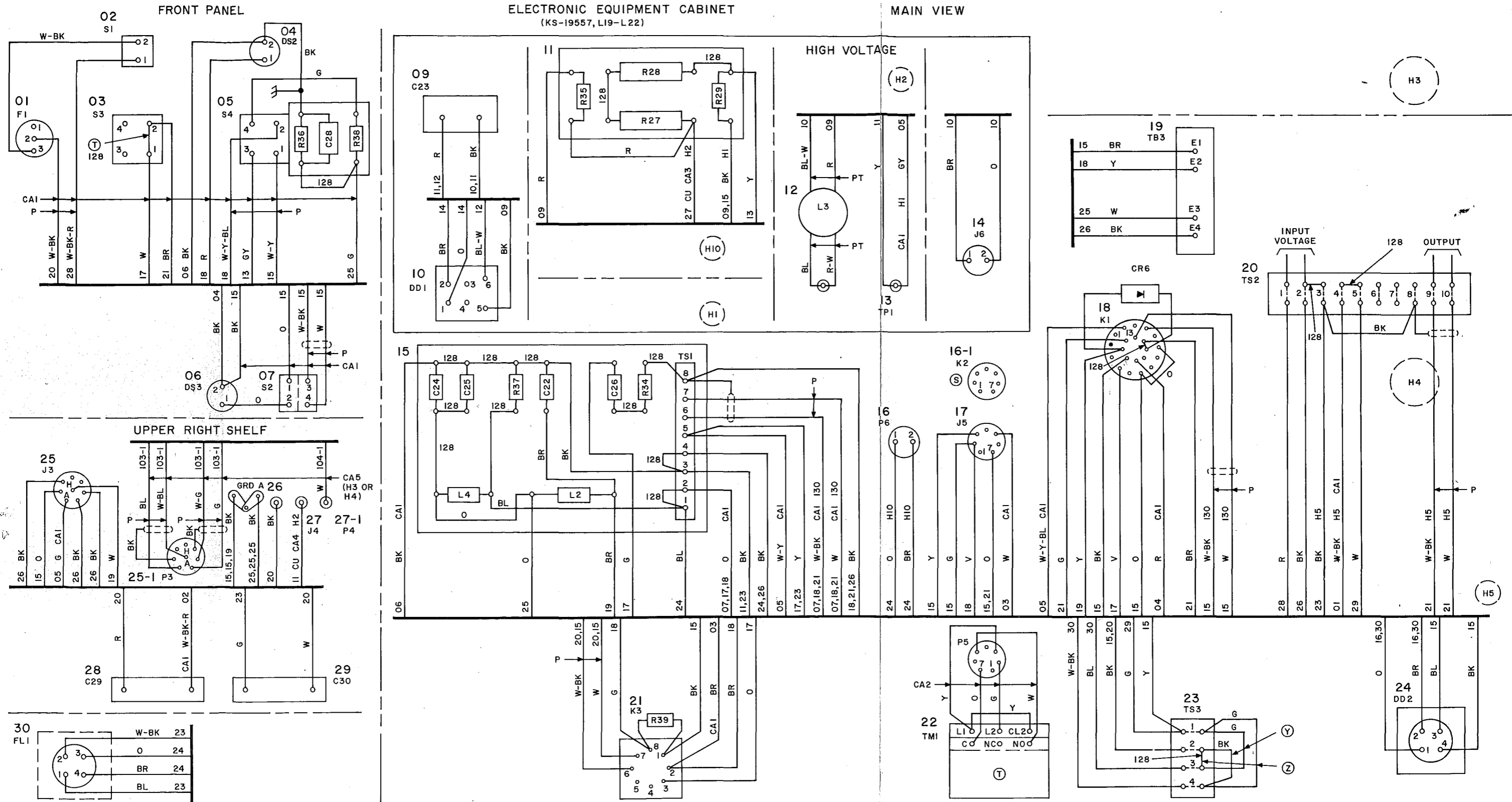
Fig. 10—KS-19557 Detector (Nuclear Blast) Wiring Diagram (Sheet 1 of 2)
