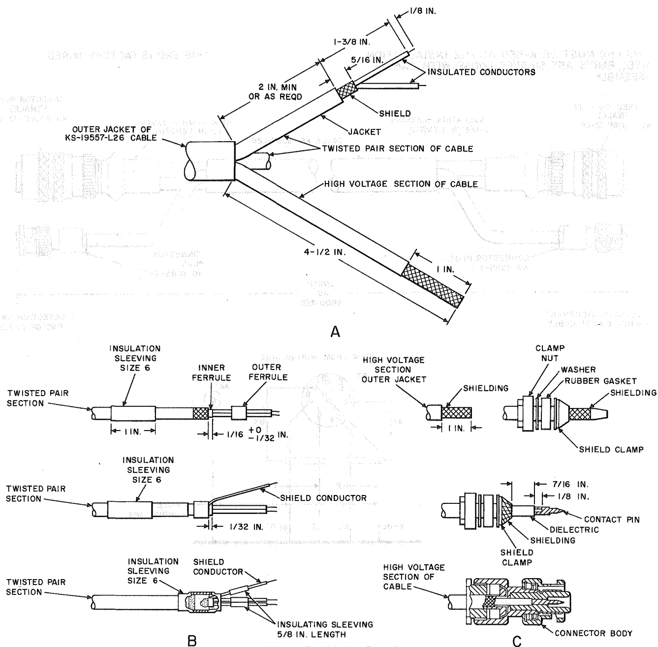
◆ Fig. 8—Connector Termination ◆
