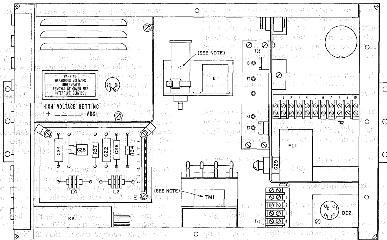
Fig. 5—Electrical Equipment Cabinet—Cover Open
