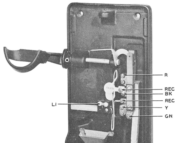
FIG. 4—164C, D—LOWER HOUSING AND BACKPLATE TERMINALS
