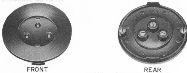
Fig. 3—94A —Plastic plate in all colors, 3-1/64 inches in diameter provided with connecting terminals and chrome plated number card holder group. 94A-3 (BK) is not provided with number card holder group. Replaces 82A. For 300-type indoor telephone sets.
