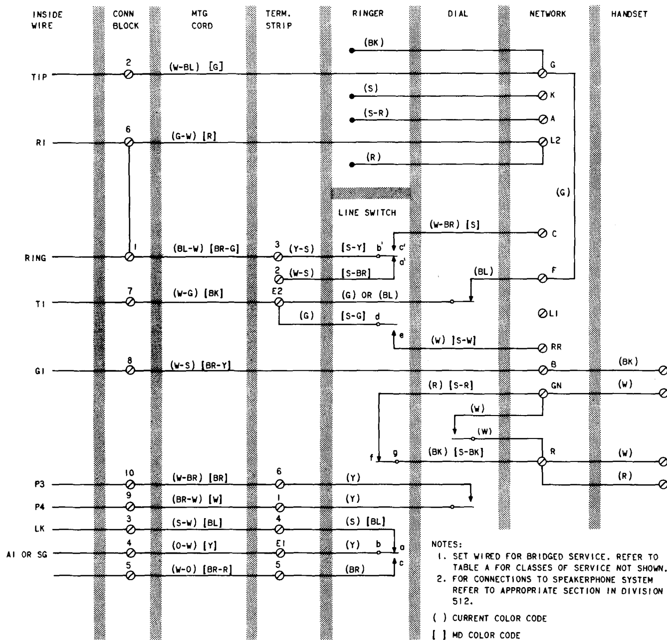
Fig. 1—500R/S Telephone Set, Connections
