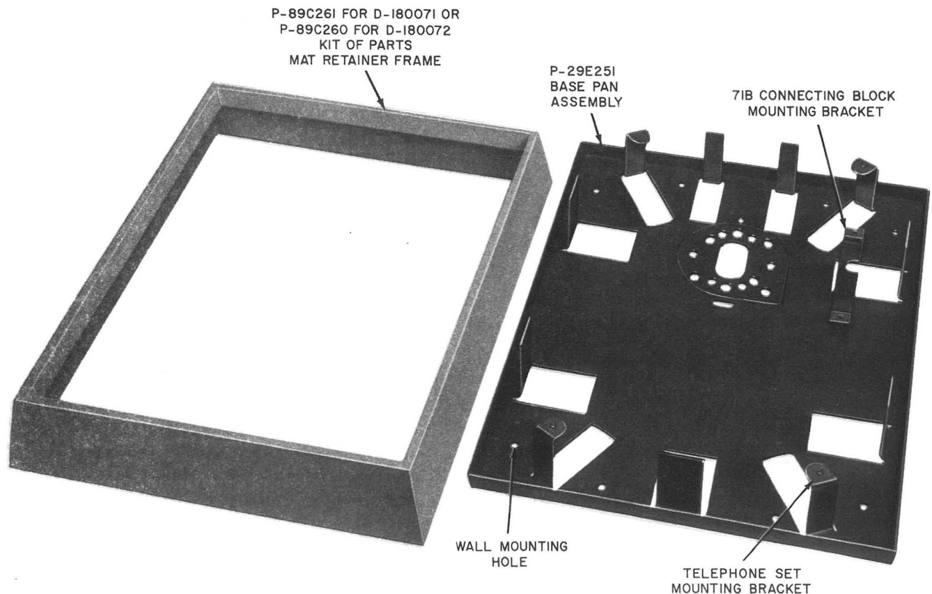
Fig. 1—D-180071 or D-180072 Kit of Parts
