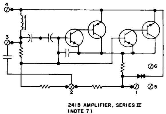
Fig. 5—2563HBM Telephone Set, Connections (Sheet 2 of 2)
