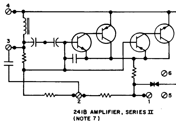
Fig. 4—2563HB (MD) Telephone Set, Connections (Sheet 2 of 2)
