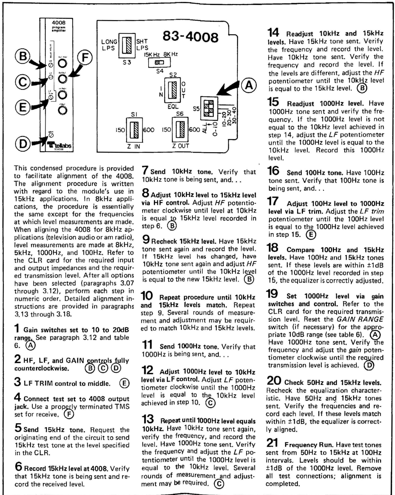
figure 5. Condensed alignment procedure
