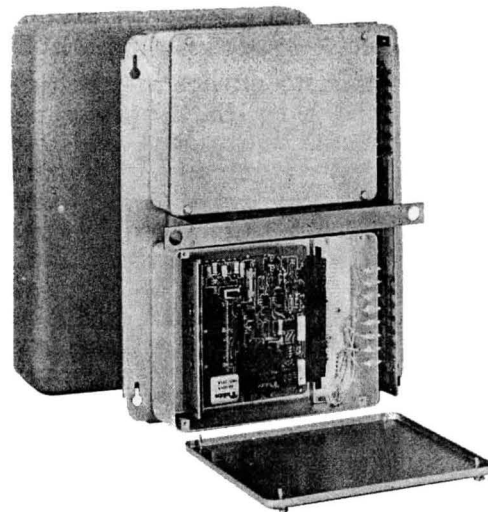
figure 4. 248RF Program Amplifier Assembly
