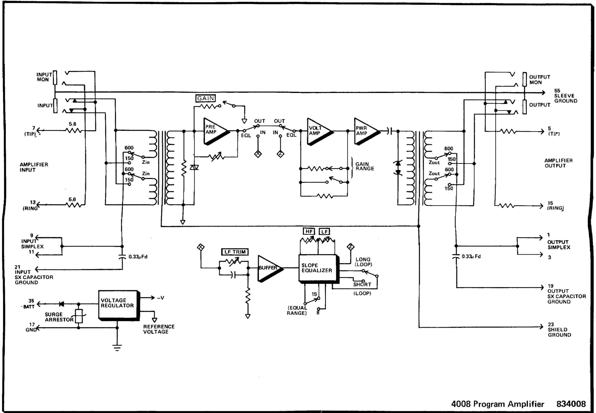
5. Block Diagram
