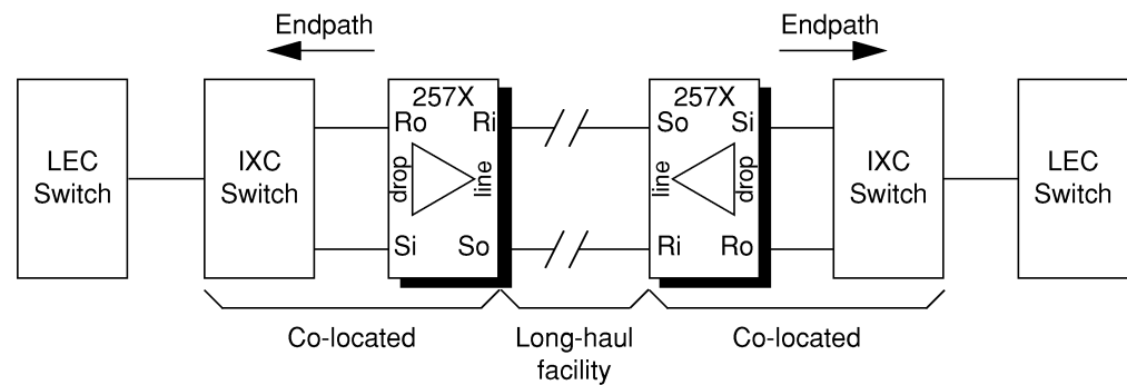
Figure 2-4 Typical Application Using Intermachine Trunk Deployment
