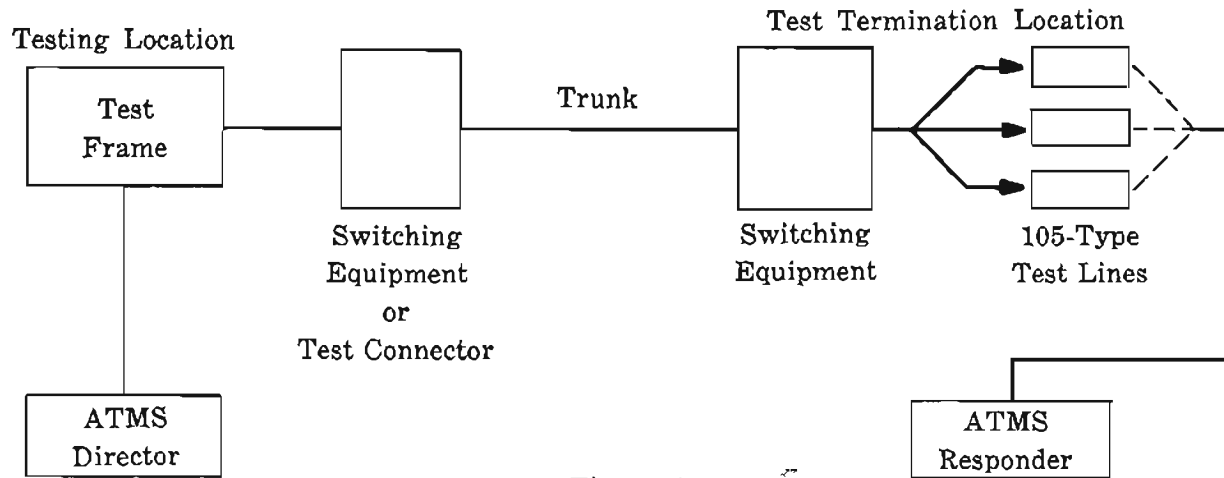
Figure 6 Arrangement for 105-Type Test Line
