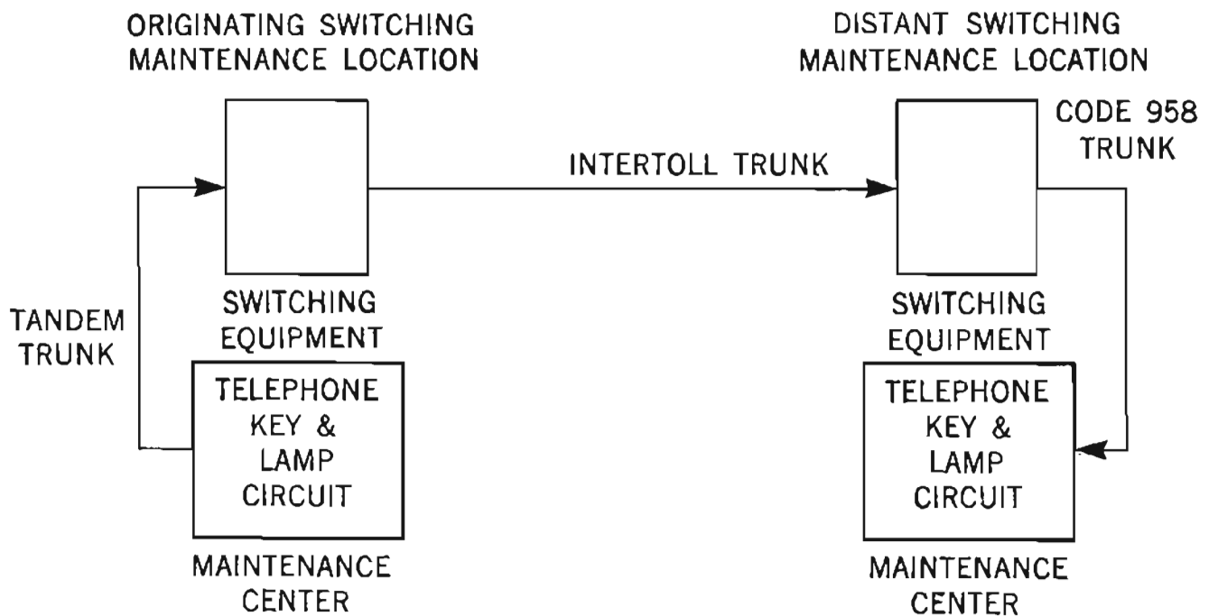
Figure 9 Arrangement for Code 958 Communicating Trunk
