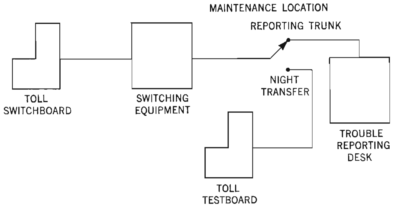
Figure 8 Arrangement for Operator Trouble Reporting Using Code 161
