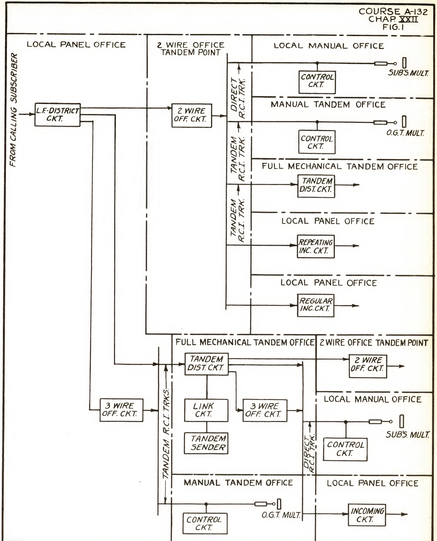
CALLS COMPLETED OVER TANDEM TRUNKS THRU MANUAL AND FULL MECHANICAL TANDEM OFFICES AND THRU TWO WIRE OFFICE TANDEM POINT FIG. I
