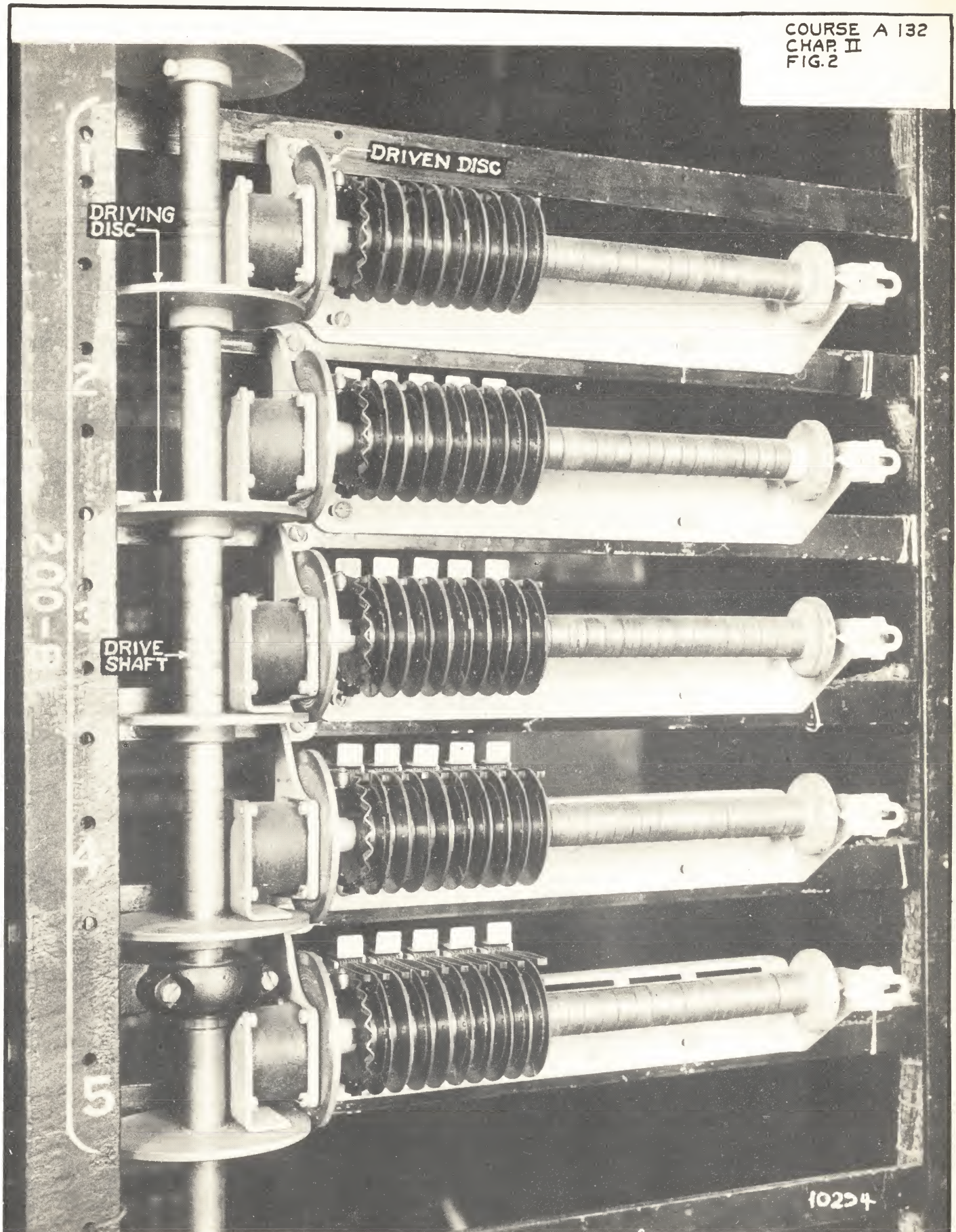
POWER DRIVEN SEQUENCE SWITCHES FIG. 2
