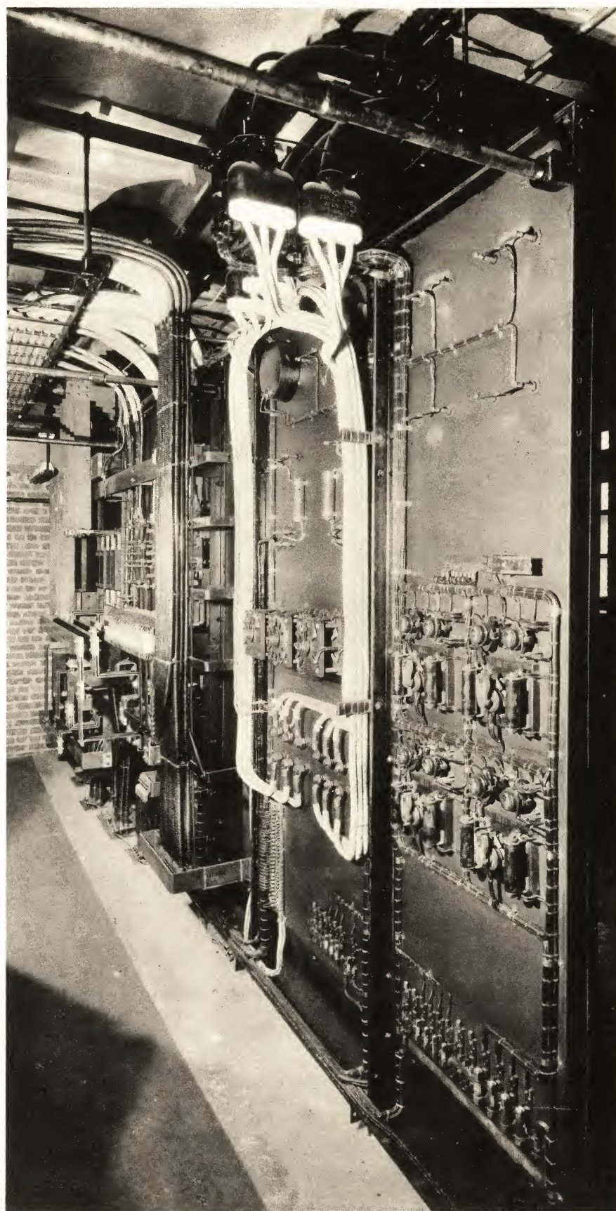
MAIN CONTROL AND BATTERY CONTROL BOARDS REAR VIEW FIG. 5
