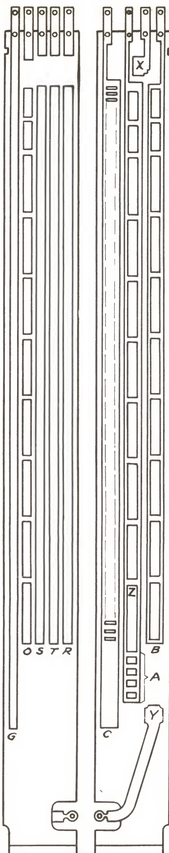
3-D DISTRICT AND OFFICE COMMUTATOR FIG. 6
