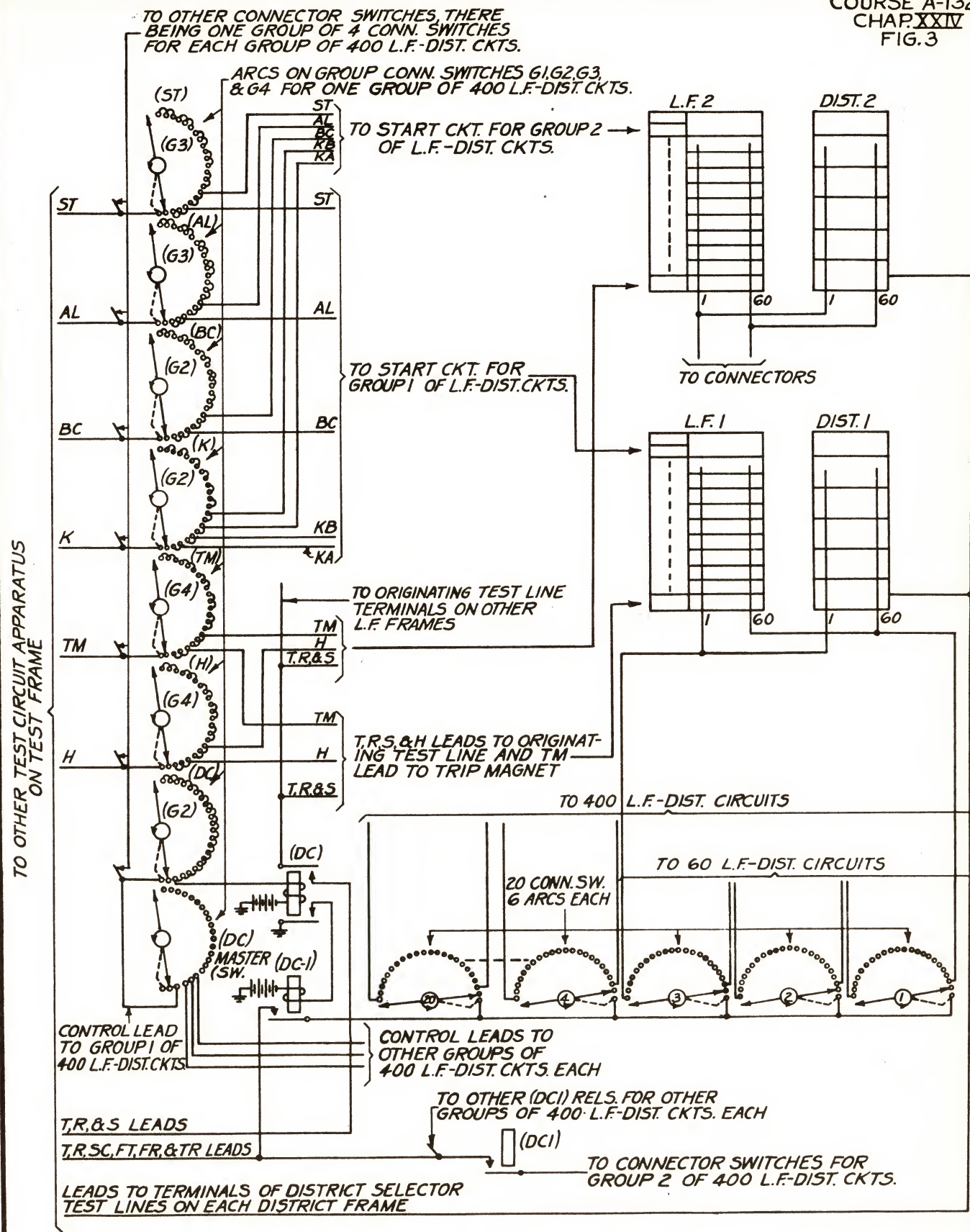
SCHMATIC ARRANGEMENT FOR CONNECTING THE ROUTINE TEST CIRCUIT TO THE LINE FINDER-DISTRICT CIRCUITS FIG. 3
