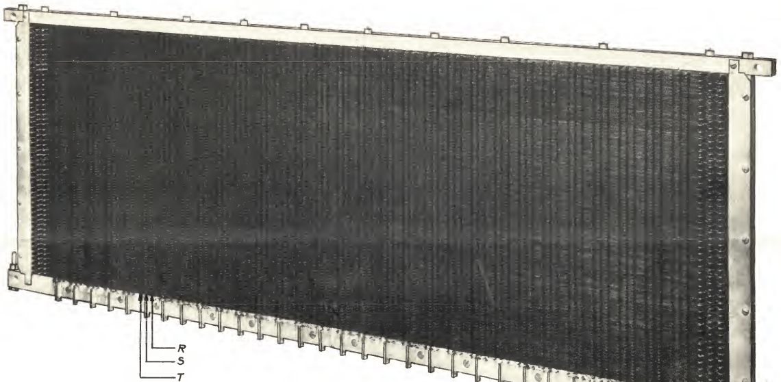
TRUNK HUNTING SELECTOR BANK 100 SETS OF S,R,&T MULTIPLE TERMINAL STRIPS
