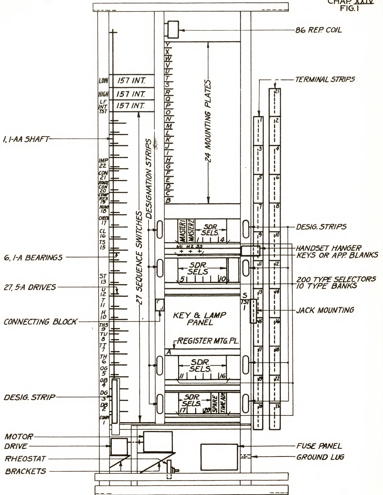
3 DIGIT SUBSCRIBER'S SENDER TEST FRAME FIG. 1
