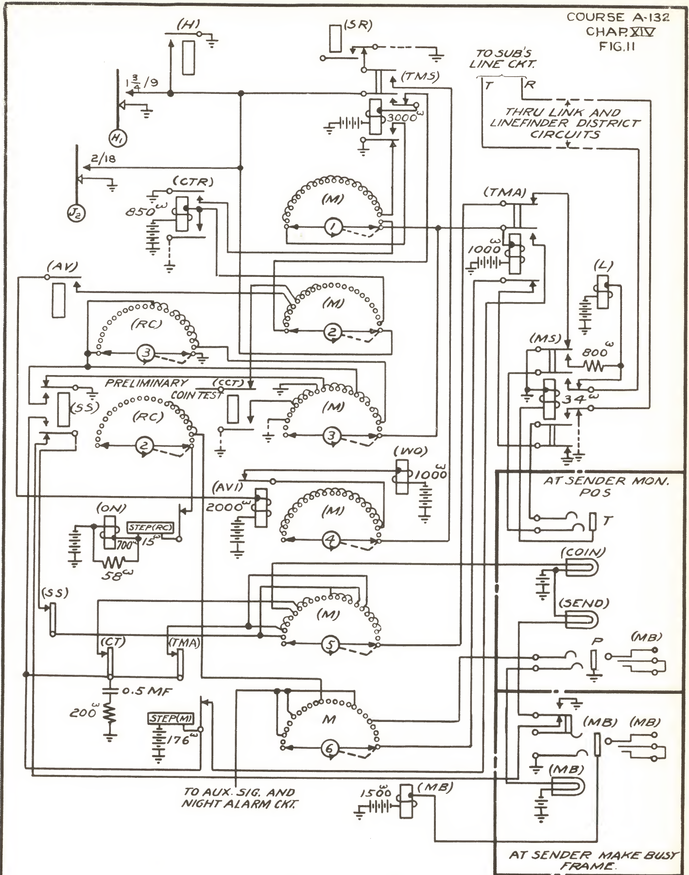
TIME MEASURE CIRCUIT FIG. II
