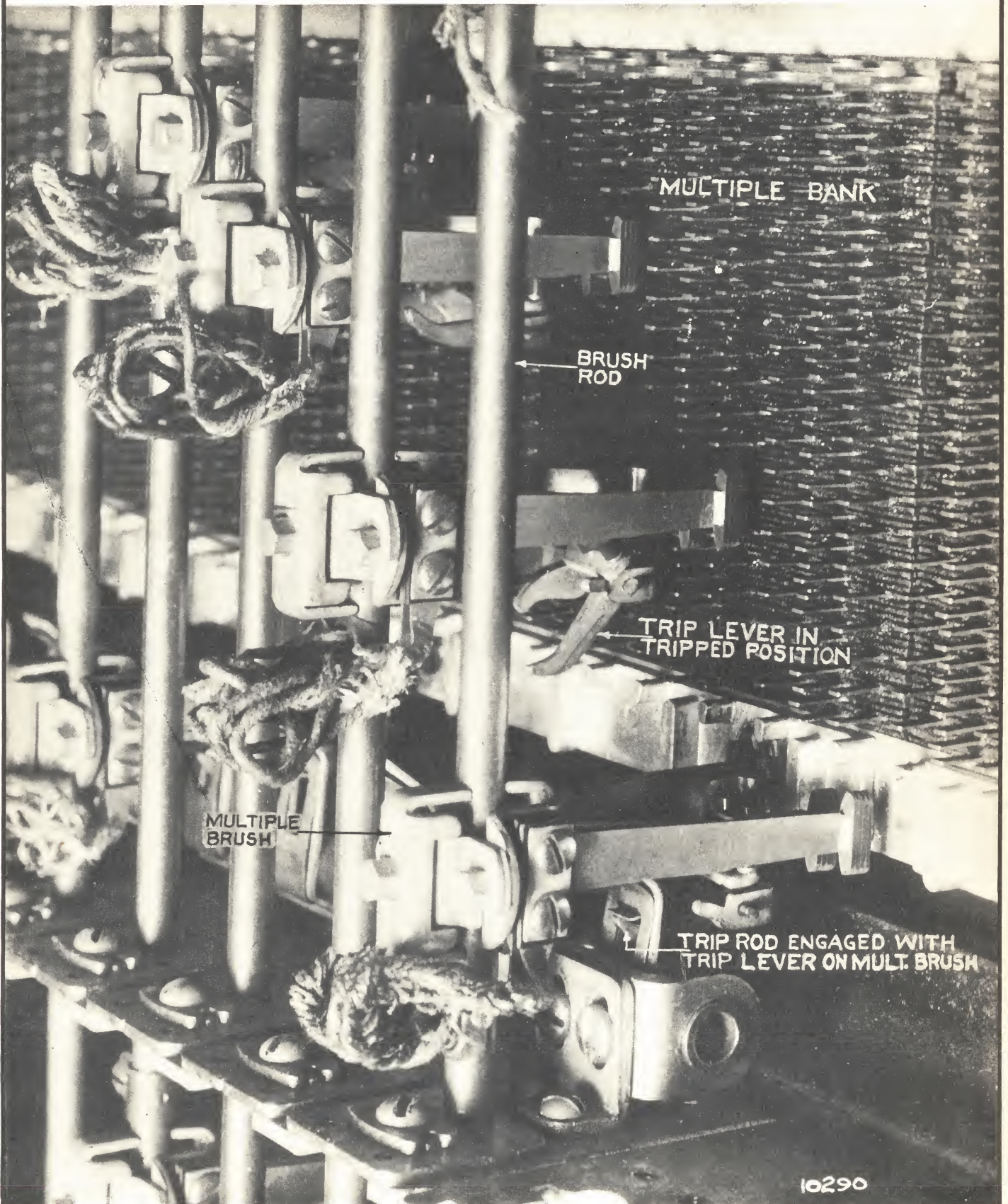
LINE FINDER BRUSH ROD & TRIP MECHANISM FIG. 10
