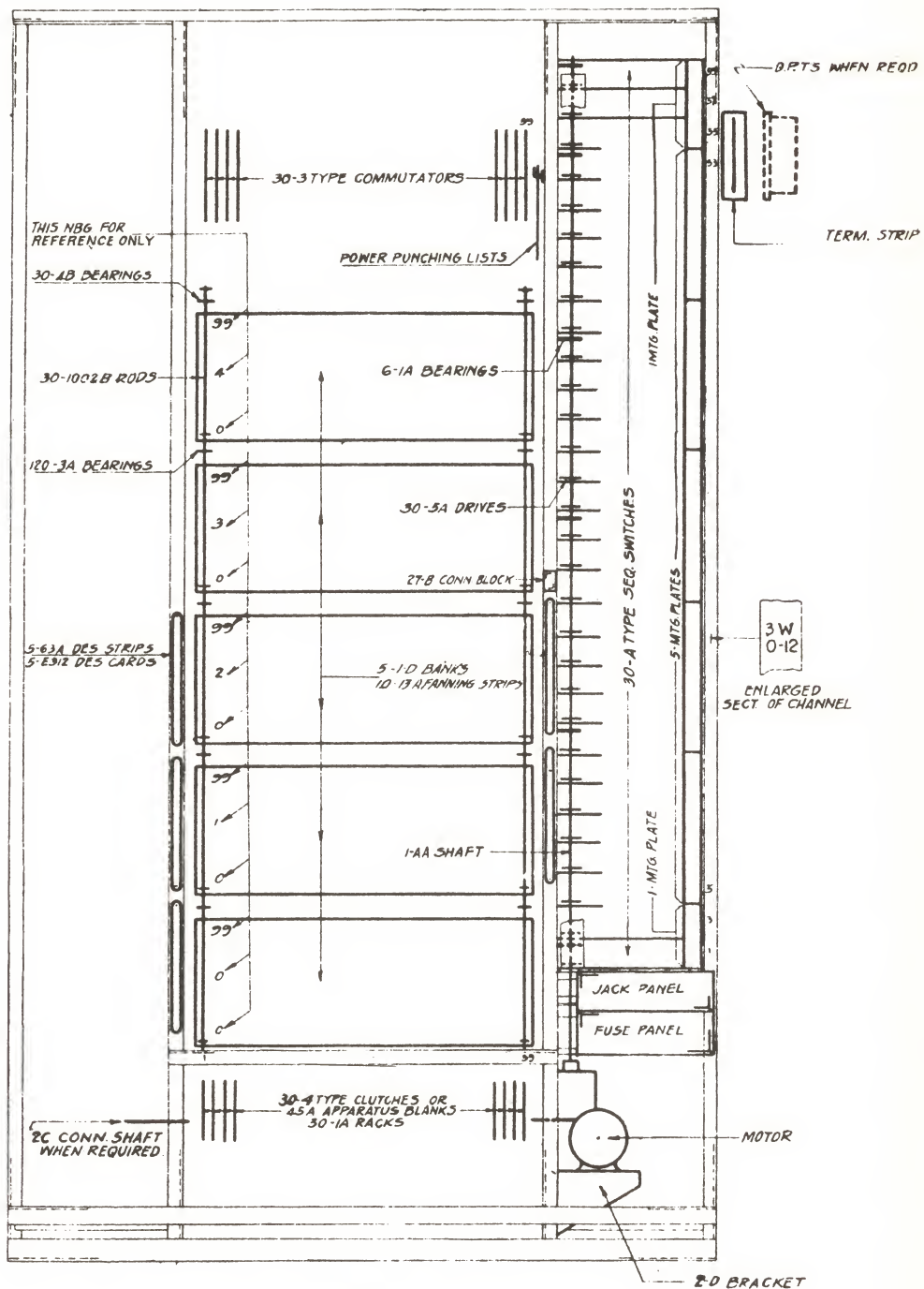
FRONT EQUIPMENT ON REAR SAME AS ABOVE EXCEPT NUMBERING TO BE 2, 4, 6 TO 60
