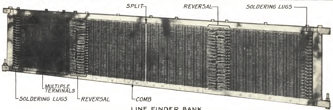
LINE FINDER BANK 40 SETS OF S,R,H,&T MULTIPLE TERMINAL STRIPS
