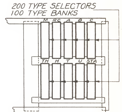
SELECTOR EQUIPMENT ON SENDER UNIT SKETCH B
