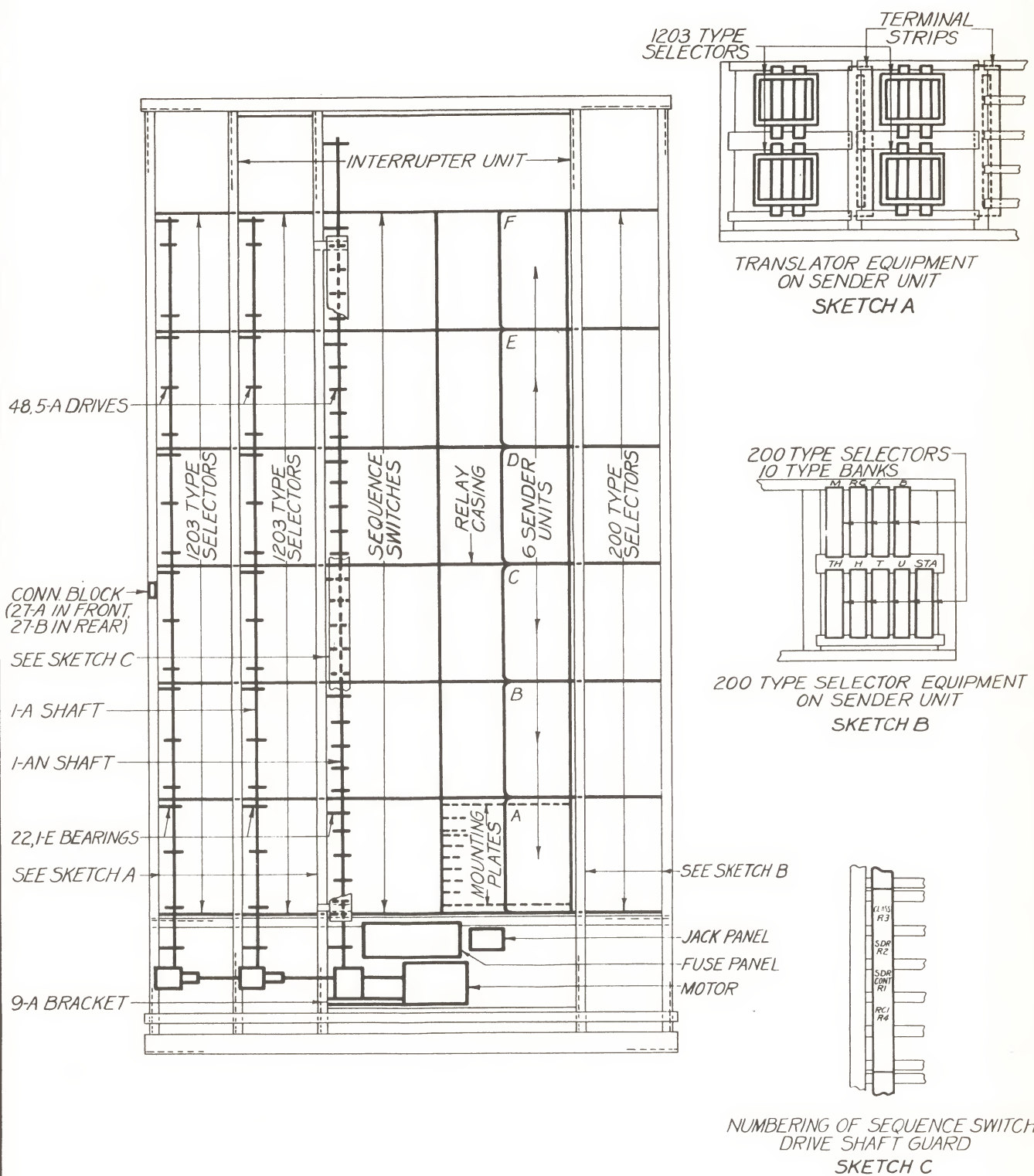
SUBSCRIBERS SENDER FRAME 2 DIGIT-UNIT TYPE WITH 88 POINT TRANSLATOR FIG. 2
