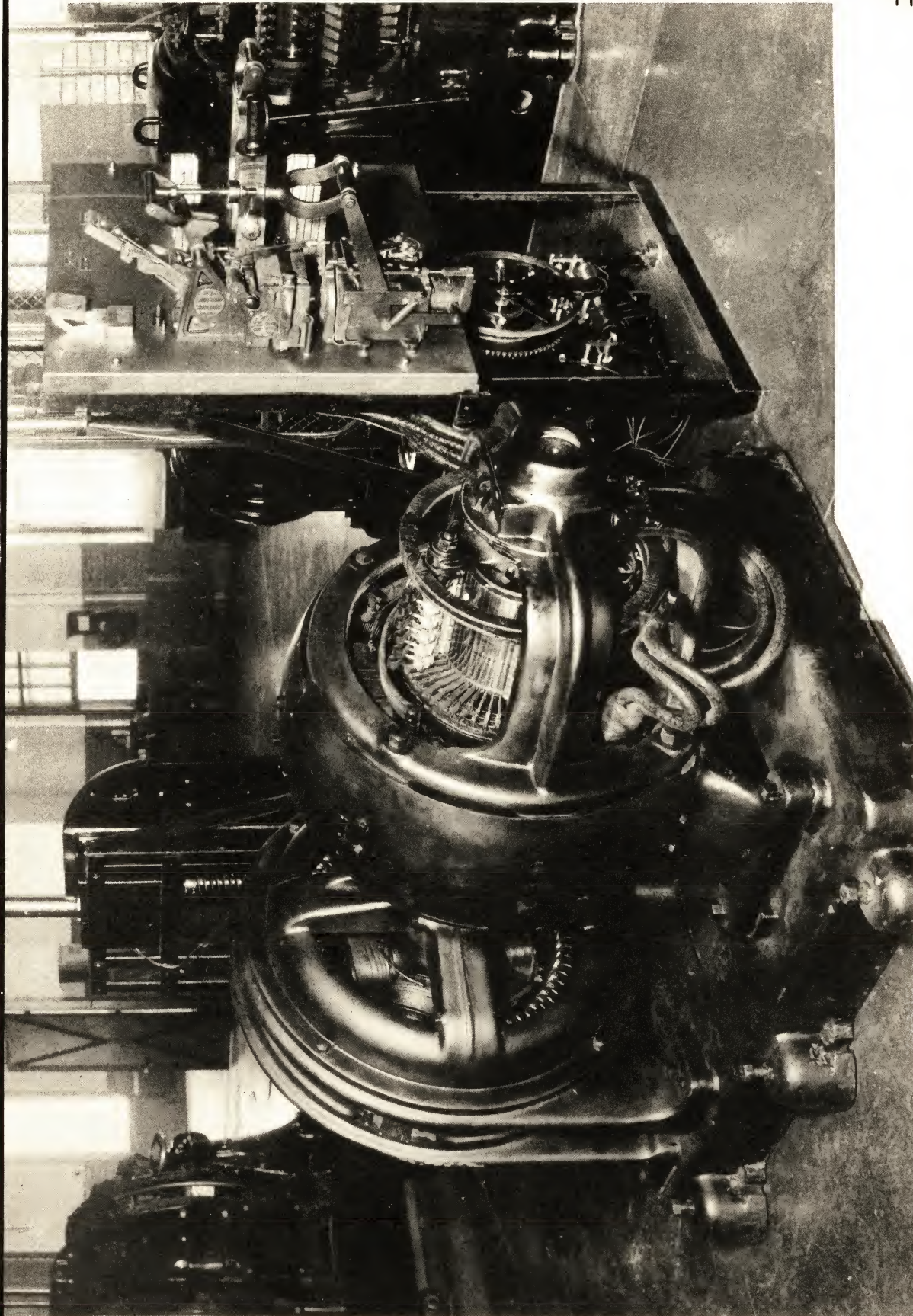
CHARGING MOTOR-GENERATOR SET COMMERCIAL TYPE GENERATOR--SYNCHRONOUS MOTOR FIG. 3
