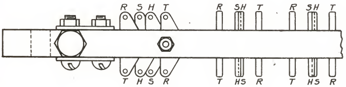
LINE FINDER BANK 40 SETS OF S,R,H,&T MULTIPLE TERMINAL STRIPS
