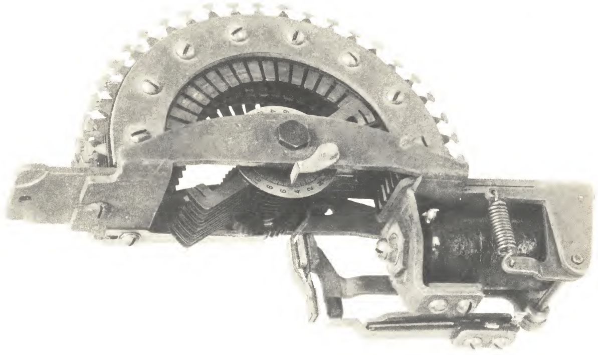
200 TYPE SELECTOR FIG. 1
