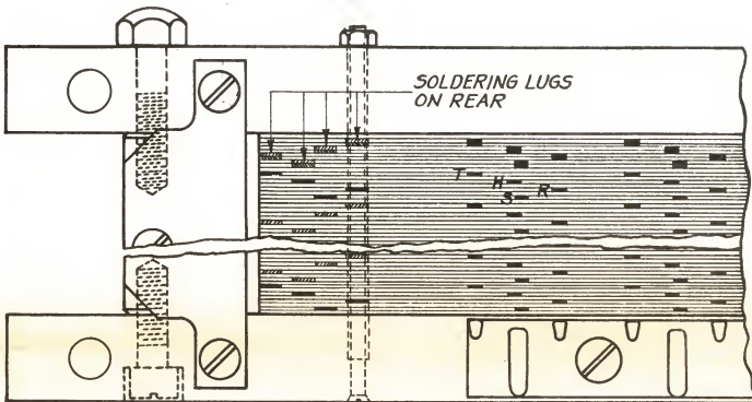
PARTIAL FRONT AND PLAN VIEWS OF LINE FINDER BANK
