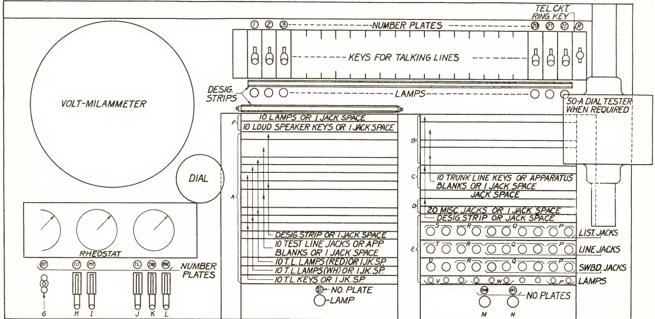
FRONT EQUIPMENT
