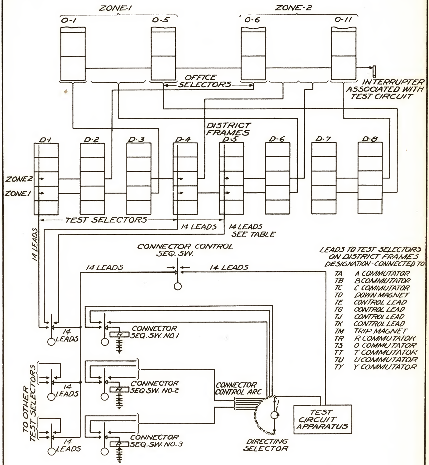
SCHMATIC ARRANGEMENT FOR CONNECTING TEST CIRCUIT TO THE VARIOUS 3 WIRE OFFICE SELECTOR CIRCUITS FIG. 4
