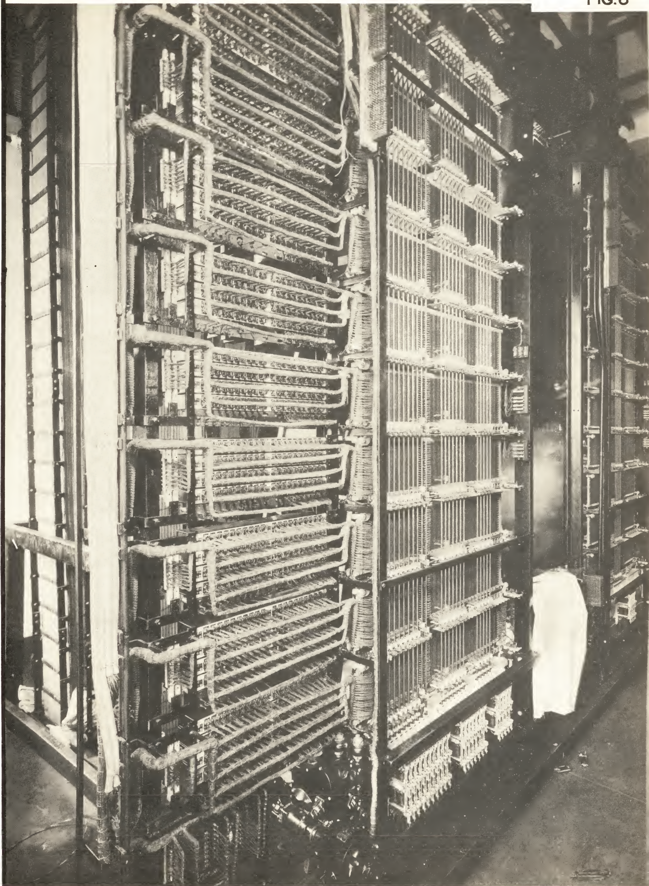
LOCAL CABLE ON LINE FINDER FRAME FIG. 8
