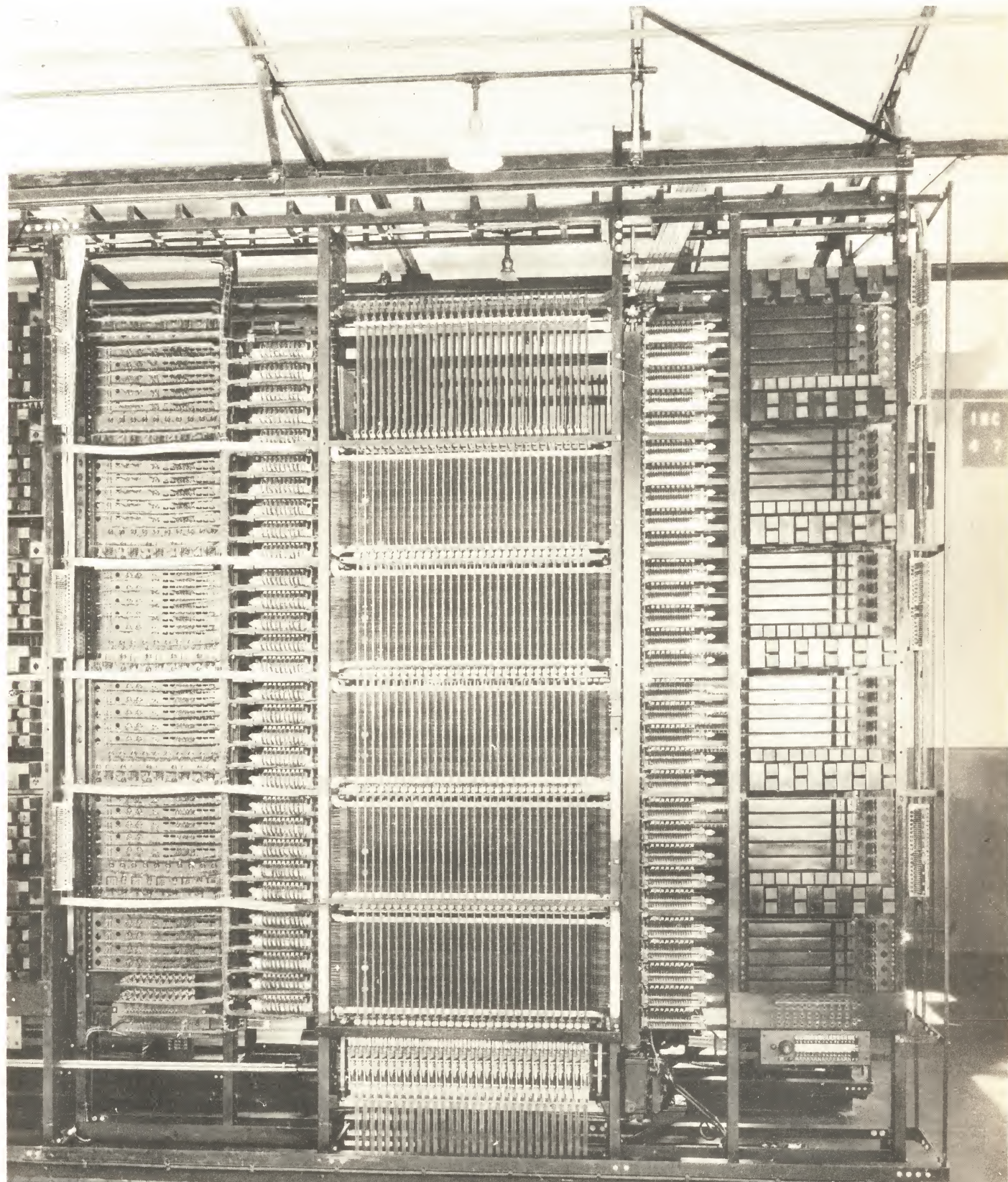
INCOMING SELECTOR FRAME FIG. 2
