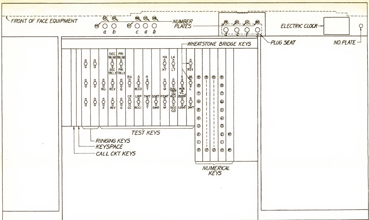
KEYSHELF EQUIPMENT
