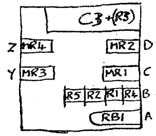
CONDENSER BOX LAYOUT
