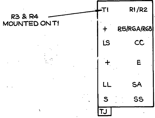
MOUNTING PLATE LAYOUT
