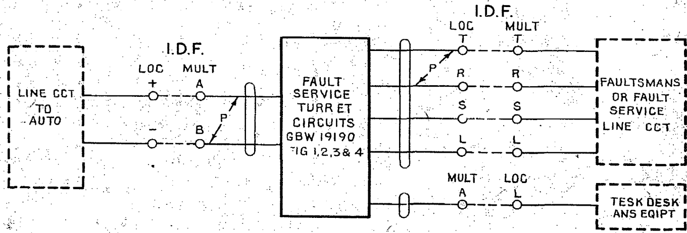
FIG.B. ANS. KEYS & FAULT SERV. SWITCHING KEY.
