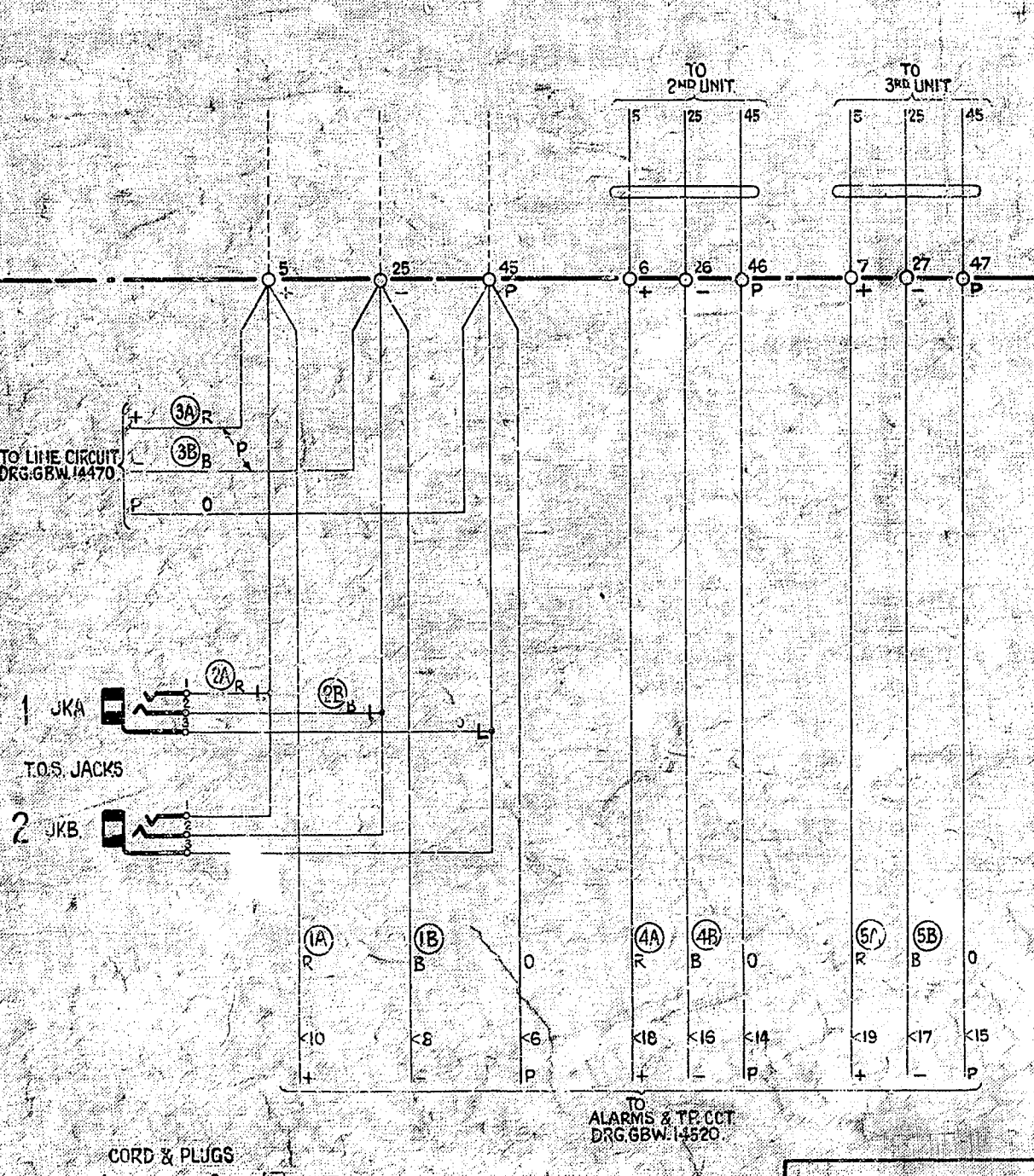
FIG 4A N.U. TONE DISTRIBUTION UNALLOTTED, CEASED OR T.O.S. LINE
