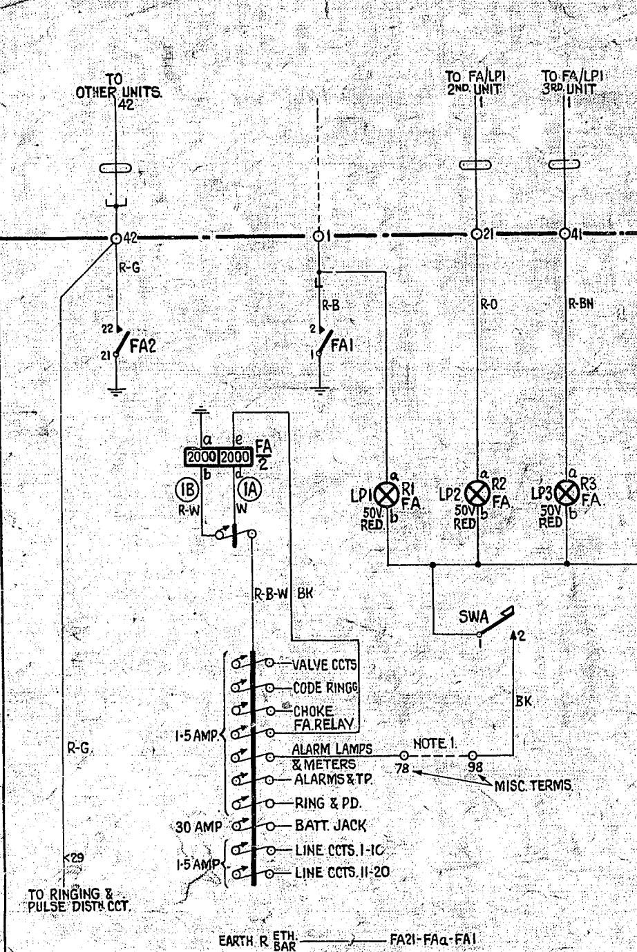
FIG 1A FUSE ALARM
