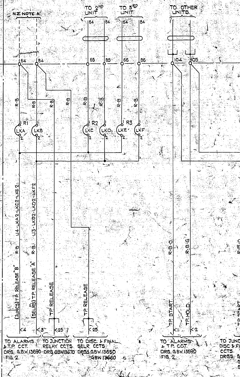
FIG. 10B 1-PER RACK
