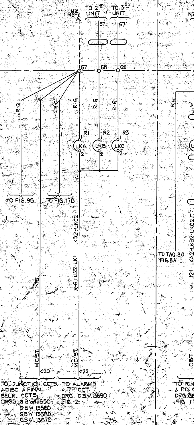
FIG. 11B 1-PER RACK
