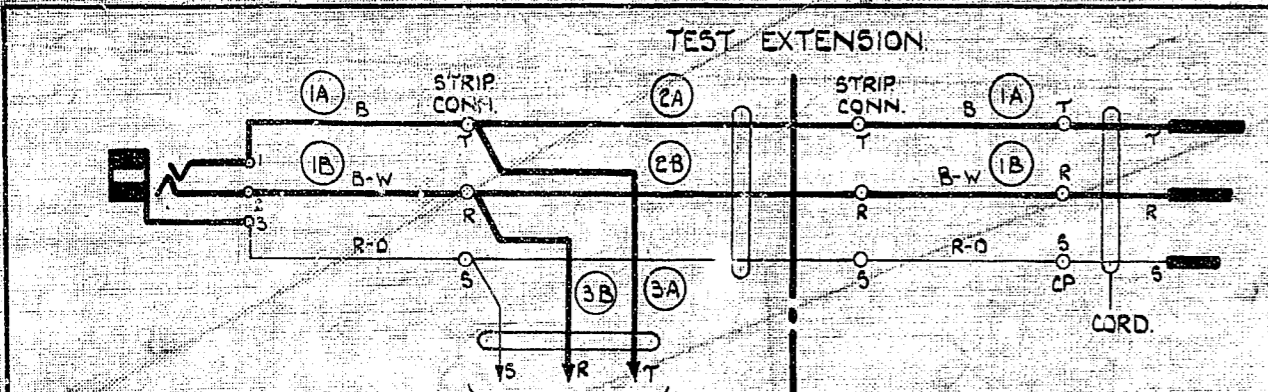
FIG. 1. TEST DESK OR RACK TO OTHER POSNS AS REQUIRED.
