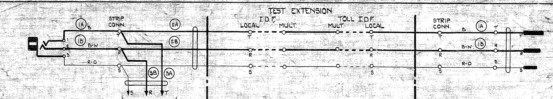
FIG. 4. TEST DESK OR RACK TO OTHER POSNS AS REQUIRED.
