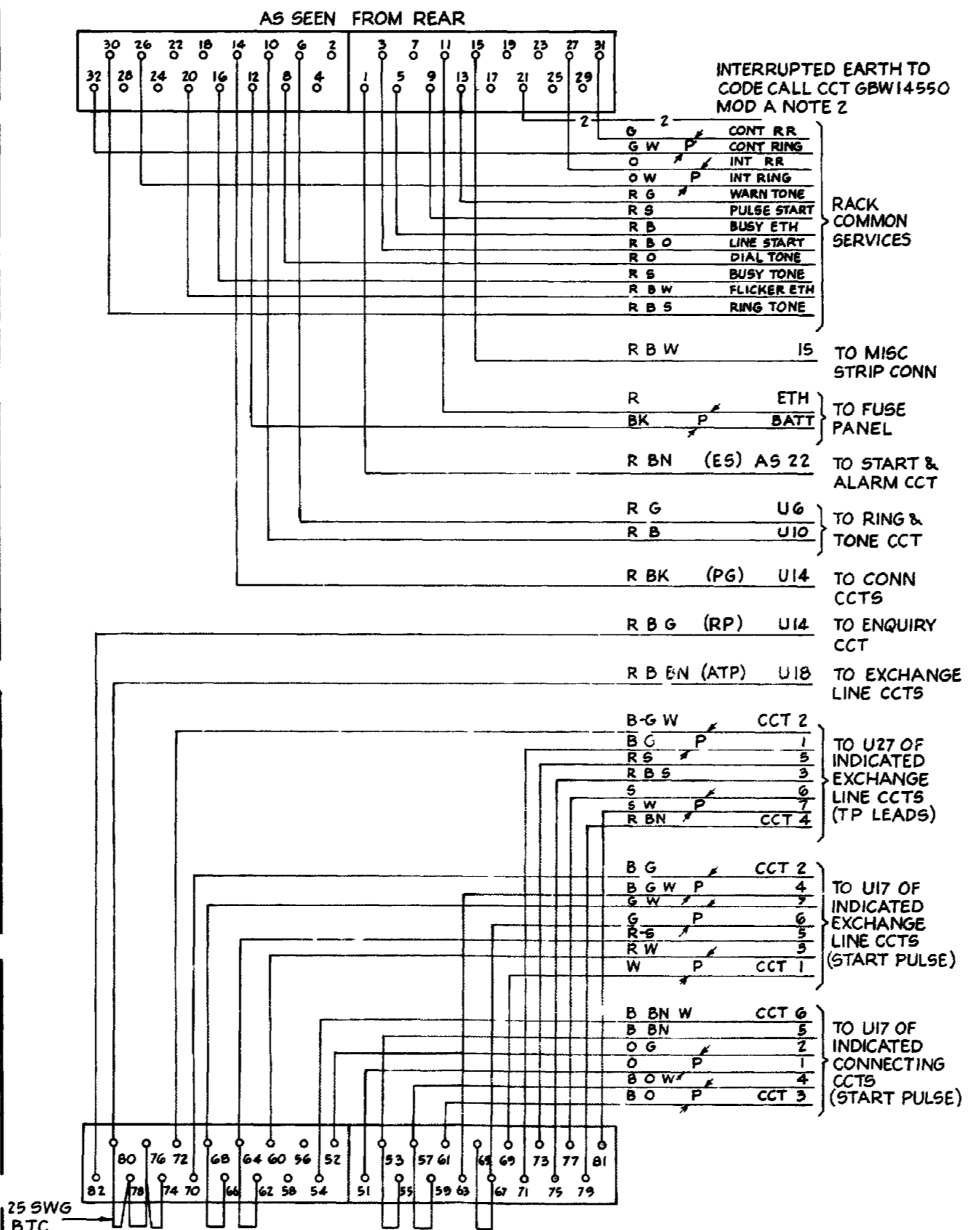
FIG 1B 35 LINE PABX
