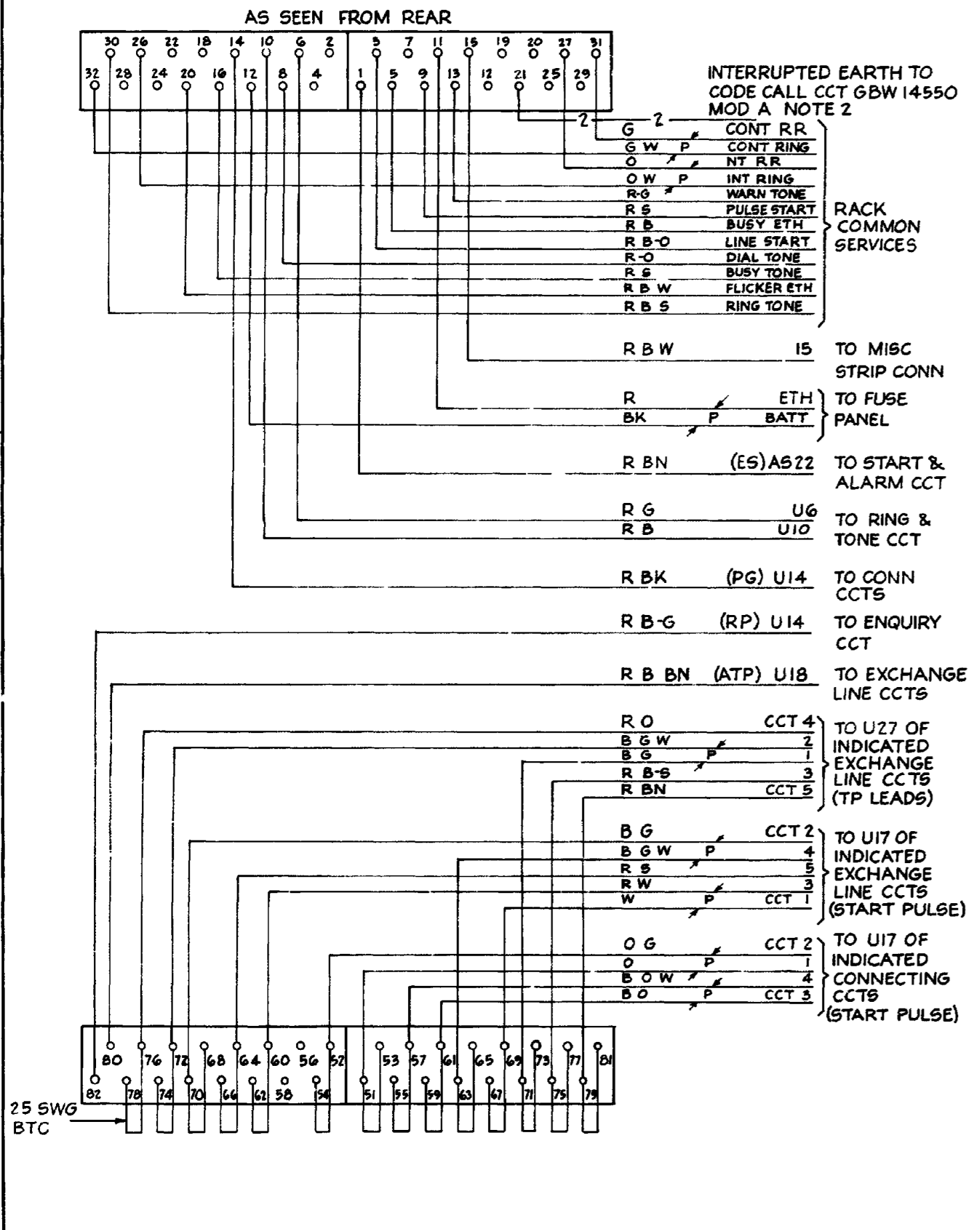
FIG 1A 20 LINE PABX
