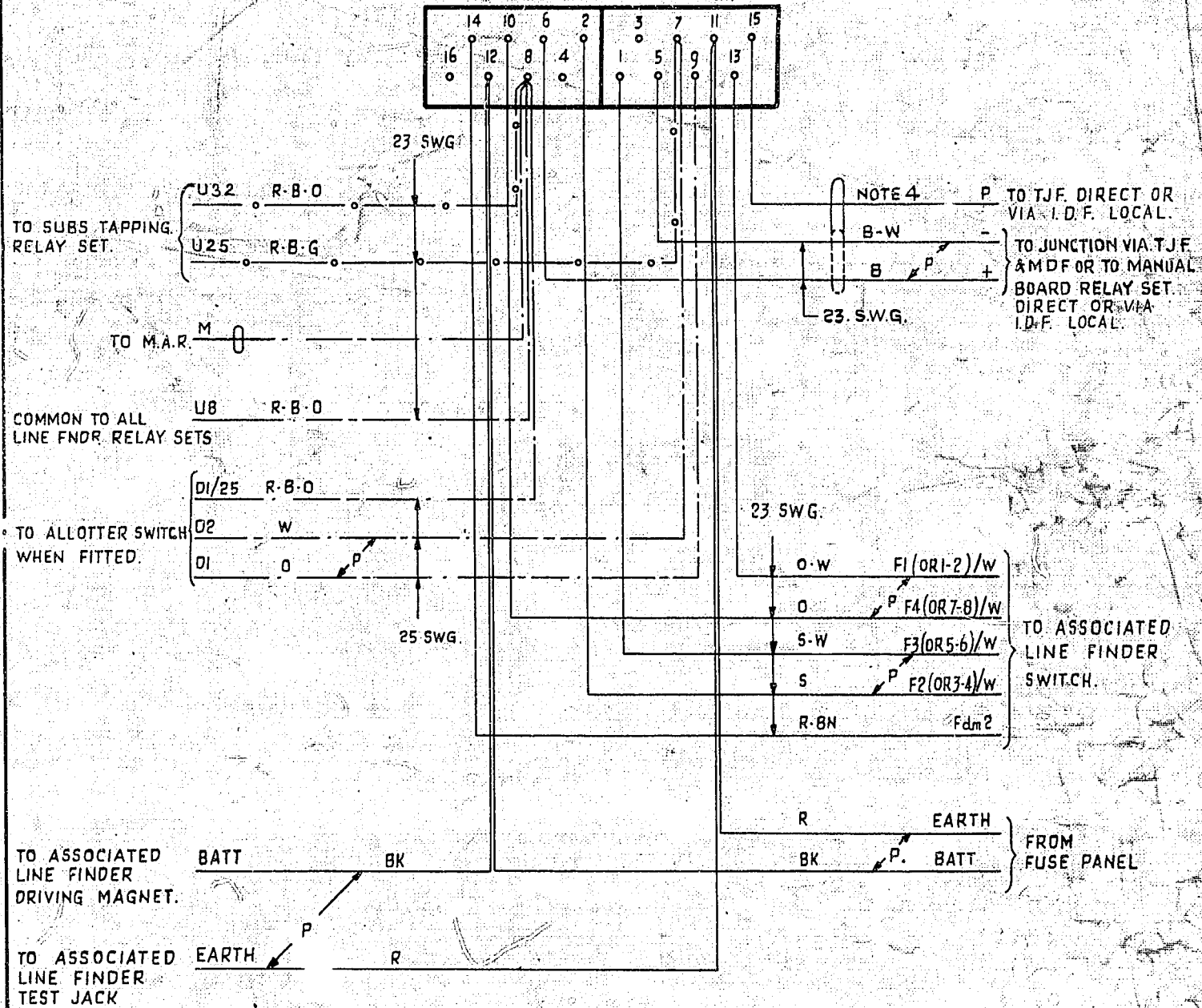
FIG. 2. LINE FINDER RELAY SET.
