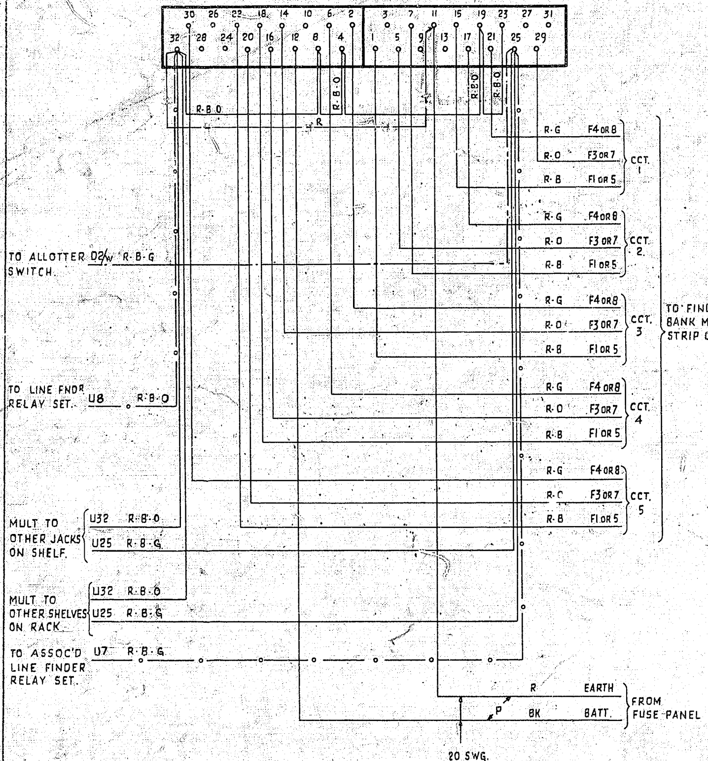
FIG. 1. SUBS TAPPING RELAY SET.
