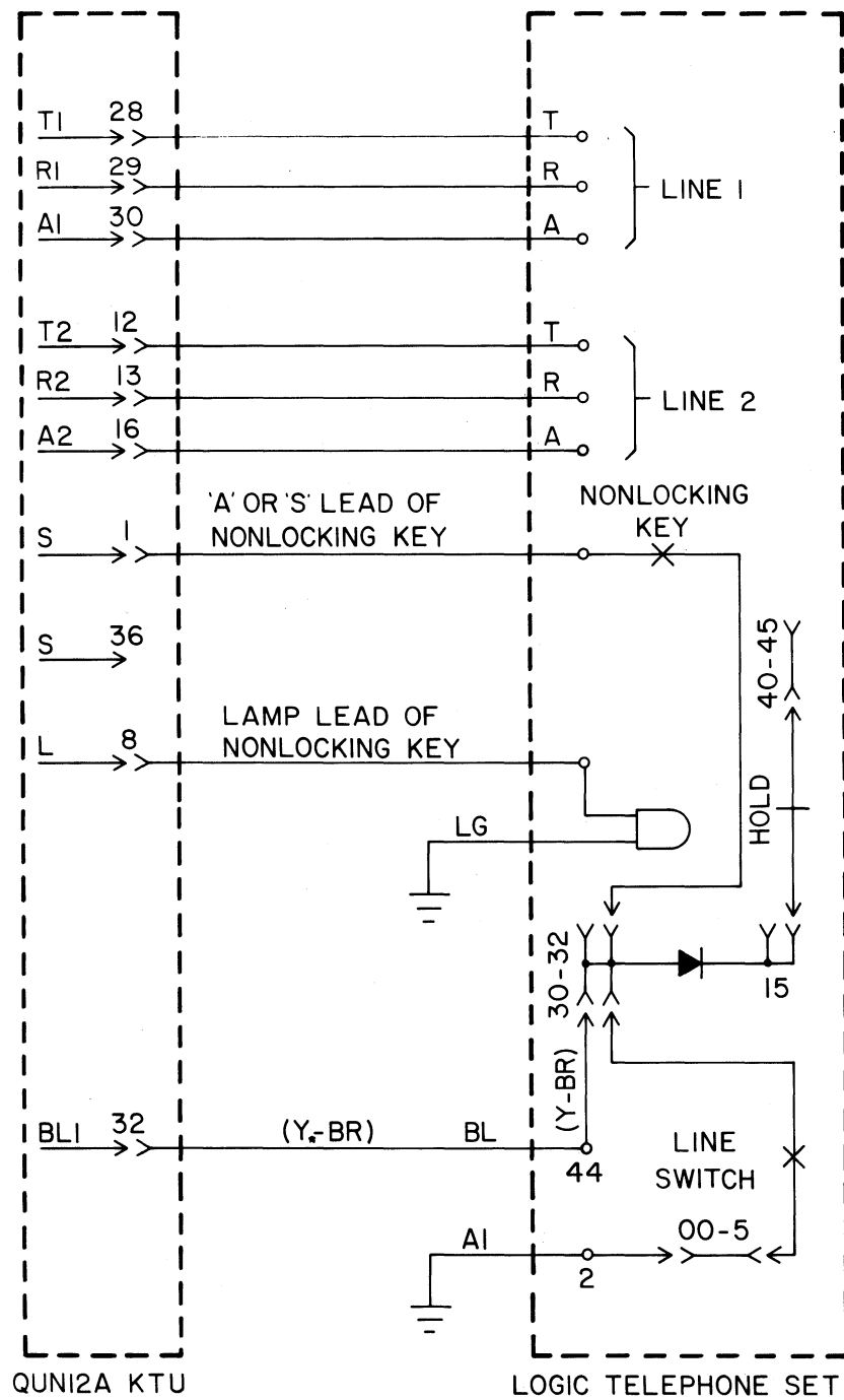
Fig. 12(a) — Add-on Circuit for QUN12A KTU
