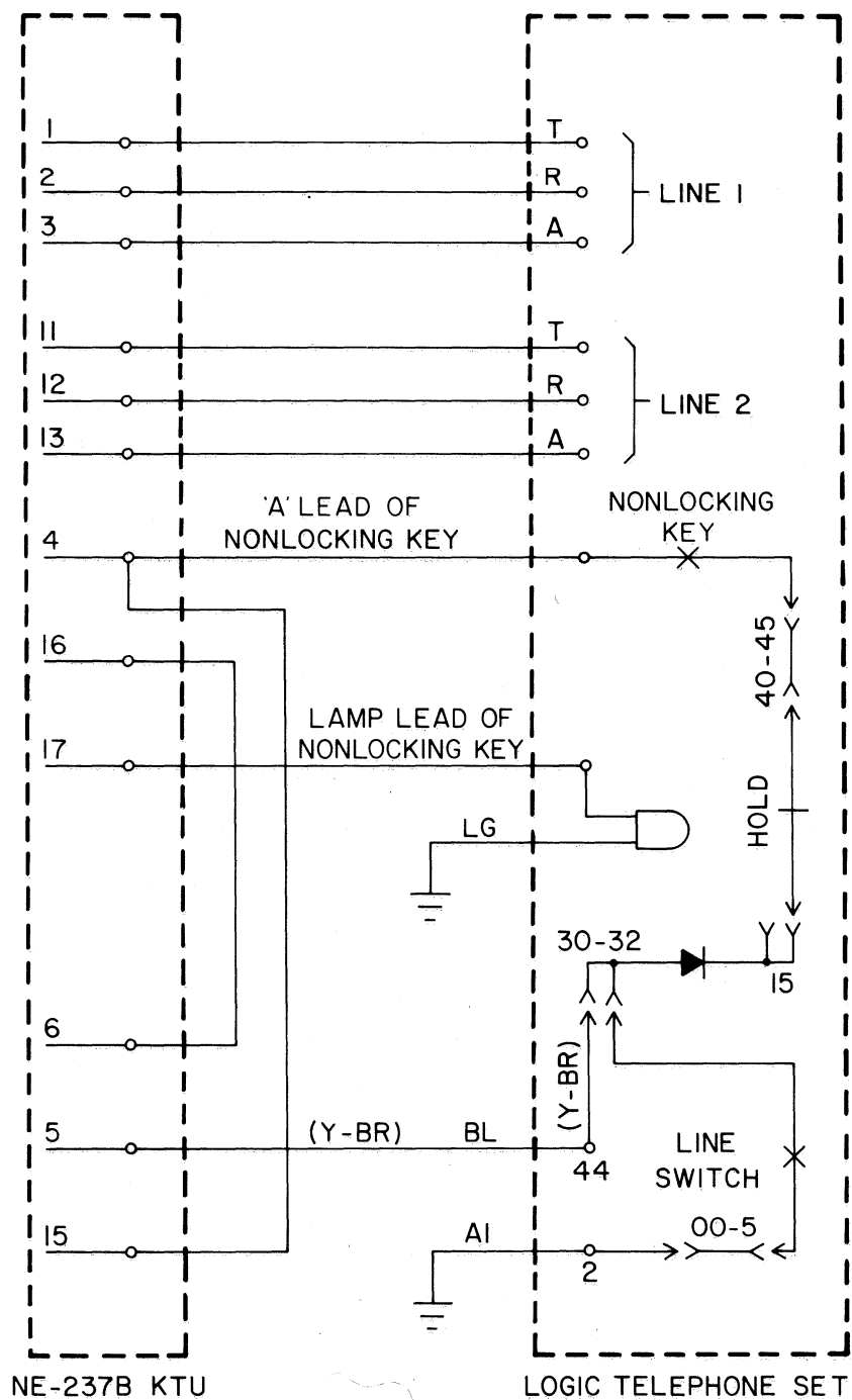
Fig. 12(b) — Add-on Circuit for NE-237B KTU
