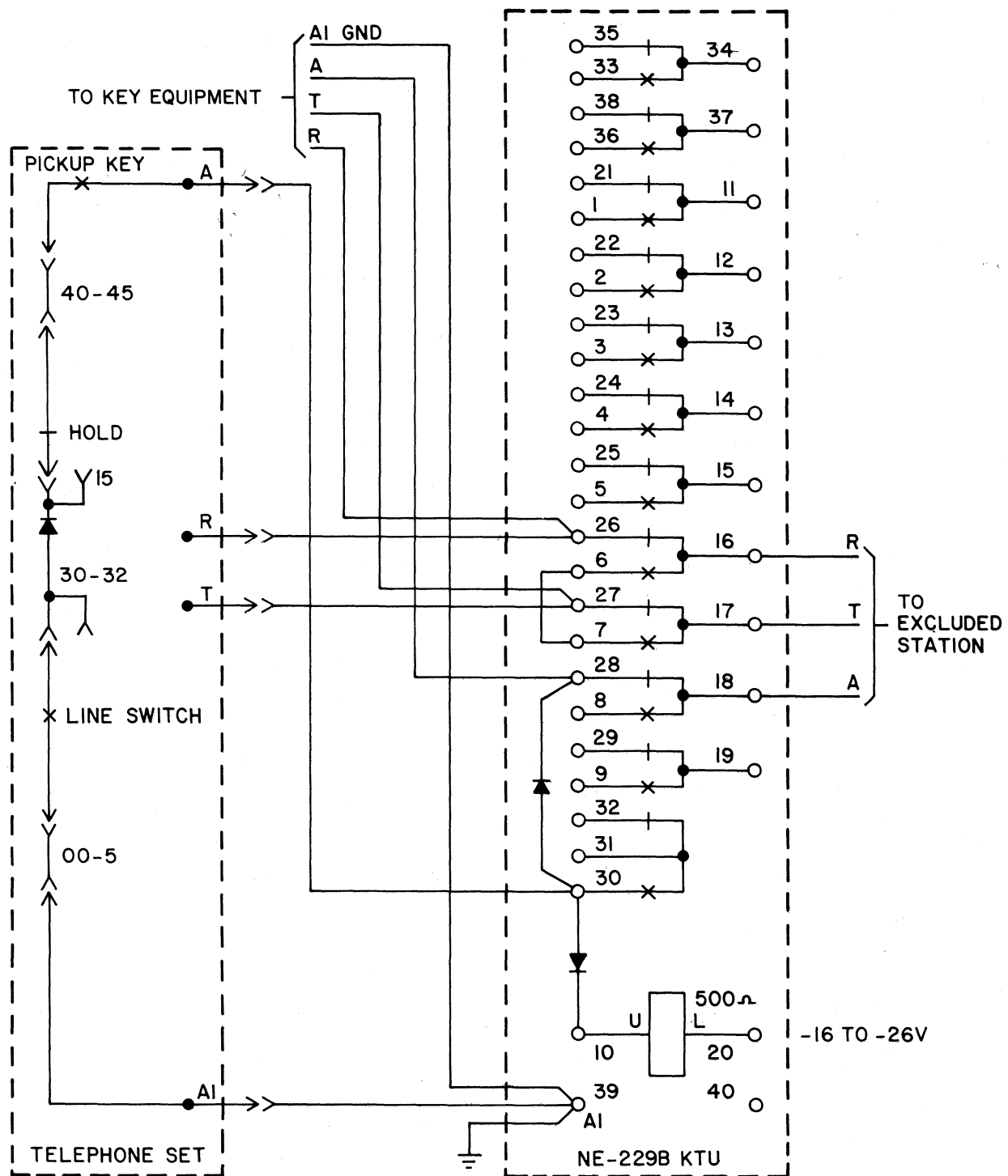
Fig. 10(b) – Automatic Exclusion for NE-229B KTU
