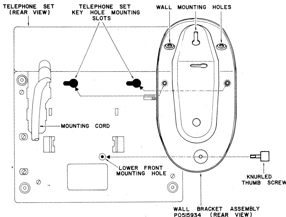
Fig. 2 — Method of Mounting LOGIC 10 Telephone Set to Wall
