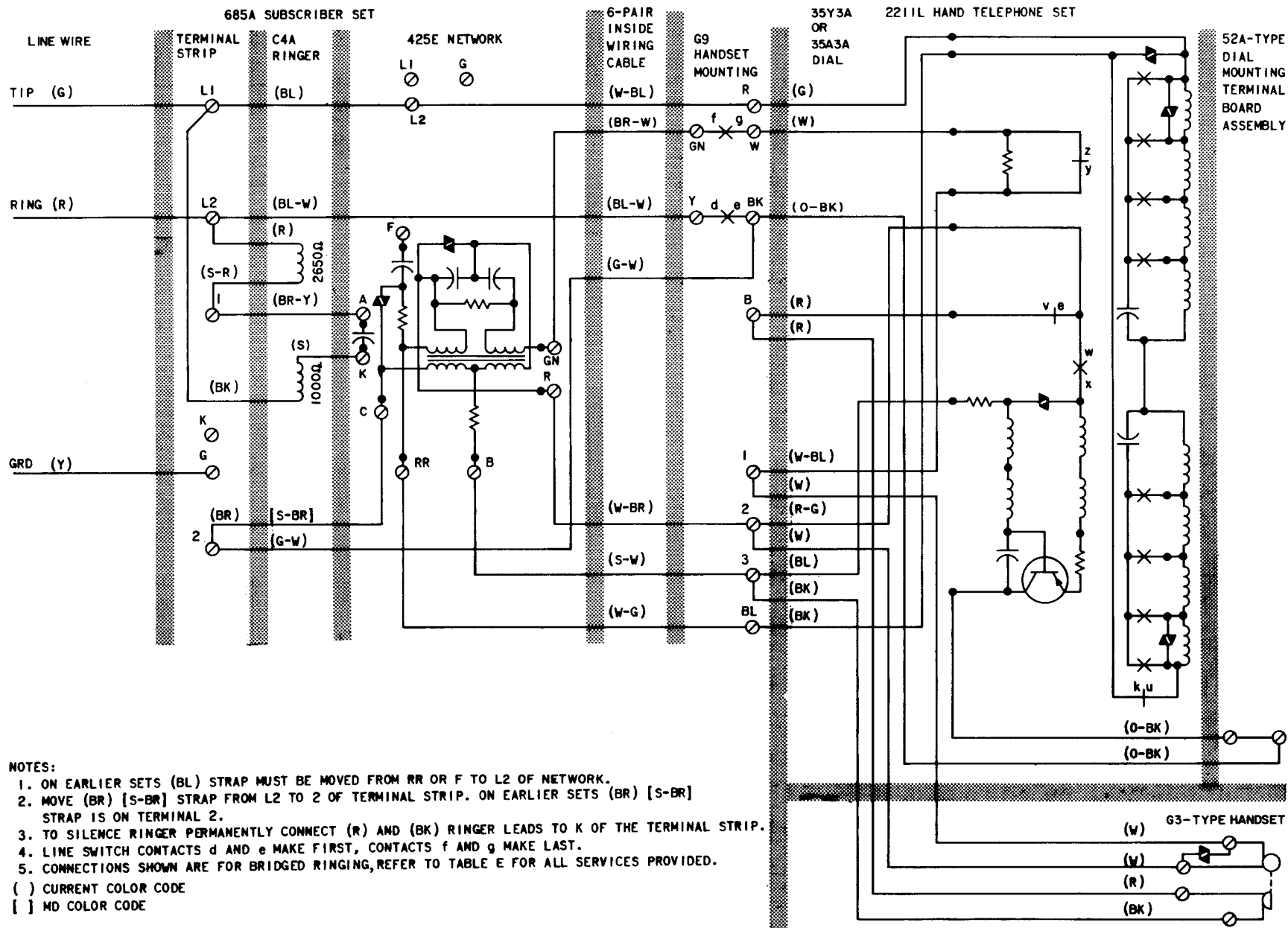
Connections for 2211L-3 Hand Telephone Set Used With Modified 685A Subscribed Set, Bridged Ringing
