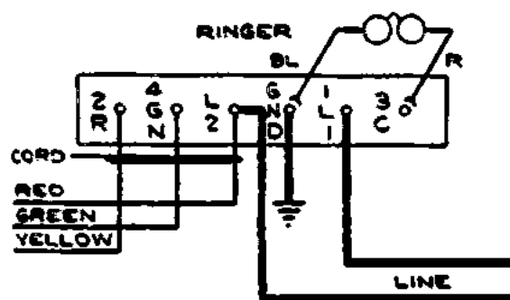
CONNECTIONS FOR FIRST PARTY ON TWO-PARTY LINES & SIMPLEX SYSTEMS
