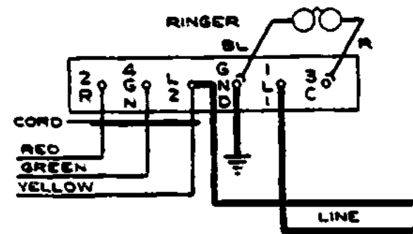
CONNECTIONS FOR SECOND PARTY ON TWO-PARTY LINES
