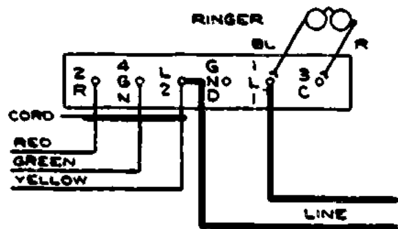
CONNECTIONS FOR REGULAR STATION
