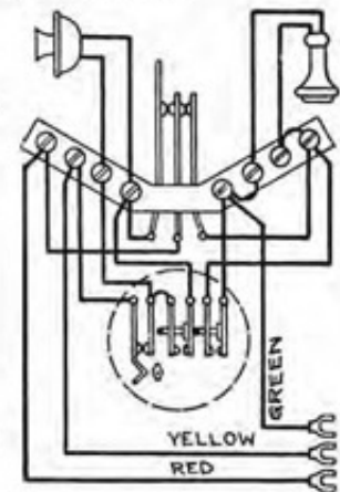
Wiring Diagrams Showing No. 1176 Desk Stand Wired to Various Types of Dials
