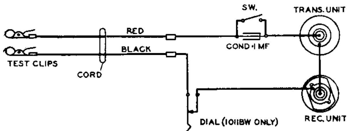
No. 1011AW and No. 1011BW Hand Set
