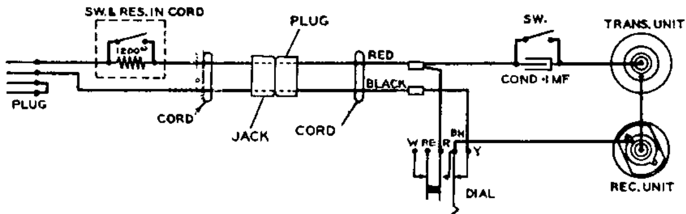
No. 1011G Hand Set Equipped with No. 2W39A Cord
