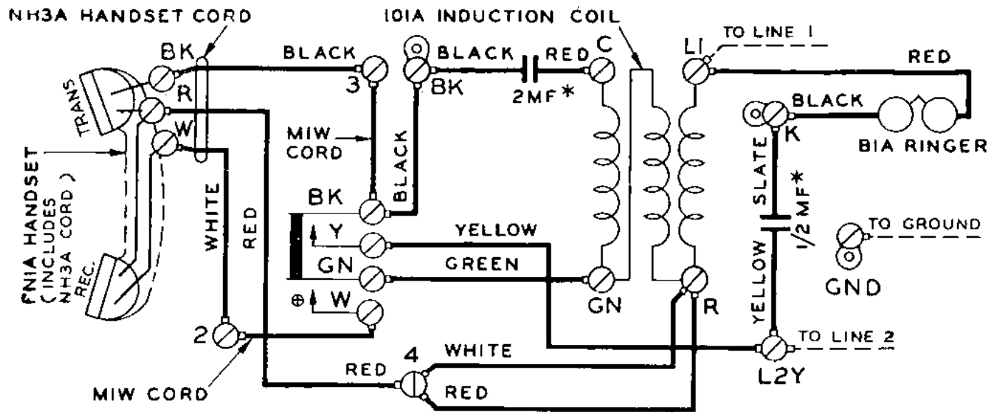
Wiring Diagram for No. 2 Type Uniphone for Manual Service
