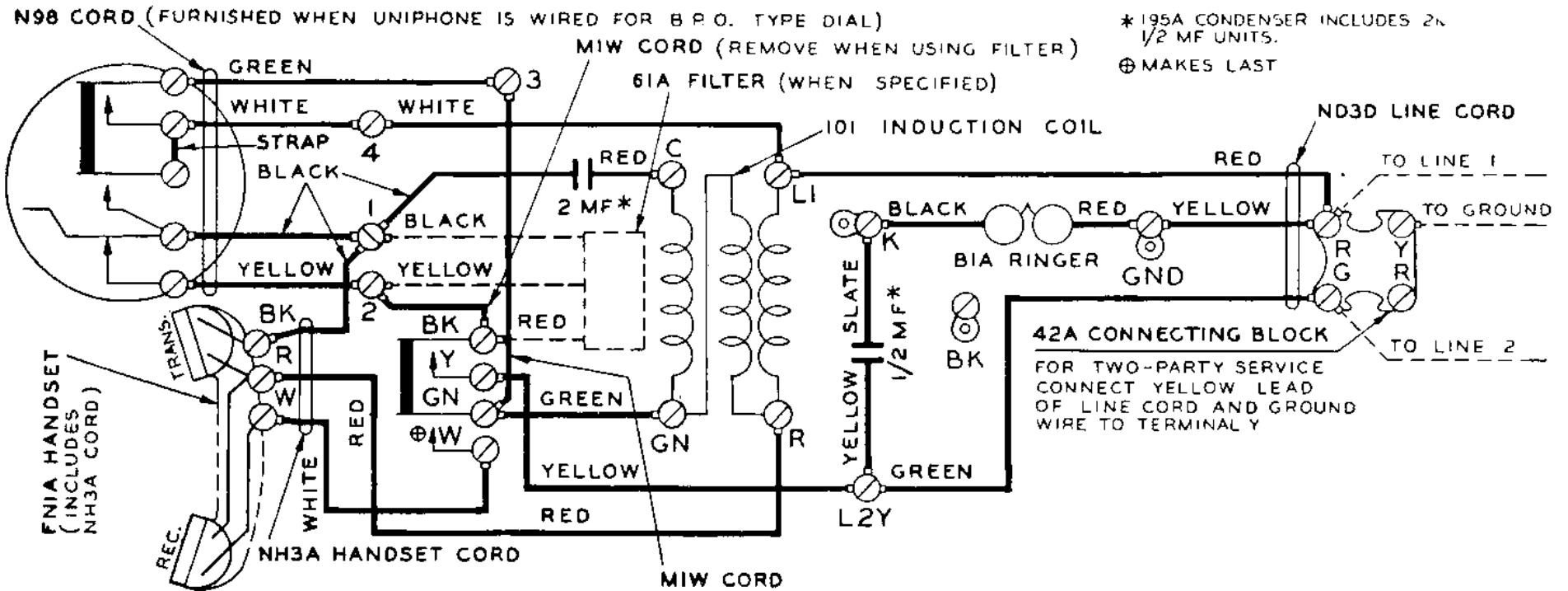
Wiring Diagram for No. 1 Type Uniphone Equipped with a British Post Office Type Dial
